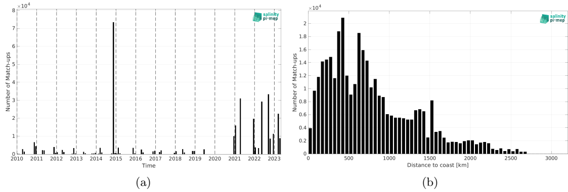
Figure 2: Number of match-ups between TSG (Polarstern) and SMOS SSS L3 v9 - 9 Days (CATDS-CEC-LOCEAN) SSS as a function of time (a) and as function of the distance to coast (b) over the Mid-Low Latitudes 45N-45S Pi-MEP region and for the full satellite product period.
