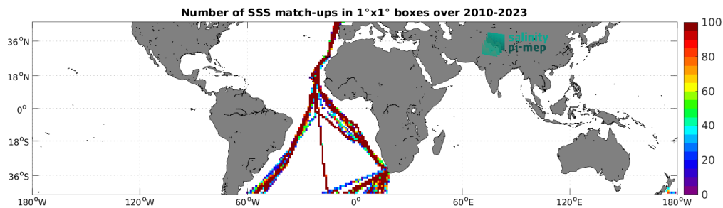
Figure 5: Number of SSS match-ups between TSG (Polarstern) SSS and the SMOS SSS L3 v9 - 9 Days (CATDS-CEC-LOCEAN) SSS product for the Mid-Low Latitudes 45N-45S Pi-MEP region over 1^\circ \times 1^\circ boxes and for the full satellite product period.
