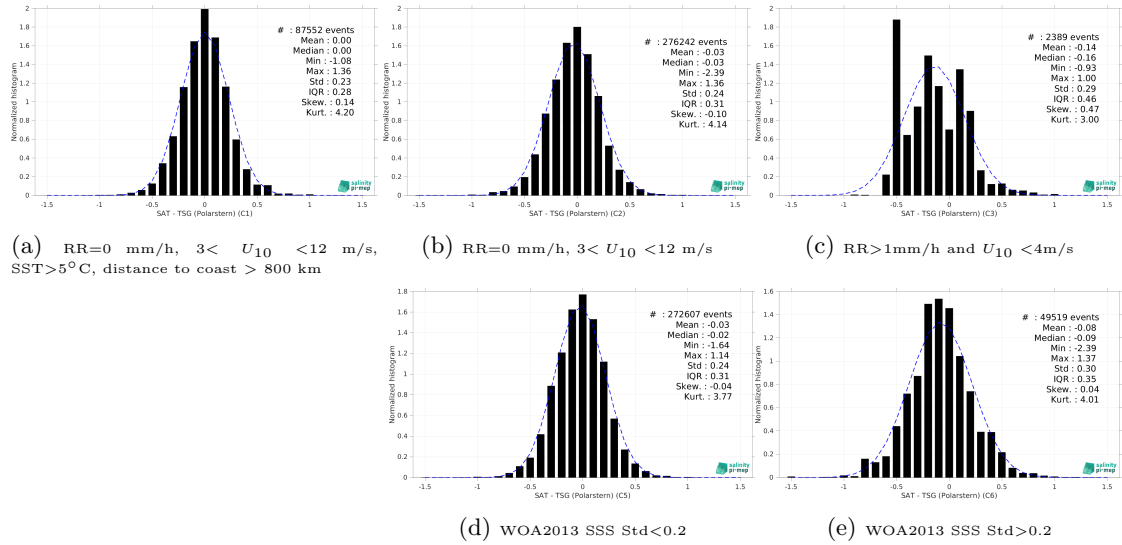
Figure 15: Normalized histogram of \Delta\text{SSS} (SMOS SSS L3 v9 - 9 Days (CATDS-CEC-LOCEAN) - TSG (Polarstern)) for 5 different subdatasets corresponding to: RR=0 mm/h, 3 < U_{10} < 12 m/s, SST > 5^\circ\text{C} , distance to coast > 800 km (a), RR=0 mm/h, 3 < U_{10} < 12 m/s (b), RR > 1 mm/h and U_{10} < 4 m/s (c), WOA2013 SSS Std < 0.2 (d), WOA2013 SSS Std > 0.2 (e).
