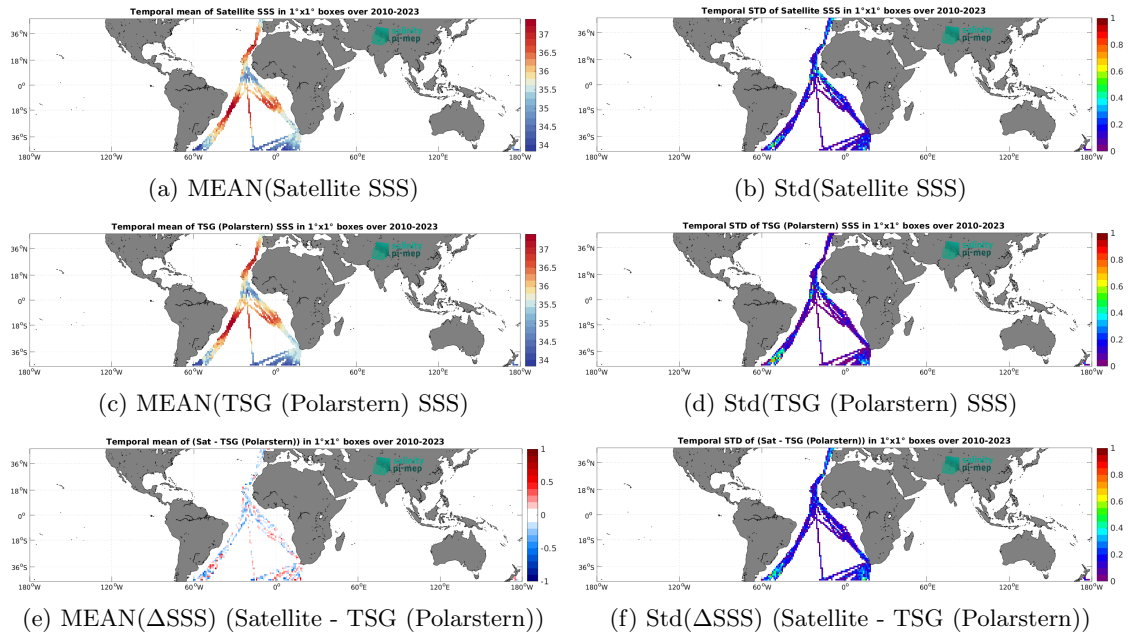
Figure 7: Temporal mean (left) and Std (right) of SSS from SMOS SSS L3 v9 - 9 Days (CATDS-CEC-LOCEAN) (top), TSG (Polarstern) (middle), and of \Delta SSS (Satellite - TSG (Polarstern)). Only match-up pairs are used to generate these maps.
