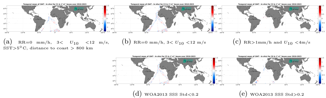
Figure 14: Temporal mean gridded over spatial boxes of size 1^\circ \times 1^\circ of \Delta\text{SSS} (SMOS SSS L3 v9 - 9 Days (CATDS-CEC-LOCEAN) - TSG (Polarstern)) for 5 different subdatasets corresponding to: RR=0 mm/h, 3 < U_{10} < 12 m/s, SST > 5°C, distance to coast > 800 km (a), RR=0 mm/h, 3 < U_{10} < 12 m/s (b), RR > 1mm/h and U_{10} < 4 m/s (c), WOA2013 SSS Std < 0.2 (d), WOA2013 SSS Std > 0.2 (e).
