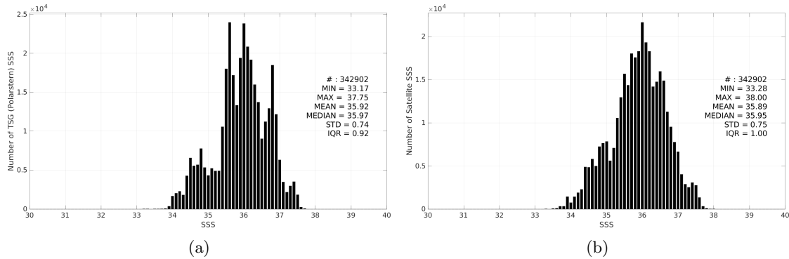
Figure 3: Histograms of SSS from TSG (Polarstern) (a) and SMOS SSS L3 v9 - 9 Days (CATDS-CEC-LOCEAN) (b) considering all match-up pairs per bins of 0.1 over the Mid-Low Latitudes 45N-45S Pi-MEP region and for the full satellite product period.
