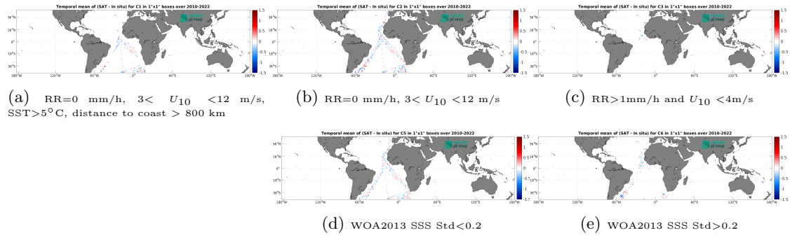
Figure 12: Temporal mean gridded over spatial boxes of size 1^\circ \times 1^\circ of \Delta SSS (SMOS SSS L3 v9 - 9 Days (CATDS-CEC-LOCEAN) - TSG (Polarstern)) for 5 different subdatasets corresponding to:RR=0 mm/h, 3 < U_{10} < 12 m/s, SST >5^\circ C, distance to coast > 800 km (a), RR=0 mm/h, 3 < U_{10} < 12 m/s (b), RR >1 mm/h and U_{10} < 4 m/s (c), WOA2013 SSS Std <0.2 (d), WOA2013 SSS Std >0.2 (e).
