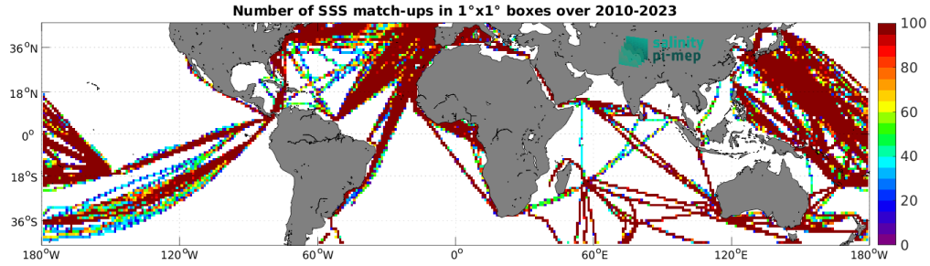
Figure 5: Number of SSS match-ups between TSG (LEGOS-DM) SSS and the SMOS SSS L3 v9 - 9 Days (CATDS-CEC-LOCEAN) SSS product for the Mid-Low Latitudes 45N-45S Pi-MEP region over 1^\circ \times 1^\circ boxes and for the full satellite product period.
