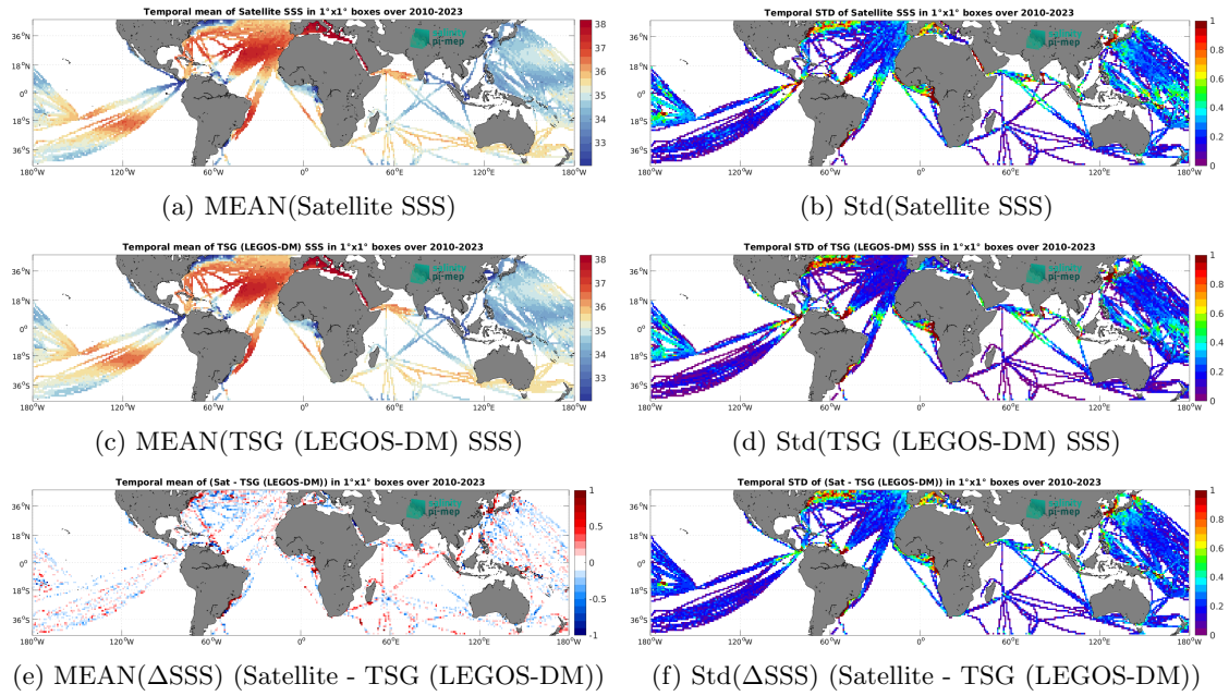
Figure 7: Temporal mean (left) and Std (right) of SSS from SMOS SSS L3 v9 - 9 Days (CATDS-CEC-LOCEAN) (top), TSG (LEGOS-DM) (middle), and of \Delta SSS (Satellite - TSG (LEGOS-DM)). Only match-up pairs are used to generate these maps.
