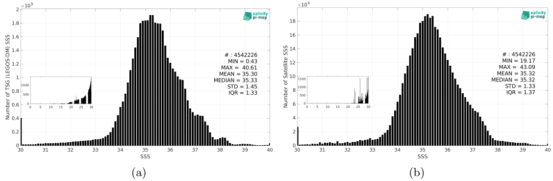
Figure 3: Histograms of SSS from TSG (LEGOS-DM) (a) and SMOS SSS L3 v9 - 9 Days (CATDS-CEC-LOCEAN) (b) considering all match-up pairs per bins of 0.1 over the Mid-Low Latitudes 45N-45S Pi-MEP region and for the full satellite product period.
