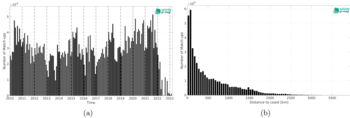
Figure 2: Number of match-ups between TSG (LEGOS-DM) and SMOS SSS L3 v9 - 9 Days (CATDS-CEC-LOCEAN) SSS as a function of time (a) and as function of the distance to coast (b) over the Mid-Low Latitudes 45N-45S Pi-MEP region and for the full satellite product period.
