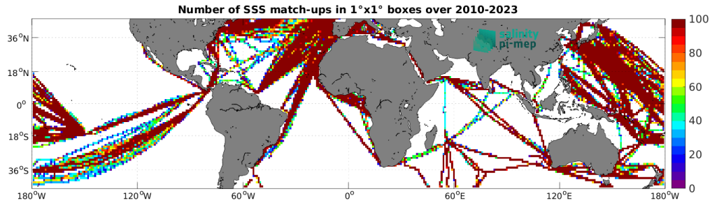
Figure 4: Number of SSS match-ups between TSG (LEGOS-DM) SSS and the SMOS SSS L3 v9 - 9 Days (CATDS-CEC-LOCEAN) SSS product for the Mid-Low Latitudes 45N-45S Pi-MEP region over 1^\circ \times 1^\circ boxes and for the full satellite product period.
