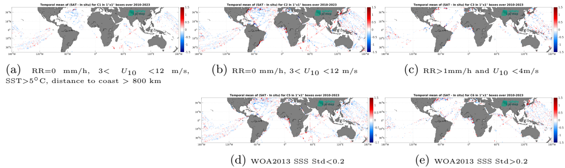
Figure 12: Temporal mean gridded over spatial boxes of size 1^\circ \times 1^\circ of \Delta\text{SSS} (SMOS SSS L3 v9 - 9 Days (CATDS-CEC-LOCEAN) - TSG (LEGOS-DM)) for 5 different subdatasets corresponding to:RR=0 mm/h, 3 < U_{10} < 12 m/s, SST >5^\circ\text{C} , distance to coast > 800 km (a), RR=0 mm/h, 3 < U_{10} < 12 m/s (b), RR >1 mm/h and U_{10} < 4 m/s (c), WOA2013 SSS Std <0.2 (d), WOA2013 SSS Std >0.2 (e).
