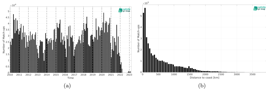
Figure 1: Number of match-ups between TSG (LEGOS-DM) and SMOS SSS L3 v9 - 9 Days (CATDS-CEC-LOCEAN) SSS as a function of time (a) and as function of the distance to coast (b) over the Mid-Low Latitudes 45N-45S Pi-MEP region and for the full satellite product period.
