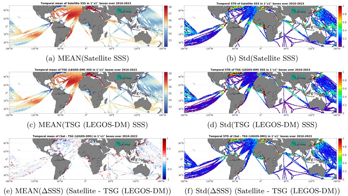
Figure 6: Temporal mean (left) and Std (right) of SSS from SMOS SSS L3 v9 - 9 Days (CATDS-CEC-LOCEAN) (top), TSG (LEGOS-DM) (middle), and of \Delta SSS (Satellite - TSG (LEGOS-DM)). Only match-up pairs are used to generate these maps.
