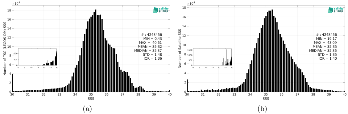
Figure 2: Histograms of SSS from TSG (LEGOS-DM) (a) and SMOS SSS L3 v9 - 9 Days (CATDS-CEC-LOCEAN) (b) considering all match-up pairs per bins of 0.1 over the Mid-Low Latitudes 45N-45S Pi-MEP region and for the full satellite product period.
