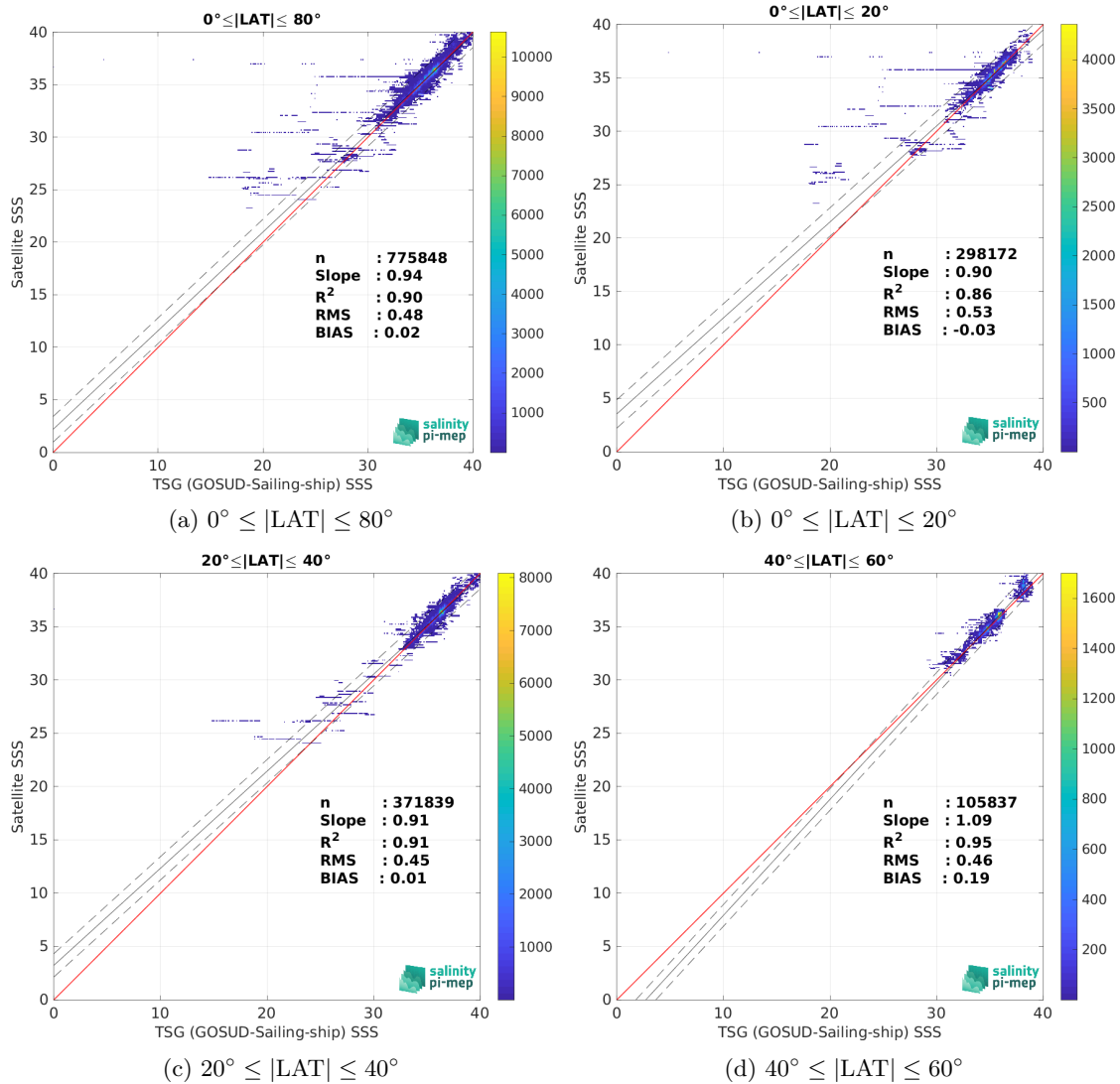
Figure 10: Contour maps of the concentration of SMOS SSS L3 v9 - 9 Days (CATDS-CEC-LOCEAN) SSS (y-axis) versus TSG (GOSUD-Sailing-ship) SSS (x-axis) at match-up pairs for different latitude bands. For each plot, the red line shows x=y . The black thin and dashed lines indicate a linear fit through the data cloud and the \pm 95\% confidence levels, respectively. The number match-up pairs n , the slope and R^2 coefficient of the linear fit, the root mean square (RMS) and the mean bias between satellite and in situ data are indicated for each latitude band in each plots.
