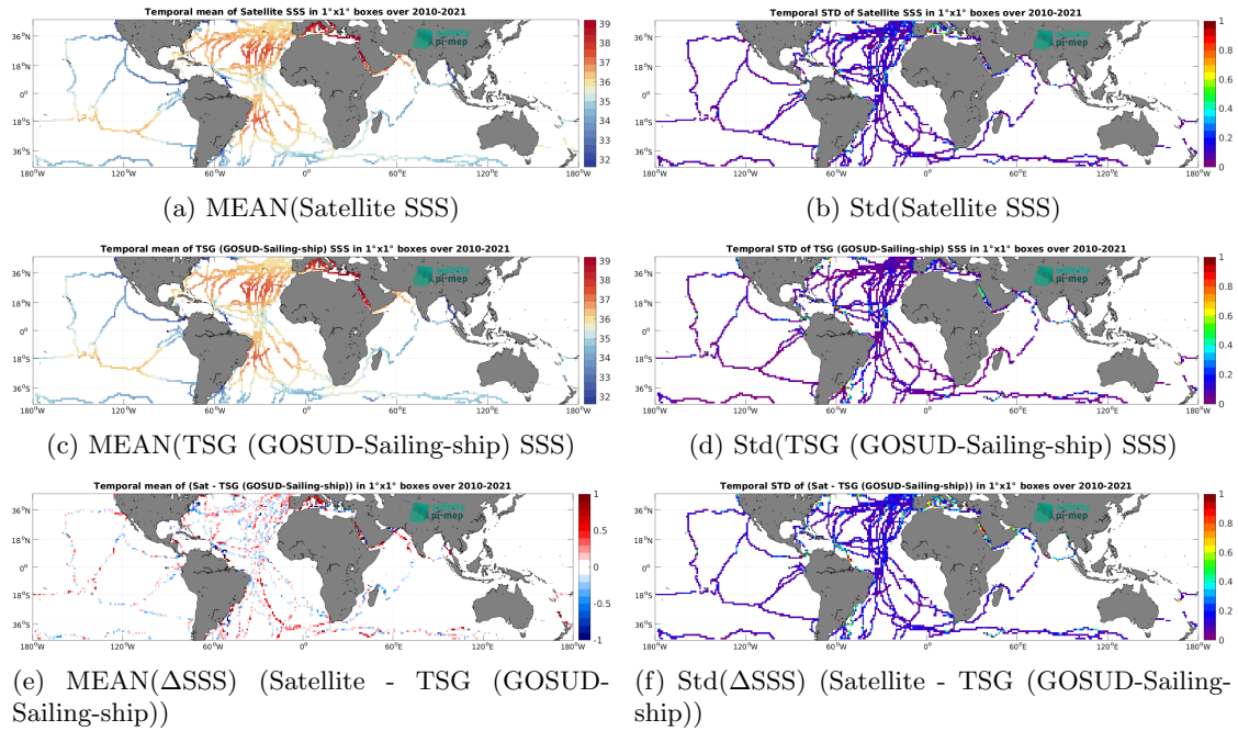
Figure 7: Temporal mean (left) and Std (right) of SSS from SMOS SSS L3 v9 - 9 Days (CATDS-CEC-LOCEAN) (top), TSG (GOSUD-Sailing-ship) (middle), and of \Delta SSS (Satellite - TSG (GOSUD-Sailing-ship)). Only match-up pairs are used to generate these maps.
