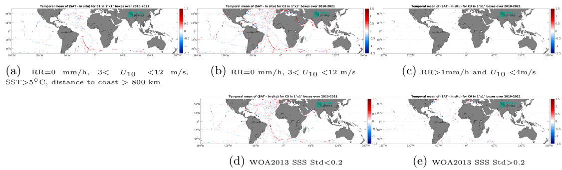
Figure 14: Temporal mean gridded over spatial boxes of size 1^\circ \times 1^\circ of \Delta\text{SSS} (SMOS SSS L3 v9 - 9 Days (CATDS-CEC-LOCEAN) - TSG (GOSUD-Sailing-ship)) for 5 different subdatasets corresponding to:RR=0 mm/h, 3 < U_{10} < 12 m/s, SST>5°C, distance to coast > 800 km (a), RR=0 mm/h, 3 < U_{10} < 12 m/s (b), RR>1mm/h and U_{10} < 4 m/s (c), WOA2013 SSS Std<0.2 (d), WOA2013 SSS Std>0.2 (e).
