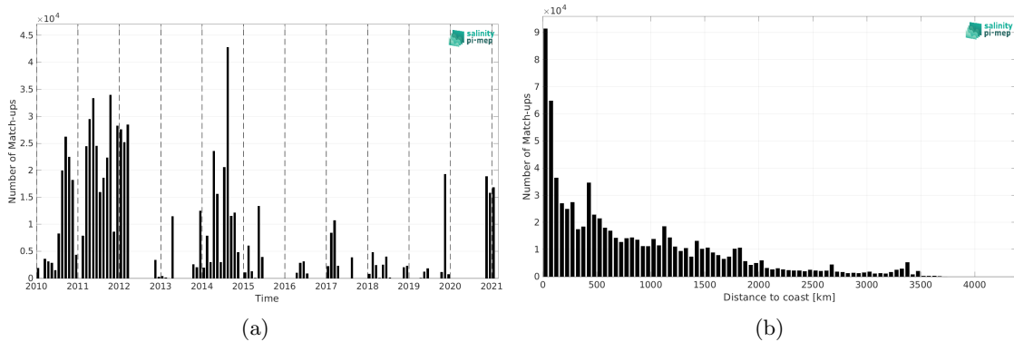
Figure 2: Number of match-ups between TSG (GOSUD-Sailing-ship) and SMOS SSS L3 v9 - 9 Days (CATDS-CEC-LOCEAN) SSS as a function of time (a) and as function of the distance to coast (b) over the Mid-Low Latitudes 45N-45S Pi-MEP region and for the full satellite product period.
