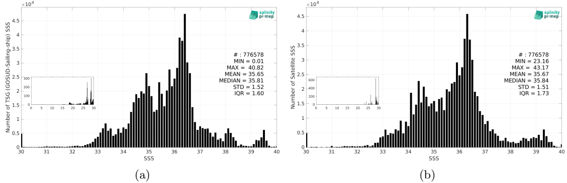
Figure 3: Histograms of SSS from TSG (GOSUD-Sailing-ship) (a) and SMOS SSS L3 v9 - 9 Days (CATDS-CEC-LOCEAN) (b) considering all match-up pairs per bins of 0.1 over the Mid-Low Latitudes 45N-45S Pi-MEP region and for the full satellite product period.
