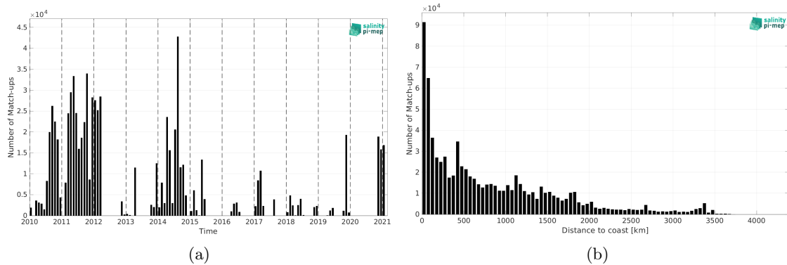
Figure 1: Number of match-ups between TSG (GOSUD-Sailing-ship) and SMOS SSS L3 v9 - 9 Days (CATDS-CEC-LOCEAN) SSS as a function of time (a) and as function of the distance to coast (b) over the Mid-Low Latitudes 45N-45S Pi-MEP region and for the full satellite product period.
