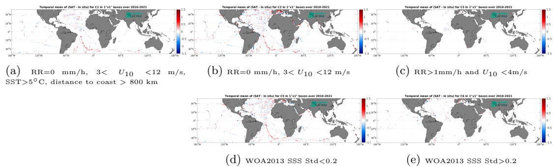
Figure 12: Temporal mean gridded over spatial boxes of size 1^\circ \times 1^\circ of \Delta SSS (SMOS SSS L3 v9 - 9 Days (CATDS-CEC-LOCEAN) - TSG (GOSUD-Sailing-ship)) for 5 different subdatasets corresponding to:RR=0 mm/h, 3 < U_{10} < 12 m/s, SST >5^\circ\text{C} , distance to coast > 800 km (a), RR=0 mm/h, 3 < U_{10} < 12 m/s (b), RR >1 mm/h and U_{10} < 4 m/s (c), WOA2013 SSS Std <0.2 (d), WOA2013 SSS Std >0.2 (e).
