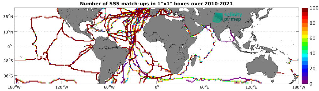
Figure 4: Number of SSS match-ups between TSG (GOSUD-Sailing-ship) SSS and the SMOS SSS L3 v9 - 9 Days (CATDS-CEC-LOCEAN) SSS product for the Mid-Low Latitudes 45N-45S Pi-MEP region over 1^\circ \times 1^\circ boxes and for the full satellite product period.
