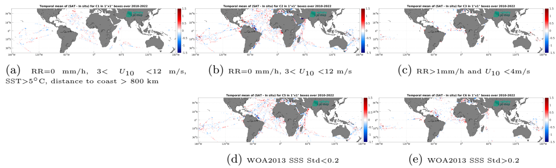
Figure 14: Temporal mean gridded over spatial boxes of size 1^\circ \times 1^\circ of \Delta SSS (SMOS SSS L3 v9 - 9 Days (CATDS-CEC-LOCEAN) - TSG (GOSUD-Research-vessel)) for 5 different subdatasets corresponding to: RR=0 mm/h, 3 < U_{10} < 12 m/s, SST > 5^\circ\text{C} , distance to coast > 800 km (a), RR=0 mm/h, 3 < U_{10} < 12 m/s (b), RR > 1 mm/h and U_{10} < 4 m/s (c), WOA2013 SSS Std < 0.2 (d), WOA2013 SSS Std > 0.2 (e).
