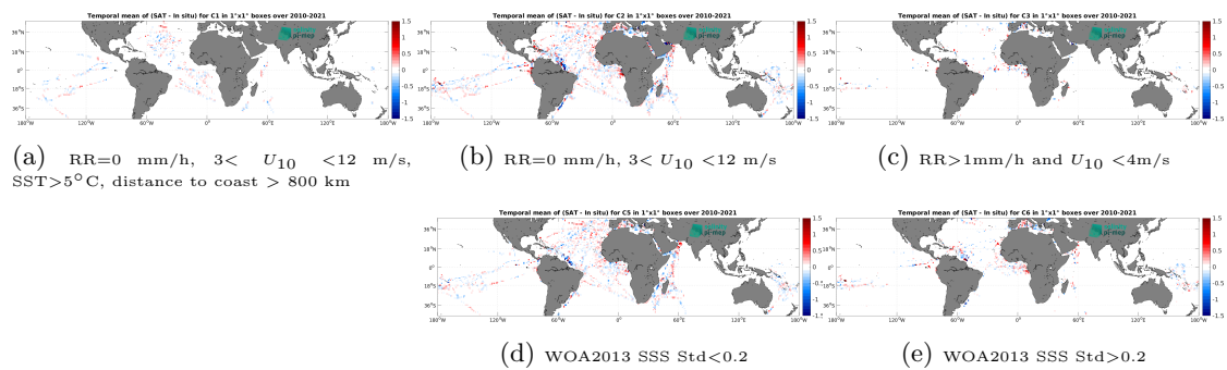
Figure 14: Temporal mean gridded over spatial boxes of size 1^\circ \times 1^\circ of \Delta\text{SSS} (SMOS SSS L3 v9 - 9 Days (CATDS-CEC-LOCEAN) - TSG (GOSUD-Research-vessel)) for 5 different subdatasets corresponding to: RR=0 mm/h, 3 < U_{10} < 12 m/s, SST > 5°C, distance to coast > 800 km (a), RR=0 mm/h, 3 < U_{10} < 12 m/s (b), RR > 1mm/h and U_{10} < 4 m/s (c), WOA2013 SSS Std < 0.2 (d), WOA2013 SSS Std > 0.2 (e).
