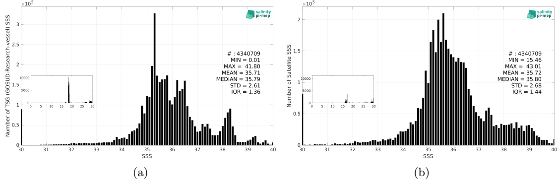
Figure 3: Histograms of SSS from TSG (GOSUD-Research-vessel) (a) and SMOS SSS L3 v9 - 9 Days (CATDS-CEC-LOCEAN) (b) considering all match-up pairs per bins of 0.1 over the Mid-Low Latitudes 45N-45S Pi-MEP region and for the full satellite product period.
