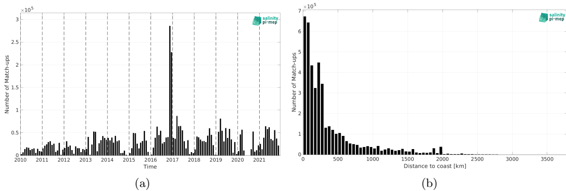
Figure 2: Number of match-ups between TSG (GOSUD-Research-vessel) and SMOS SSS L3 v9 - 9 Days (CATDS-CEC-LOCEAN) SSS as a function of time (a) and as function of the distance to coast (b) over the Mid-Low Latitudes 45N-45S Pi-MEP region and for the full satellite product period.
