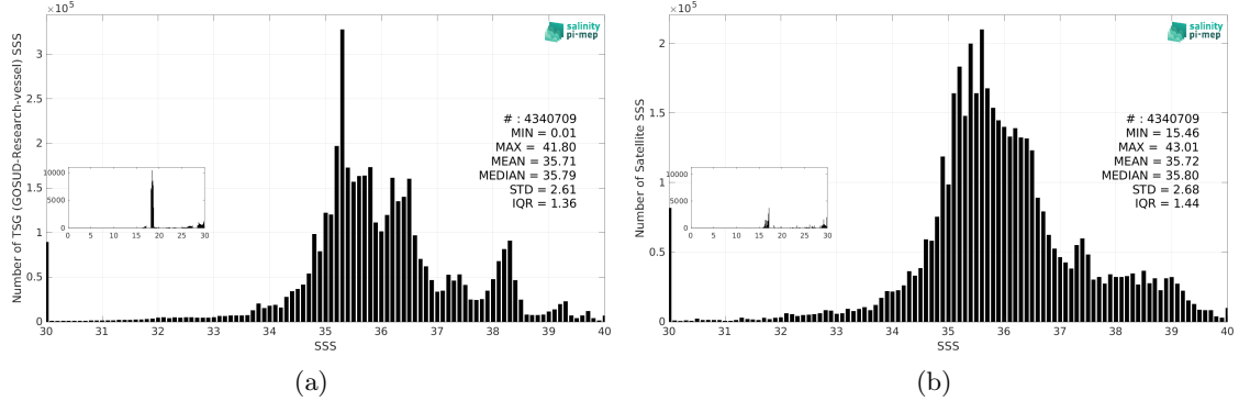
Figure 2: Histograms of SSS from TSG (GOSUD-Research-vessel) (a) and SMOS SSS L3 v9 - 9 Days (CATDS-CEC-LOCEAN) (b) considering all match-up pairs per bins of 0.1 over the Mid-Low Latitudes 45N-45S Pi-MEP region and for the full satellite product period.
