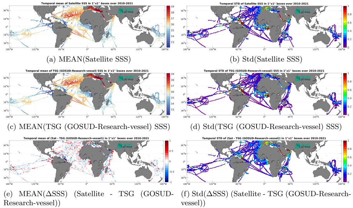
Figure 6: Temporal mean (left) and Std (right) of SSS from SMOS SSS L3 v9 - 9 Days (CATDS-CEC-LOCEAN) (top), TSG (GOSUD-Research-vessel) (middle), and of \Delta SSS (Satellite - TSG (GOSUD-Research-vessel)). Only match-up pairs are used to generate these maps.
