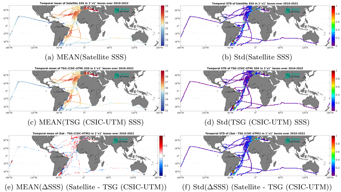
Figure 6: Temporal mean (left) and Std (right) of SSS from SMOS SSS L3 v9 - 9 Days (CATDS-CEC-LOCEAN) (top), TSG (CSIC-UTM) (middle), and of \Delta SSS (Satellite - TSG (CSIC-UTM)). Only match-up pairs are used to generate these maps.
