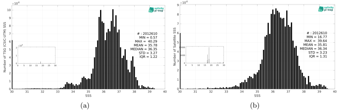
Figure 2: Histograms of SSS from TSG (CSIC-UTM) (a) and SMOS SSS L3 v9 - 9 Days (CATDS-CEC-LOCEAN) (b) considering all match-up pairs per bins of 0.1 over the Mid-Low Latitudes 45N-45S Pi-MEP region and for the full satellite product period.
