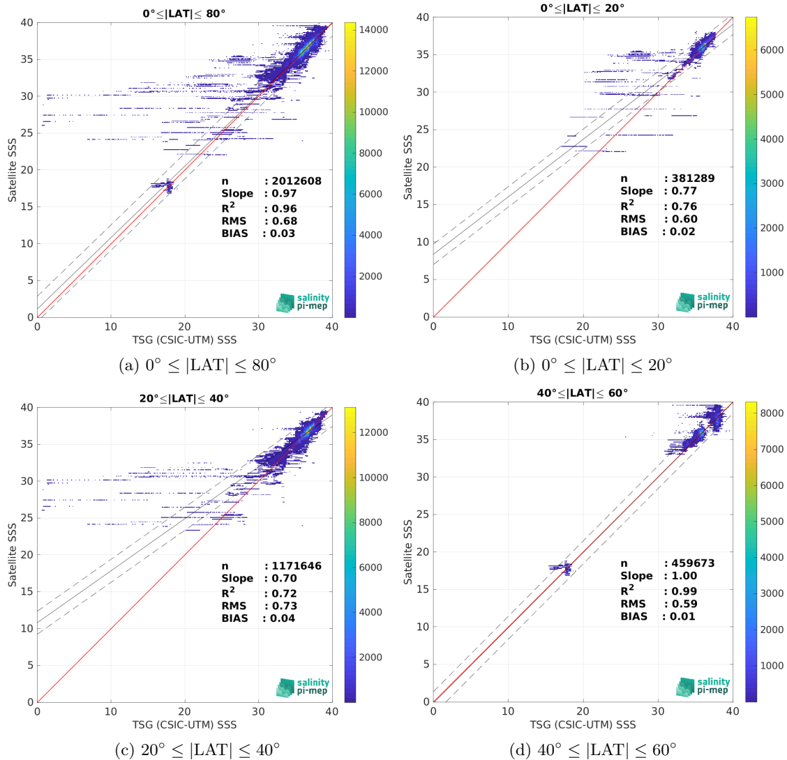
Figure 9: Contour maps of the concentration of SMOS SSS L3 v9 - 9 Days (CATDS-CEC-LOCEAN) SSS (y-axis) versus TSG (CSIC-UTM) SSS (x-axis) at match-up pairs for different latitude bands. For each plot, the red line shows x=y . The black thin and dashed lines indicate a linear fit through the data cloud and the \pm 95\% confidence levels, respectively. The number match-up pairs n , the slope and R^2 coefficient of the linear fit, the root mean square (RMS) and the mean bias between satellite and in situ data are indicated for each latitude band in each plots.
