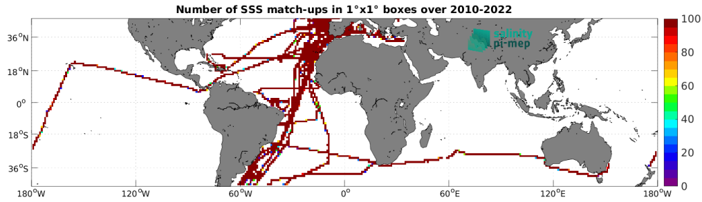
Figure 4: Number of SSS match-ups between TSG (CSIC-UTM) SSS and the SMOS SSS L3 v9 - 9 Days (CATDS-CEC-LOCEAN) SSS product for the Mid-Low Latitudes 45N-45S Pi-MEP region over 1^\circ \times 1^\circ boxes and for the full satellite product period.
