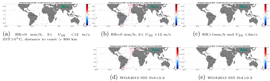
Figure 12: Temporal mean gridded over spatial boxes of size 1^\circ \times 1^\circ of \Delta SSS (SMOS SSS L3 v9 - 9 Days (CATDS-CEC-LOCEAN) - TSG (CSIC-UTM)) for 5 different subdatasets corresponding to:RR=0 mm/h, 3 < U_{10} < 12 m/s, SST >5^\circ C, distance to coast > 800 km (a), RR=0 mm/h, 3 < U_{10} < 12 m/s (b), RR >1 mm/h and U_{10} < 4 m/s (c), WOA2013 SSS Std <0.2 (d), WOA2013 SSS Std >0.2 (e).
