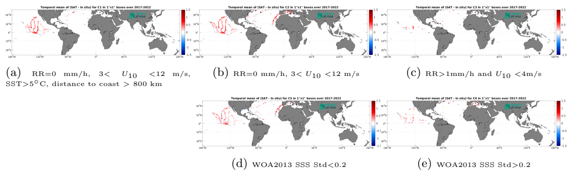
Figure 14: Temporal mean gridded over spatial boxes of size 1^\circ \times 1^\circ of \Delta\text{SSS} (SMOS SSS L3 v9 - 9 Days (CATDS-CEC-LOCEAN) - Saifdrone) for 5 different subdatasets corresponding to: RR=0 mm/h, 3 < U_{10} < 12 m/s, SST > 5°C, distance to coast > 800 km (a), RR=0 mm/h, 3 < U_{10} < 12 m/s (b), RR > 1mm/h and U_{10} < 4 m/s (c), WOA2013 SSS Std < 0.2 (d), WOA2013 SSS Std > 0.2 (e).
