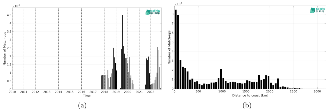
Figure 2: Number of match-ups between Saildrone and SMOS SSS L3 v9 - 9 Days (CATDS-CEC-LOCEAN) SSS as a function of time (a) and as function of the distance to coast (b) over the Mid-Low Latitudes 45N-45S Pi-MEP region and for the full satellite product period.
