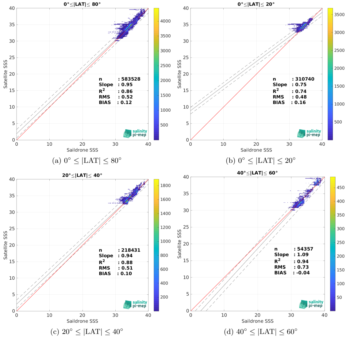
Figure 10: Contour maps of the concentration of SMOS SSS L3 v9 - 9 Days (CATDS-CEC-LOCEAN) SSS (y-axis) versus Sairdrone SSS (x-axis) at match-up pairs for different latitude bands. For each plot, the red line shows x=y . The black thin and dashed lines indicate a linear fit through the data cloud and the \pm 95\% confidence levels, respectively. The number match-up pairs n , the slope and R^2 coefficient of the linear fit, the root mean square (RMS) and the mean bias between satellite and in situ data are indicated for each latitude band in each plots.
