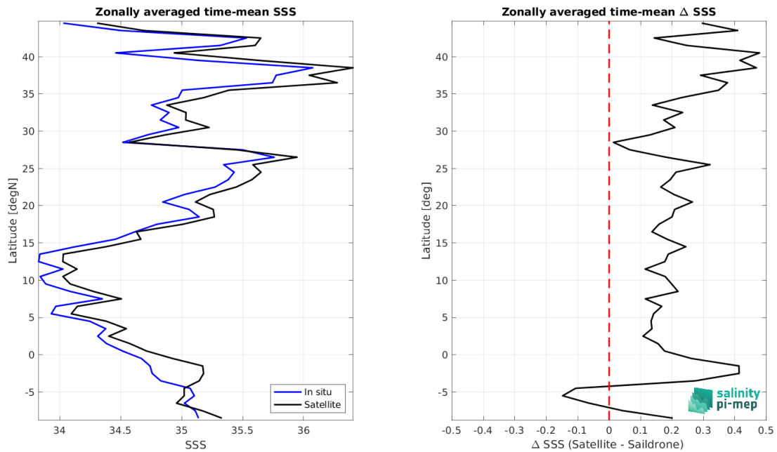
Figure 9: Left panel: Zonal mean SSS from SMOS SSS L3 v9 - 9 Days (CATDS-CEC-LOCEAN) satellite product (black) and from Sairdron (blue). Right panel: Zonal mean of \Delta SSS (Satellite - Sairdron) for all the collected Pi-MEP match-up pairs estimated over the full satellite product period.
