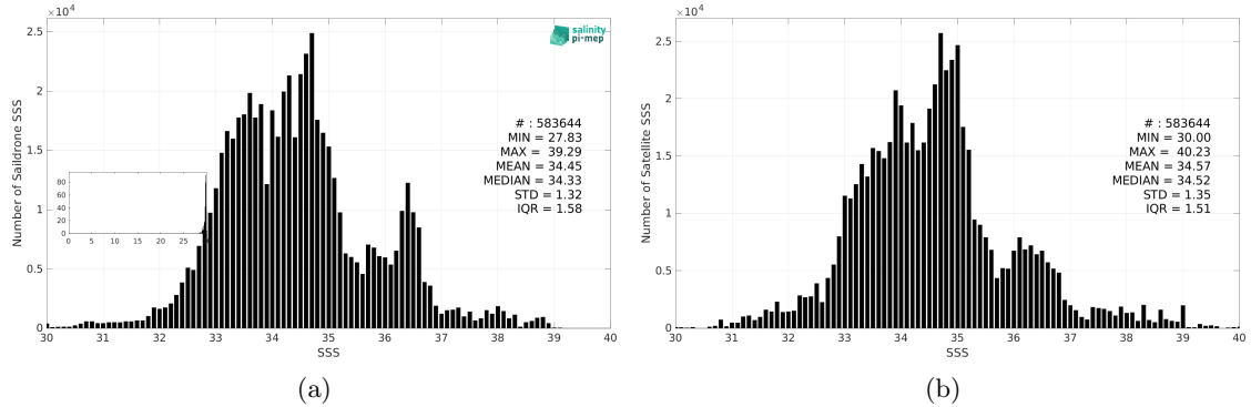
Figure 3: Histograms of SSS from Saildrone (a) and SMOS SSS L3 v9 - 9 Days (CATDS-CEC-LOCEAN) (b) considering all match-up pairs per bins of 0.1 over the Mid-Low Latitudes 45N-45S Pi-MEP region and for the full satellite product period.
