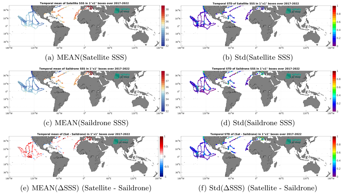
Figure 6: Temporal mean (left) and Std (right) of SSS from SMOS SSS L3 v9 - 9 Days (CATDS-CEC-LOCEAN) (top), Saildrone (middle), and of \Delta SSS (Satellite - Saildrone). Only match-up pairs are used to generate these maps.
