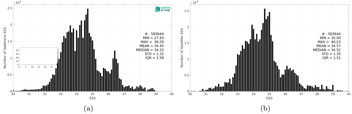
Figure 2: Histograms of SSS from Saildrone (a) and SMOS SSS L3 v9 - 9 Days (CATDS-CEC-LOCEAN) (b) considering all match-up pairs per bins of 0.1 over the Mid-Low Latitudes 45N-45S Pi-MEP region and for the full satellite product period.
