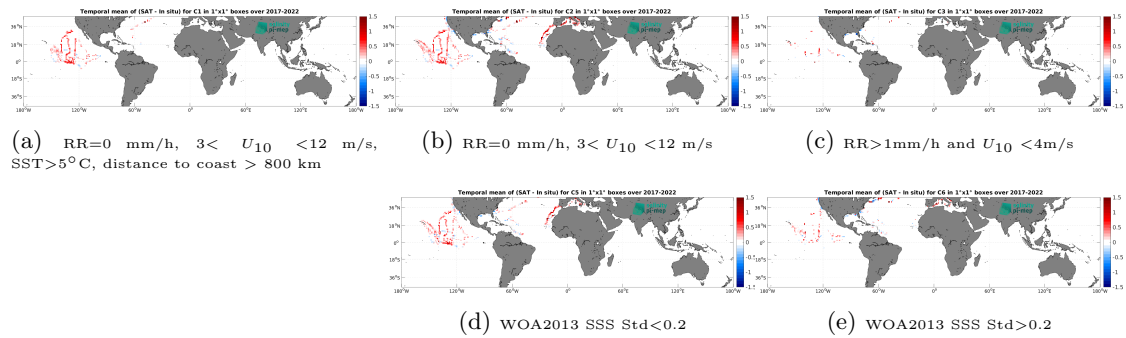
Figure 12: Temporal mean gridded over spatial boxes of size 1^\circ \times 1^\circ of \Delta SSS (SMOS SSS L3 v9 - 9 Days (CATDS-CEC-LOCEAN) - Saifdrone) for 5 different subdatasets corresponding to:RR=0 mm/h, 3 < U_{10} < 12 m/s, SST >5^\circ C, distance to coast > 800 km (a), RR=0 mm/h, 3 < U_{10} < 12 m/s (b), RR >1 mm/h and U_{10} < 4 m/s (c), WOA2013 SSS Std <0.2 (d), WOA2013 SSS Std >0.2 (e).
