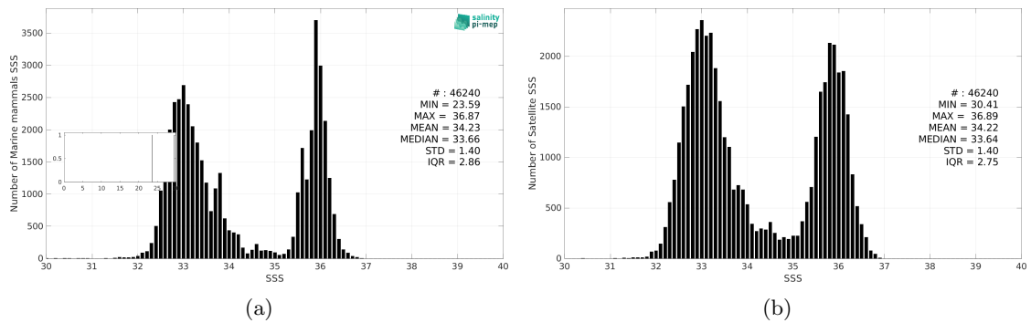
Figure 2: Histograms of SSS from Marine mammals (a) and SMOS SSS L3 v9 - 9 Days (CATDS-CEC-LOCEAN) (b) considering all match-up pairs per bins of 0.1 over the Mid-Low Latitudes 45N-45S Pi-MEP region and for the full satellite product period.
