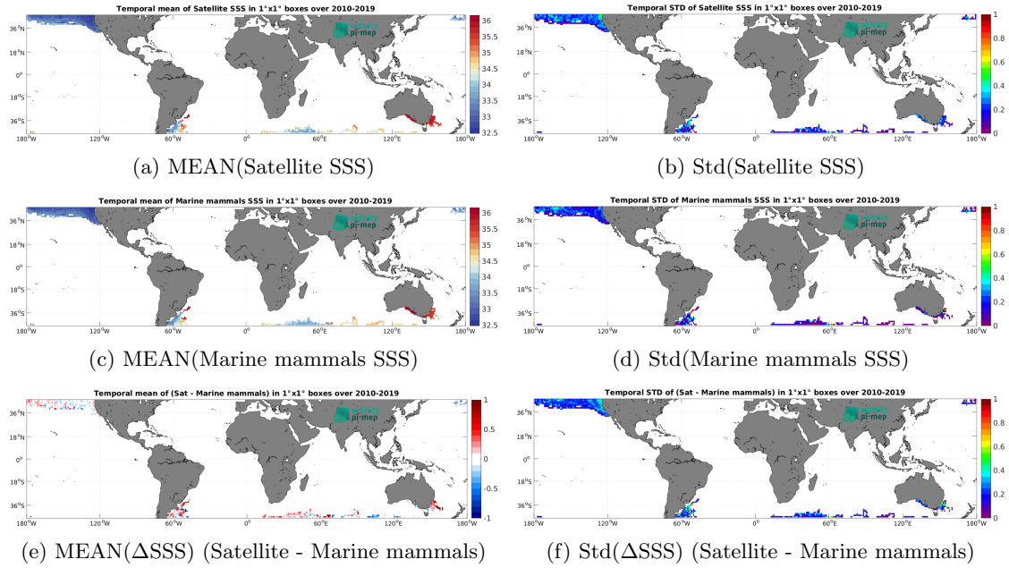
Figure 6: Temporal mean (left) and Std (right) of SSS from SMOS SSS L3 v9 - 9 Days (CATDS-CEC-LOCEAN) (top), Marine mammals (middle), and of \Delta SSS (Satellite - Marine mammals). Only match-up pairs are used to generate these maps.
