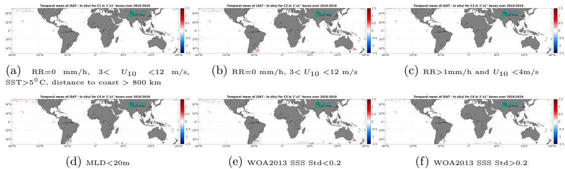
Figure 12: Temporal mean gridded over spatial boxes of size 1^{\circ}\times 1^{\circ} of \Delta\text{SSS} (SMOS SSS L3 v9 - 9 Days (CATDS-CEC-LOCEAN) - Marine mammals) for 6 different subdatasets corresponding to: RR=0 mm/h, 3 < U_{10} < 12 m/s, SST > 5^{\circ}\text{C} , distance to coast > 800 km (a), RR=0 mm/h, 3 < U_{10} < 12 m/s (b), RR > 1\text{mm/h} and U_{10} < 4\text{m/s} (c), MLD < 20\text{m} (d), WOA2013 SSS Std < 0.2 (e), WOA2013 SSS Std > 0.2 (f).
