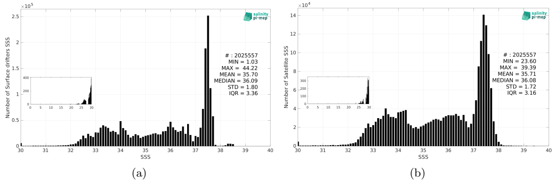
Figure 2: Histograms of SSS from Surface drifters (a) and SMOS SSS L3 v9 - 9 Days (CATDS-CEC-LOCEAN) (b) considering all match-up pairs per bins of 0.1 over the Mid-Low Latitudes 45N-45S Pi-MEP region and for the full satellite product period.
