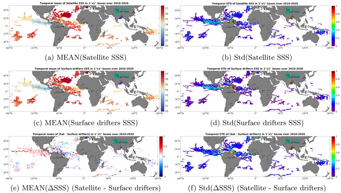
Figure 5: Temporal mean (left) and Std (right) of SSS from SMOS SSS L3 v9 - 9 Days (CATDS-CEC-LOCEAN) (top), Surface drifters (middle), and of \Delta SSS (Satellite - Surface drifters). Only match-up pairs are used to generate these maps.
