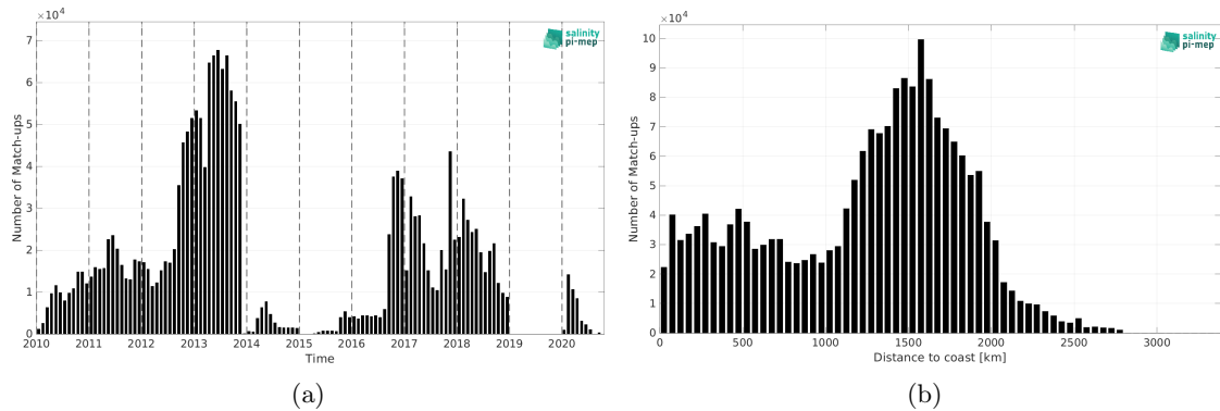
Figure 1: Number of match-ups between Surface drifters and SMOS SSS L3 v9 - 9 Days (CATDS-CEC-LOCEAN) SSS as a function of time (a) and as function of the distance to coast (b) over the Mid-Low Latitudes 45N-45S Pi-MEP region and for the full satellite product period.
