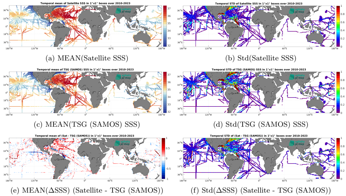
Figure 7: Temporal mean (left) and Std (right) of SSS from SMOS SSS L3 v9 - 18 Days (CATDS-CEC-LOCEAN) (top), TSG (SAMOS) (middle), and of \Delta SSS (Satellite - TSG (SAMOS)). Only match-up pairs are used to generate these maps.
