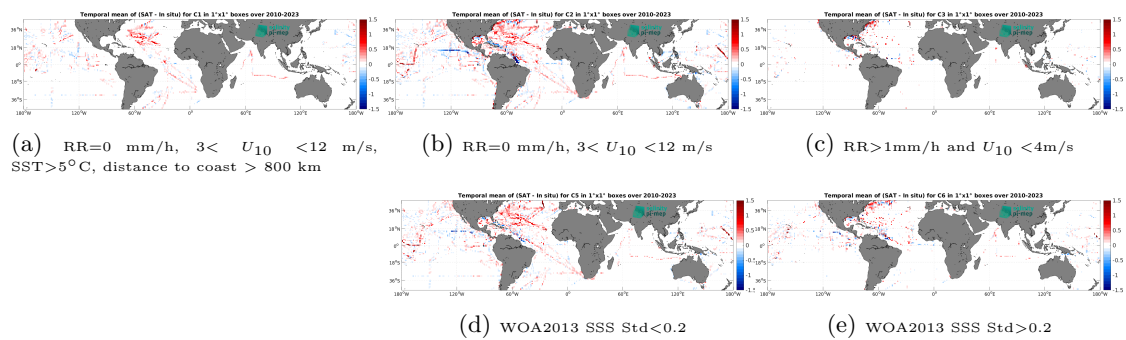
Figure 14: Temporal mean gridded over spatial boxes of size 1^\circ \times 1^\circ of \Delta SSS (SMOS SSS L3 v9 - 18 Days (CATDS-CEC-LOCEAN) - TSG (SAMOS)) for 5 different subdatasets corresponding to:RR=0 mm/h, 3 < U_{10} < 12 m/s, SST >5^\circ C, distance to coast > 800 km (a), RR=0 mm/h, 3 < U_{10} < 12 m/s (b), RR >1 mm/h and U_{10} < 4 m/s (c), WOA2013 SSS Std <0.2 (d), WOA2013 SSS Std >0.2 (e).
