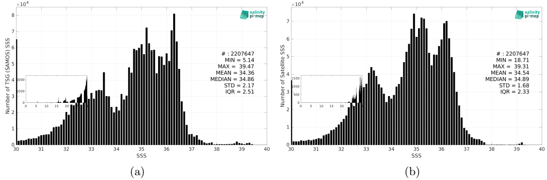
Figure 3: Histograms of SSS from TSG (SAMOS) (a) and SMOS SSS L3 v9 - 18 Days (CATDS-CEC-LOCEAN) (b) considering all match-up pairs per bins of 0.1 over the Mid-Low Latitudes 45N-45S Pi-MEP region and for the full satellite product period.
