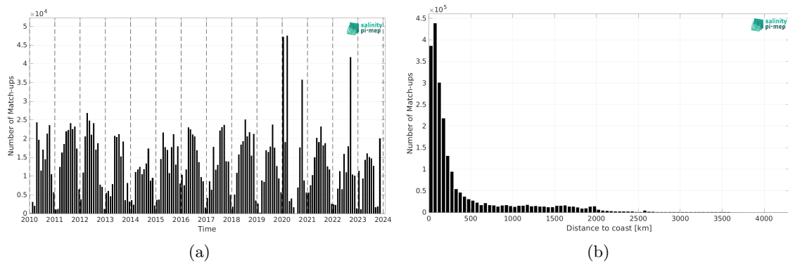
Figure 2: Number of match-ups between TSG (SAMOS) and SMOS SSS L3 v9 - 18 Days (CATDS-CEC-LOCEAN) SSS as a function of time (a) and as function of the distance to coast (b) over the Mid-Low Latitudes 45N-45S Pi-MEP region and for the full satellite product period.
