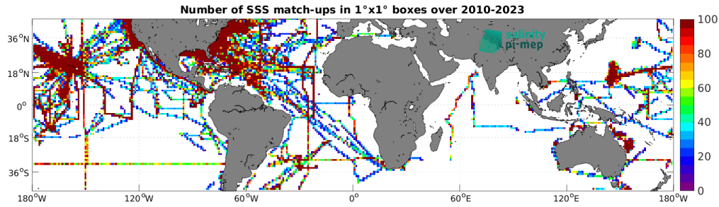
Figure 5: Number of SSS match-ups between TSG (SAMOS) SSS and the SMOS SSS L3 v9 - 18 Days (CATDS-CEC-LOCEAN) SSS product for the Mid-Low Latitudes 45N-45S Pi-MEP region over 1^\circ \times 1^\circ boxes and for the full satellite product period.
