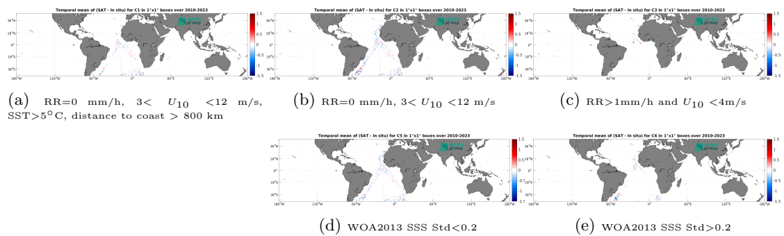
Figure 14: Temporal mean gridded over spatial boxes of size 1^\circ \times 1^\circ of \Delta\text{SSS} (SMOS SSS L3 v9 - 18 Days (CATDS-CEC-LOCEAN) - TSG (Polarstern)) for 5 different subdatasets corresponding to:RR=0 mm/h, 3 < U_{10} < 12 m/s, SST > 5°C, distance to coast > 800 km (a), RR=0 mm/h, 3 < U_{10} < 12 m/s (b), RR > 1mm/h and U_{10} < 4 m/s (c), WOA2013 SSS Std < 0.2 (d), WOA2013 SSS Std > 0.2 (e).
