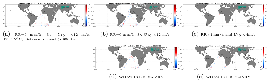
Figure 14: Temporal mean gridded over spatial boxes of size 1^\circ \times 1^\circ of \Delta SSS (SMOS SSS L3 v9 - 18 Days (CATDS-CEC-LOCEAN) - TSG (Polarstern)) for 5 different subdatasets corresponding to:RR=0 mm/h, 3 < U_{10} < 12 m/s, SST > 5°C, distance to coast > 800 km (a), RR=0 mm/h, 3 < U_{10} < 12 m/s (b), RR > 1mm/h and U_{10} < 4 m/s (c), WOA2013 SSS Std < 0.2 (d), WOA2013 SSS Std > 0.2 (e).
