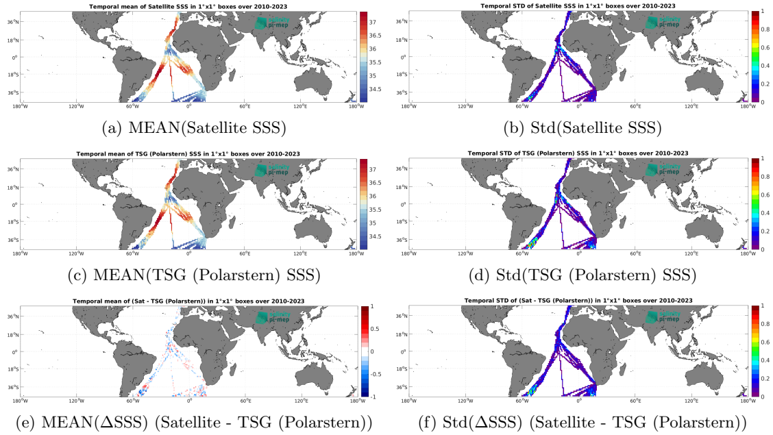
Figure 7: Temporal mean (left) and Std (right) of SSS from SMOS SSS L3 v9 - 18 Days (CATDS-CEC-LOCEAN) (top), TSG (Polarstern) (middle), and of \Delta SSS (Satellite - TSG (Polarstern)). Only match-up pairs are used to generate these maps.
