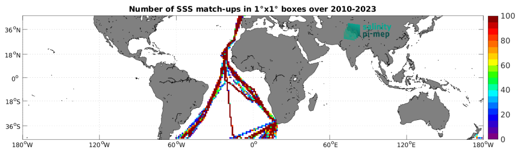
Figure 5: Number of SSS match-ups between TSG (Polarstern) SSS and the SMOS SSS L3 v9 - 18 Days (CATDS-CEC-LOCEAN) SSS product for the Mid-Low Latitudes 45N-45S Pi-MEP region over 1^\circ \times 1^\circ boxes and for the full satellite product period.
