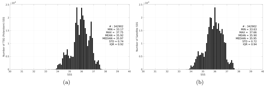
Figure 3: Histograms of SSS from TSG (Polarstern) (a) and SMOS SSS L3 v9 - 18 Days (CATDS-CEC-LOCEAN) (b) considering all match-up pairs per bins of 0.1 over the Mid-Low Latitudes 45N-45S Pi-MEP region and for the full satellite product period.
