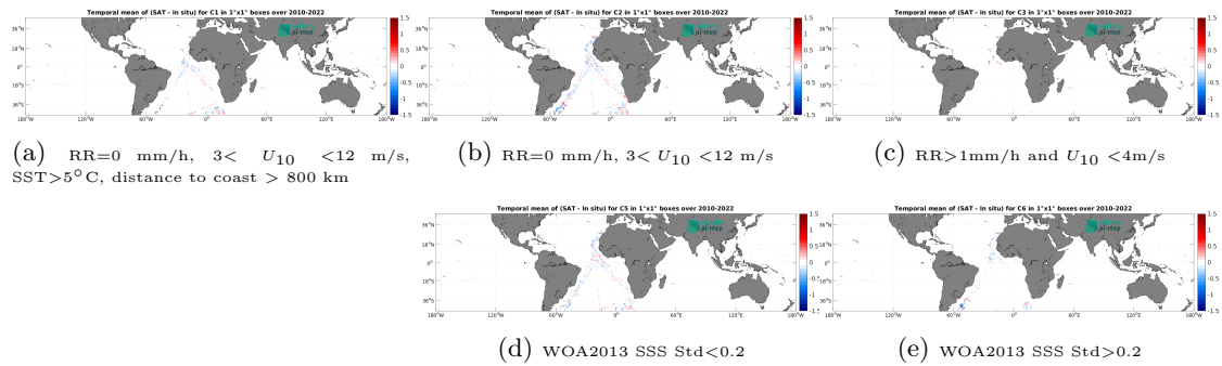
Figure 12: Temporal mean gridded over spatial boxes of size 1^\circ \times 1^\circ of \Delta\text{SSS} (SMOS SSS L3 v9 - 18 Days (CATDS-CEC-LOCEAN) - TSG (Polarstern)) for 5 different subdatasets corresponding to: RR=0 mm/h, 3 < U_{10} < 12 m/s, SST > 5^\circ\text{C} , distance to coast > 800 km (a), RR=0 mm/h, 3 < U_{10} < 12 m/s (b), RR > 1 mm/h and U_{10} < 4 m/s (c), WOA2013 SSS Std < 0.2 (d), WOA2013 SSS Std > 0.2 (e).
