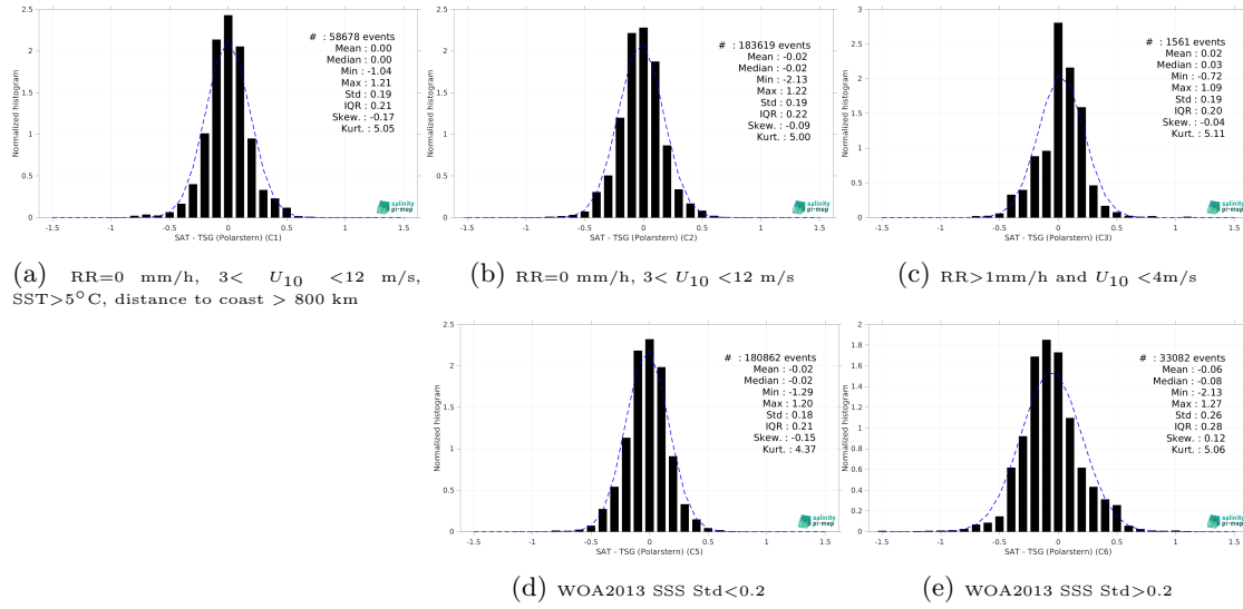
Figure 13: Normalized histogram of \Delta SSS (SMOS SSS L3 v9 - 18 Days (CATDS-CEC-LOCEAN) - TSG (Polarstern)) for 5 different subdatasets corresponding to: RR=0 mm/h, 3 < U_{10} < 12 m/s, SST>5°C, distance to coast > 800 km (a), RR=0 mm/h, 3 < U_{10} < 12 m/s (b), RR>1mm/h and U_{10} < 4 m/s (c), WOA2013 SSS Std<0.2 (d), WOA2013 SSS Std>0.2 (e).
