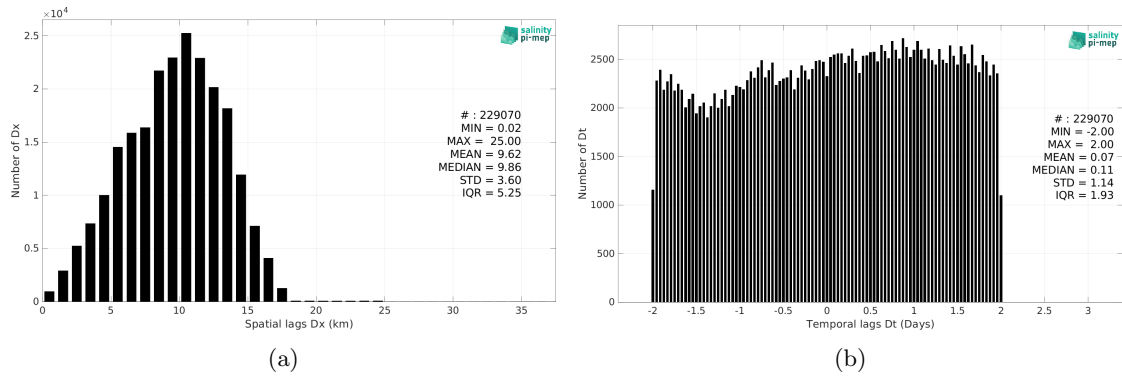
Figure 5: Histograms of the spatial (a) and temporal (b) lags between the location/time of the TSG (Polarstern) measurement and the date of the corresponding SMOS SSS L3 v9 - 18 Days (CATDS-CEC-LOCEAN) SSS pixel.
