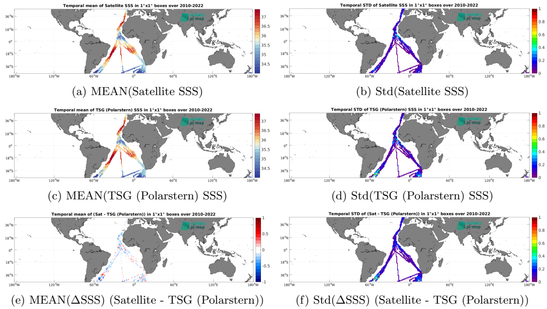
Figure 6: Temporal mean (left) and Std (right) of SSS from SMOS SSS L3 v9 - 18 Days (CATDS-CEC-LOCEAN) (top), TSG (Polarstern) (middle), and of \Delta SSS (Satellite - TSG (Polarstern)). Only match-up pairs are used to generate these maps.
