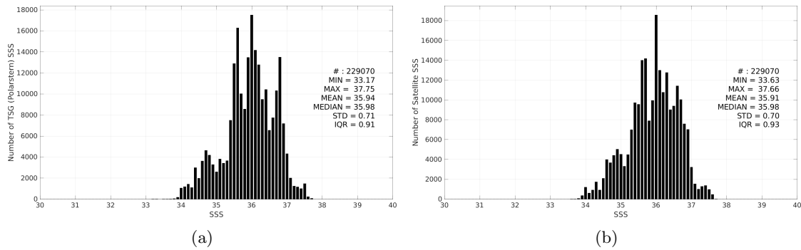
Figure 2: Histograms of SSS from TSG (Polarstern) (a) and SMOS SSS L3 v9 - 18 Days (CATDS-CEC-LOCEAN) (b) considering all match-up pairs per bins of 0.1 over the Mid-Low Latitudes 45N-45S Pi-MEP region and for the full satellite product period.
