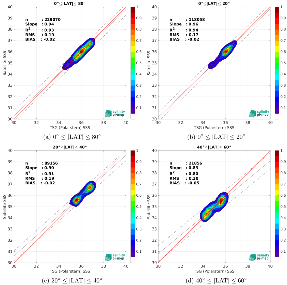
Figure 9: Contour maps of the concentration of SMOS SSS L3 v9 - 18 Days (CATDS-CEC-LOCEAN) SSS ( y -axis) versus TSG (Polarstern) SSS ( x -axis) at match-up pairs for different latitude bands. For each plot, the red line shows x=y . The black thin and dashed lines indicate a linear fit through the data cloud and the \pm 95\% confidence levels, respectively. The number match-up pairs n , the slope and R^2 coefficient of the linear fit, the root mean square (RMS) and the mean bias between satellite and in situ data are indicated for each latitude band in each plots.
