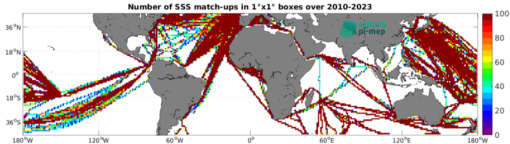
Figure 5: Number of SSS match-ups between TSG (LEGOS-DM) SSS and the SMOS SSS L3 v9 - 18 Days (CATDS-CEC-LOCEAN) SSS product for the Mid-Low Latitudes 45N-45S Pi-MEP region over 1^{\circ} \times 1^{\circ} boxes and for the full satellite product period.
