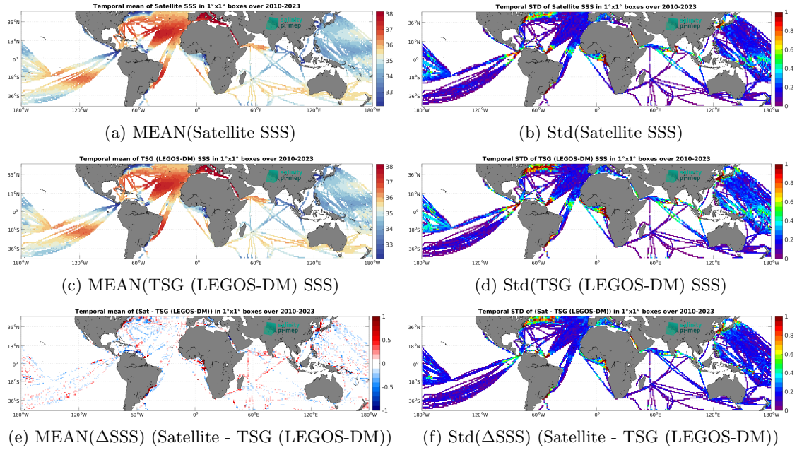
Figure 7: Temporal mean (left) and Std (right) of SSS from SMOS SSS L3 v9 - 18 Days (CATDS-CEC-LOCEAN) (top), TSG (LEGOS-DM) (middle), and of \Delta SSS (Satellite - TSG (LEGOS-DM)). Only match-up pairs are used to generate these maps.
