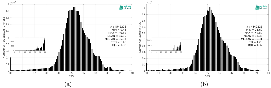
Figure 3: Histograms of SSS from TSG (LEGOS-DM) (a) and SMOS SSS L3 v9 - 18 Days (CATDS-CEC-LOCEAN) (b) considering all match-up pairs per bins of 0.1 over the Mid-Low Latitudes 45N-45S Pi-MEP region and for the full satellite product period.
