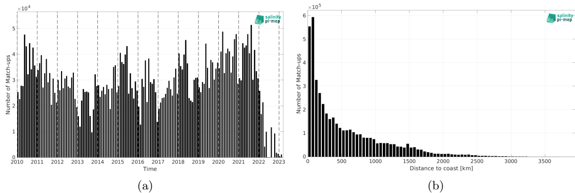
Figure 2: Number of match-ups between TSG (LEGOS-DM) and SMOS SSS L3 v9 - 18 Days (CATDS-CEC-LOCEAN) SSS as a function of time (a) and as function of the distance to coast (b) over the Mid-Low Latitudes 45N-45S Pi-MEP region and for the full satellite product period.
