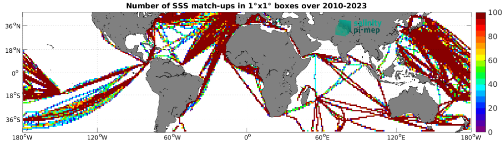
Figure 5: Number of SSS match-ups between TSG (LEGOS-DM) SSS and the SMOS SSS L3 v9 - 18 Days (CATDS-CEC-LOCEAN) SSS product for the Mid-Low Latitudes 45N-45S Pi-MEP region over 1^\circ \times 1^\circ boxes and for the full satellite product period.
