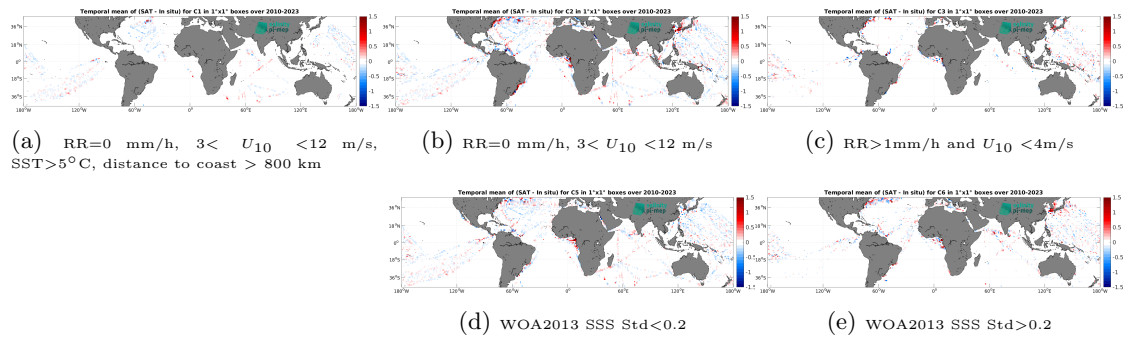
Figure 12: Temporal mean gridded over spatial boxes of size 1^\circ \times 1^\circ of \Delta SSS (SMOS SSS L3 v9 - 18 Days (CATDS-CEC-LOCEAN) - TSG (LEGOS-DM)) for 5 different subdatasets corresponding to:RR=0 mm/h, 3 < U_{10} < 12 m/s, SST >5^\circ C, distance to coast > 800 km (a), RR=0 mm/h, 3 < U_{10} < 12 m/s (b), RR >1 mm/h and U_{10} < 4 m/s (c), WOA2013 SSS Std <0.2 (d), WOA2013 SSS Std >0.2 (e).
