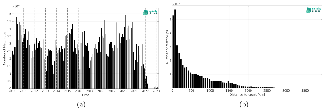
Figure 1: Number of match-ups between TSG (LEGOS-DM) and SMOS SSS L3 v9 - 18 Days (CATDS-CEC-LOCEAN) SSS as a function of time (a) and as function of the distance to coast (b) over the Mid-Low Latitudes 45N-45S Pi-MEP region and for the full satellite product period.
