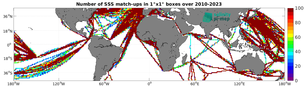
Figure 4: Number of SSS match-ups between TSG (LEGOS-DM) SSS and the SMOS SSS L3 v9 - 18 Days (CATDS-CEC-LOCEAN) SSS product for the Mid-Low Latitudes 45N-45S Pi-MEP region over 1^\circ \times 1^\circ boxes and for the full satellite product period.
