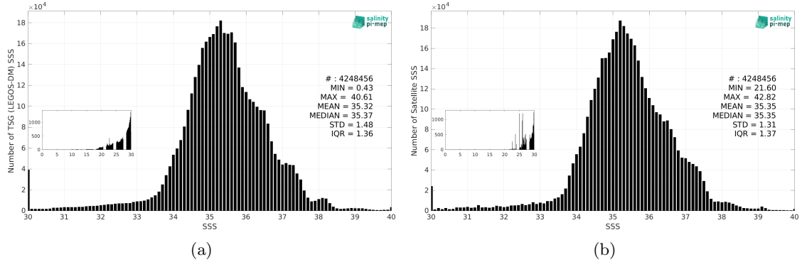
Figure 2: Histograms of SSS from TSG (LEGOS-DM) (a) and SMOS SSS L3 v9 - 18 Days (CATDS-CEC-LOCEAN) (b) considering all match-up pairs per bins of 0.1 over the Mid-Low Latitudes 45N-45S Pi-MEP region and for the full satellite product period.
