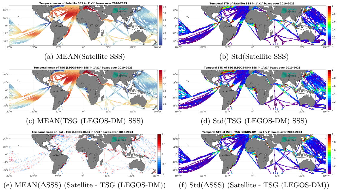
Figure 6: Temporal mean (left) and Std (right) of SSS from SMOS SSS L3 v9 - 18 Days (CATDS-CEC-LOCEAN) (top), TSG (LEGOS-DM) (middle), and of \Delta SSS (Satellite - TSG (LEGOS-DM)). Only match-up pairs are used to generate these maps.
