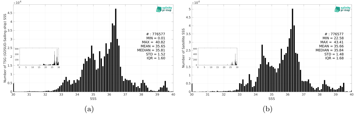
Figure 3: Histograms of SSS from TSG (GOSUD-Sailing-ship) (a) and SMOS SSS L3 v9 - 18 Days (CATDS-CEC-LOCEAN) (b) considering all match-up pairs per bins of 0.1 over the Mid-Low Latitudes 45N-45S Pi-MEP region and for the full satellite product period.
