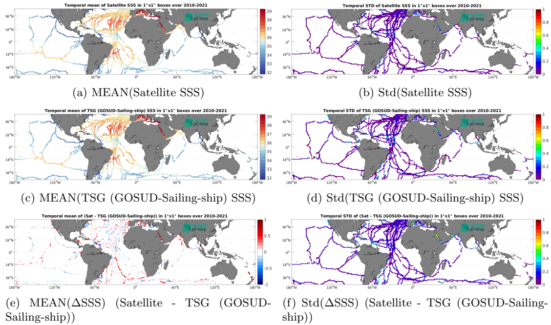
Figure 7: Temporal mean (left) and Std (right) of SSS from SMOS SSS L3 v9 - 18 Days (CATDS-CEC-LOCEAN) (top), TSG (GOSUD-Sailing-ship) (middle), and of \Delta SSS (Satellite - TSG (GOSUD-Sailing-ship)). Only match-up pairs are used to generate these maps.
