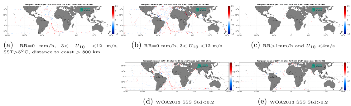
Figure 14: Temporal mean gridded over spatial boxes of size 1^\circ \times 1^\circ of \Delta SSS (SMOS SSS L3 v9 - 18 Days (CATDS-CEC-LOCEAN) - TSG (GOSUD-Sailing-ship)) for 5 different subdatasets corresponding to: RR=0 mm/h, 3 < U_{10} < 12 m/s, SST > 5°C, distance to coast > 800 km (a), RR=0 mm/h, 3 < U_{10} < 12 m/s (b), RR > 1mm/h and U_{10} < 4 m/s (c), WOA2013 SSS Std < 0.2 (d), WOA2013 SSS Std > 0.2 (e).
