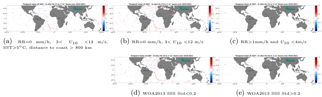
Figure 12: Temporal mean gridded over spatial boxes of size 1^\circ \times 1^\circ of \Delta SSS (SMOS SSS L3 v9 - 18 Days (CATDS-CEC-LOCEAN) - TSG (GOSUD-Sailing-ship)) for 5 different subdatasets corresponding to: RR=0 mm/h, 3 < U_{10} < 12 m/s, SST > 5^\circ\text{C} , distance to coast > 800 km (a), RR=0 mm/h, 3 < U_{10} < 12 m/s (b), RR > 1 mm/h and U_{10} < 4 m/s (c), WOA2013 SSS Std < 0.2 (d), WOA2013 SSS Std > 0.2 (e).
