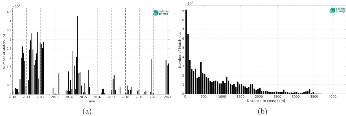
Figure 1: Number of match-ups between TSG (GOSUD-Sailing-ship) and SMOS SSS L3 v9 - 18 Days (CATDS-CEC-LOCEAN) SSS as a function of time (a) and as function of the distance to coast (b) over the Mid-Low Latitudes 45N-45S Pi-MEP region and for the full satellite product period.
