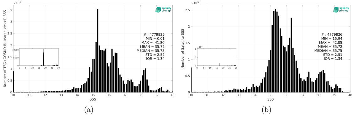
Figure 3: Histograms of SSS from TSG (GOSUD-Research-vessel) (a) and SMOS SSS L3 v9 - 18 Days (CATDS-CEC-LOCEAN) (b) considering all match-up pairs per bins of 0.1 over the Mid-Low Latitudes 45N-45S Pi-MEP region and for the full satellite product period.
