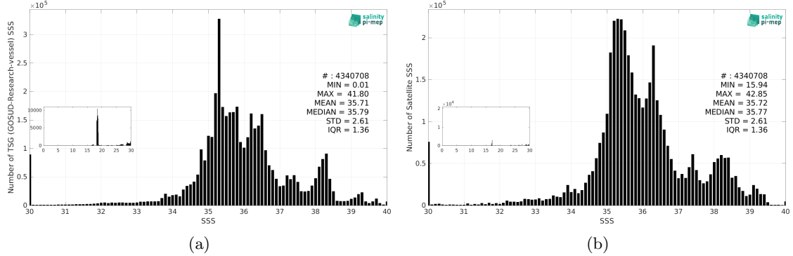
Figure 3: Histograms of SSS from TSG (GOSUD-Research-vessel) (a) and SMOS SSS L3 v9 - 18 Days (CATDS-CEC-LOCEAN) (b) considering all match-up pairs per bins of 0.1 over the Mid-Low Latitudes 45N-45S Pi-MEP region and for the full satellite product period.
