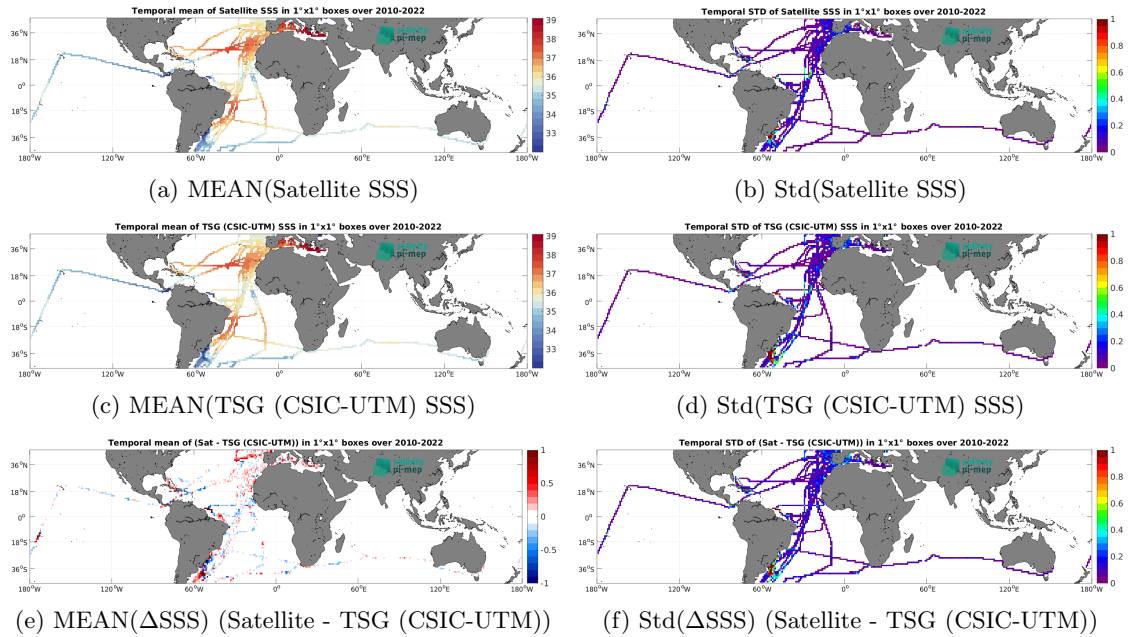
Figure 6: Temporal mean (left) and Std (right) of SSS from SMOS SSS L3 v9 - 18 Days (CATDS-CEC-LOCEAN) (top), TSG (CSIC-UTM) (middle), and of \Delta SSS (Satellite - TSG (CSIC-UTM)). Only match-up pairs are used to generate these maps.
