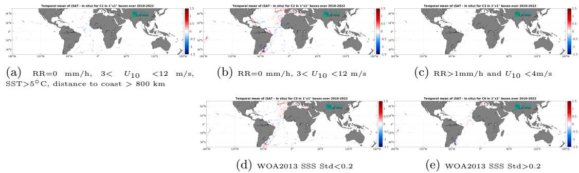
Figure 12: Temporal mean gridded over spatial boxes of size 1^\circ \times 1^\circ of \Delta SSS (SMOS SSS L3 v9 - 18 Days (CATDS-CEC-LOCEAN) - TSG (CSIC-UTM)) for 5 different subdatasets corresponding to:RR=0 mm/h, 3 < U_{10} < 12 m/s, SST >5^\circ\text{C} , distance to coast > 800 km (a), RR=0 mm/h, 3 < U_{10} < 12 m/s (b), RR >1 mm/h and U_{10} < 4 m/s (c), WOA2013 SSS Std <0.2 (d), WOA2013 SSS Std >0.2 (e).
