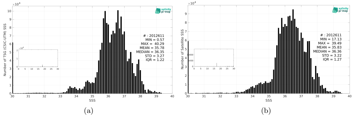
Figure 2: Histograms of SSS from TSG (CSIC-UTM) (a) and SMOS SSS L3 v9 - 18 Days (CATDS-CEC-LOCEAN) (b) considering all match-up pairs per bins of 0.1 over the Mid-Low Latitudes 45N-45S Pi-MEP region and for the full satellite product period.
