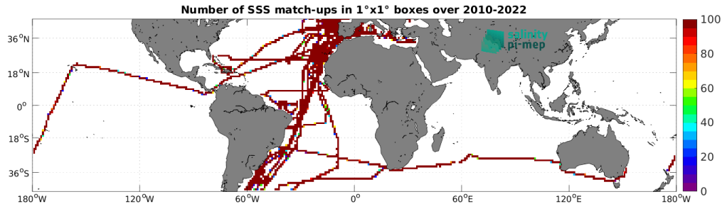
Figure 4: Number of SSS match-ups between TSG (CSIC-UTM) SSS and the SMOS SSS L3 v9 - 18 Days (CATDS-CEC-LOCEAN) SSS product for the Mid-Low Latitudes 45N-45S Pi-MEP region over 1^\circ \times 1^\circ boxes and for the full satellite product period.
