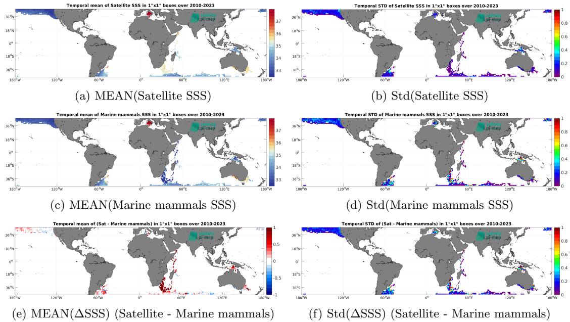
Figure 7: Temporal mean (left) and Std (right) of SSS from SMOS SSS L3 v9 - 18 Days (CATDS-CEC-LOCEAN) (top), Marine mammals (middle), and of \Delta SSS (Satellite - Marine mammals). Only match-up pairs are used to generate these maps.
