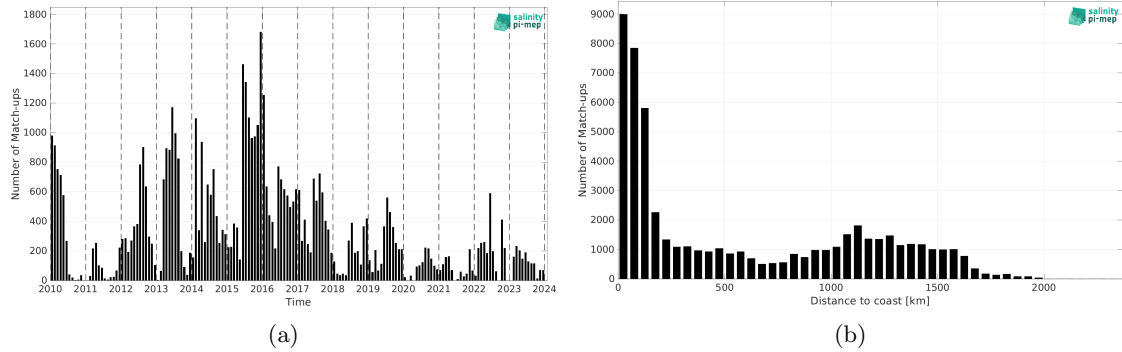
Figure 2: Number of match-ups between Marine mammals and SMOS SSS L3 v9 - 18 Days (CATDS-CEC-LOCEAN) SSS as a function of time (a) and as function of the distance to coast (b) over the Mid-Low Latitudes 45N-45S Pi-MEP region and for the full satellite product period.
