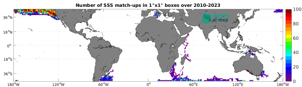
Figure 5: Number of SSS match-ups between Marine mammals SSS and the SMOS SSS L3 v9 - 18 Days (CATDS-CEC-LOCEAN) SSS product for the Mid-Low Latitudes 45N-45S Pi-MEP region over 1^\circ \times 1^\circ boxes and for the full satellite product period.
