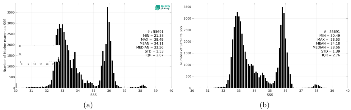
Figure 3: Histograms of SSS from Marine mammals (a) and SMOS SSS L3 v9 - 18 Days (CATDS-CEC-LOCEAN) (b) considering all match-up pairs per bins of 0.1 over the Mid-Low Latitudes 45N-45S Pi-MEP region and for the full satellite product period.
