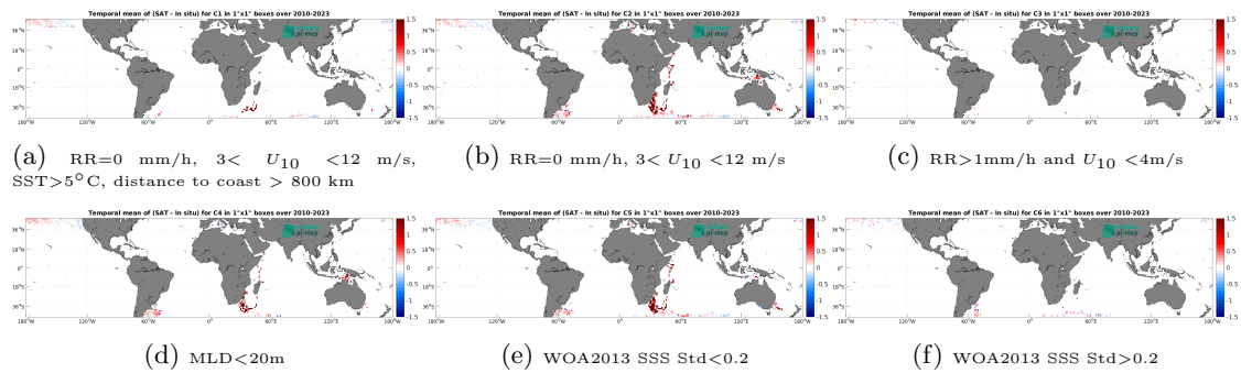
Figure 14: Temporal mean gridded over spatial boxes of size 1^\circ \times 1^\circ of \Delta SSS (SMOS SSS L3 v9 - 18 Days (CATDS-CEC-LOCEAN) - Marine mammals) for 6 different subdatasets corresponding to: RR=0 mm/h, 3 < U_{10} < 12 m/s, SST > 5°C, distance to coast > 800 km (a), RR=0 mm/h, 3 < U_{10} < 12 m/s (b), RR > 1mm/h and U_{10} < 4 m/s (c),MLD < 20m (d),WOA2013 SSS Std < 0.2 (e),WOA2013 SSS Std > 0.2 (f).
