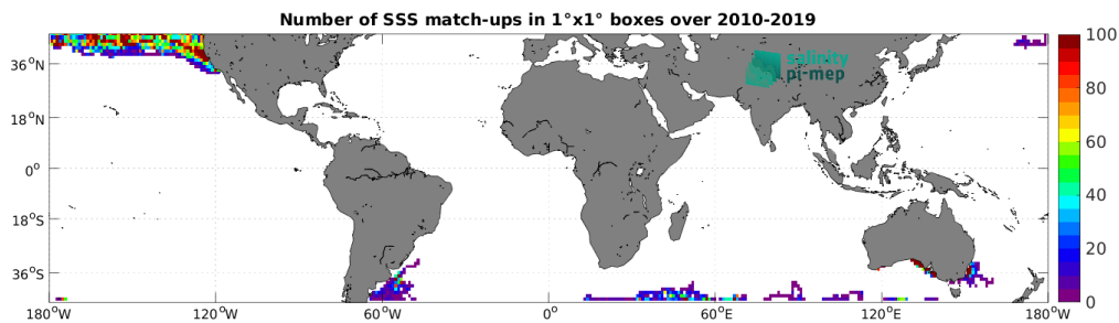
Figure 4: Number of SSS match-ups between Marine mammals SSS and the SMOS SSS L3 v9 - 18 Days (CATDS-CEC-LOCEAN) SSS product for the Mid-Low Latitudes 45N-45S Pi-MEP region over 1^\circ \times 1^\circ boxes and for the full satellite product period.
