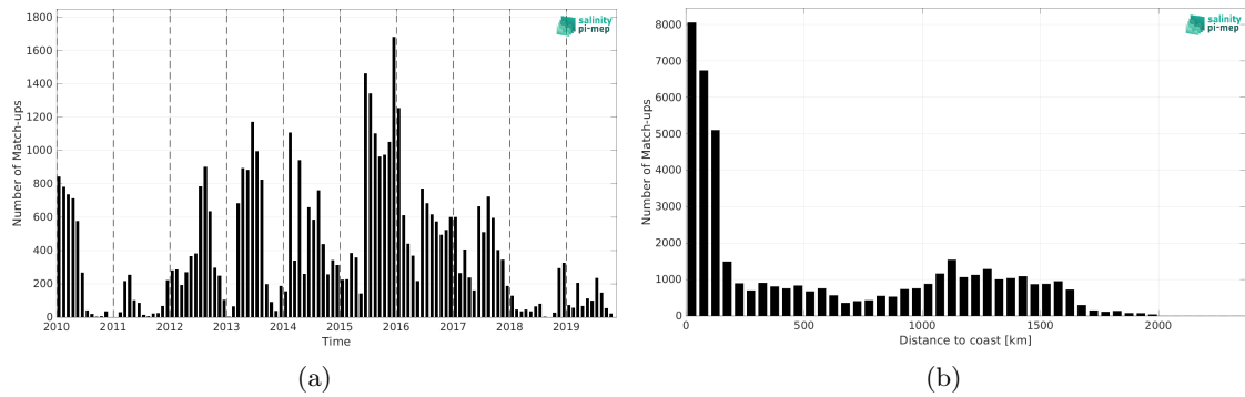
Figure 1: Number of match-ups between Marine mammals and SMOS SSS L3 v9 - 18 Days (CATDS-CEC-LOCEAN) SSS as a function of time (a) and as function of the distance to coast (b) over the Mid-Low Latitudes 45N-45S Pi-MEP region and for the full satellite product period.
