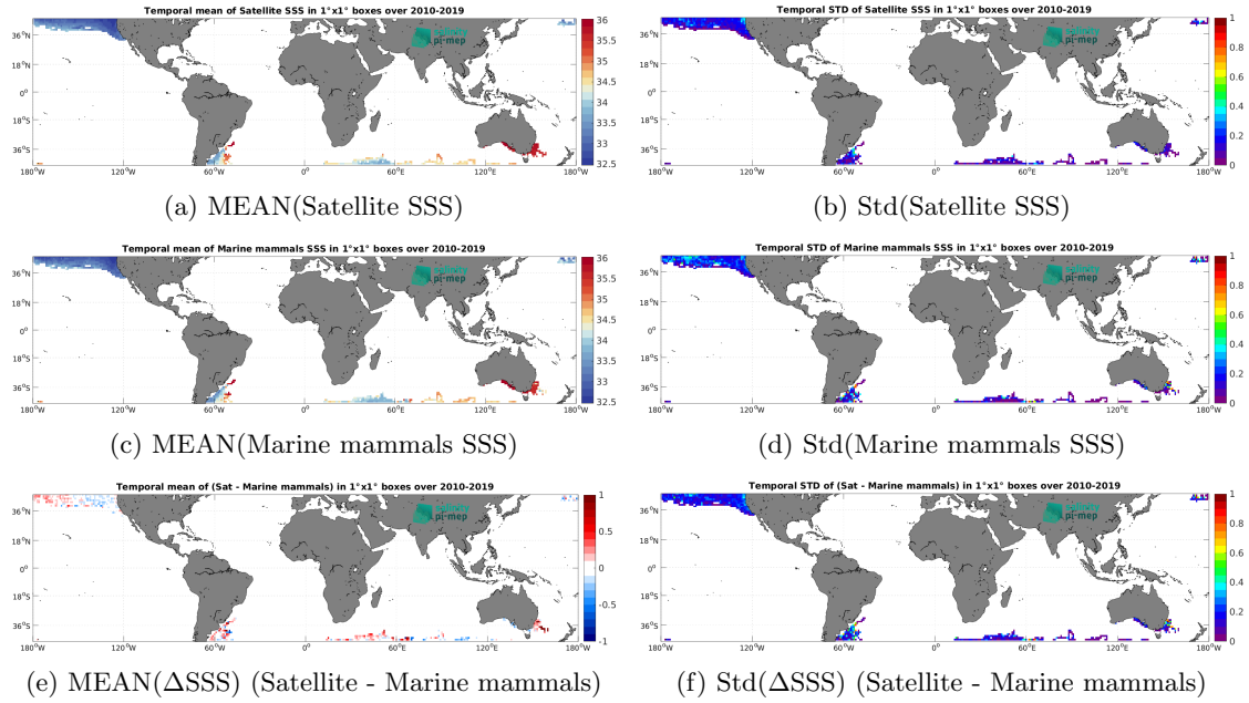
Figure 6: Temporal mean (left) and Std (right) of SSS from SMOS SSS L3 v9 - 18 Days (CATDS-CEC-LOCEAN) (top), Marine mammals (middle), and of \Delta SSS (Satellite - Marine mammals). Only match-up pairs are used to generate these maps.
