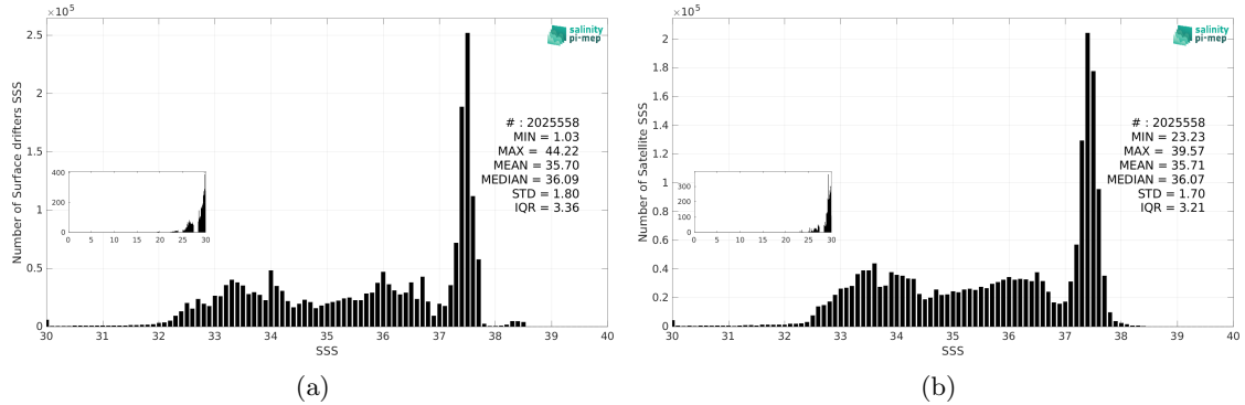
Figure 3: Histograms of SSS from Surface drifters (a) and SMOS SSS L3 v9 - 18 Days (CATDS-CEC-LOCEAN) (b) considering all match-up pairs per bins of 0.1 over the Mid-Low Latitudes 45N-45S Pi-MEP region and for the full satellite product period.
