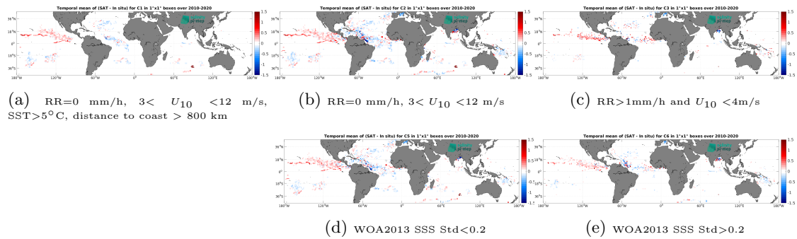
Figure 13: Temporal mean gridded over spatial boxes of size 1^\circ \times 1^\circ of \Delta\text{SSS} (SMOS SSS L3 v9 - 18 Days (CATDS-CEC-LOCEAN) - Surface drifters) for 5 different subdatasets corresponding to:RR=0 mm/h, 3 < U_{10} < 12 m/s, SST >5^\circ\text{C} , distance to coast > 800 km (a), RR=0 mm/h, 3 < U_{10} < 12 m/s (b), RR >1 mm/h and U_{10} < 4 m/s (c), WOA2013 SSS Std <0.2 (d), WOA2013 SSS Std >0.2 (e).
