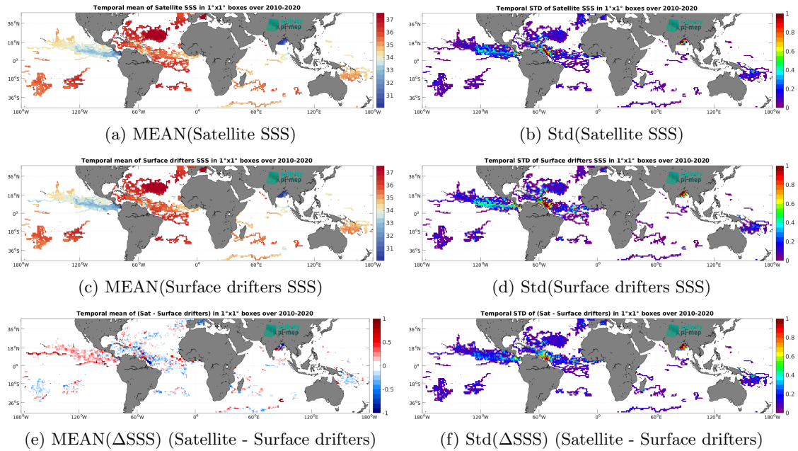
Figure 6: Temporal mean (left) and Std (right) of SSS from SMOS SSS L3 v9 - 18 Days (CATDS-CEC-LOCEAN) (top), Surface drifters (middle), and of \Delta SSS (Satellite - Surface drifters). Only match-up pairs are used to generate these maps.
