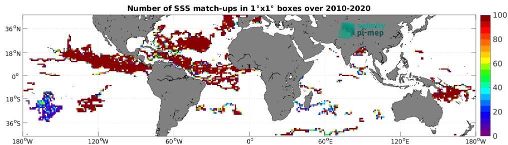
Figure 4: Number of SSS match-ups between Surface drifters SSS and the SMOS SSS L3 v9 - 18 Days (CATDS-CEC-LOCEAN) SSS product for the Mid-Low Latitudes 45N-45S Pi-MEP region over 1^\circ \times 1^\circ boxes and for the full satellite product period.
