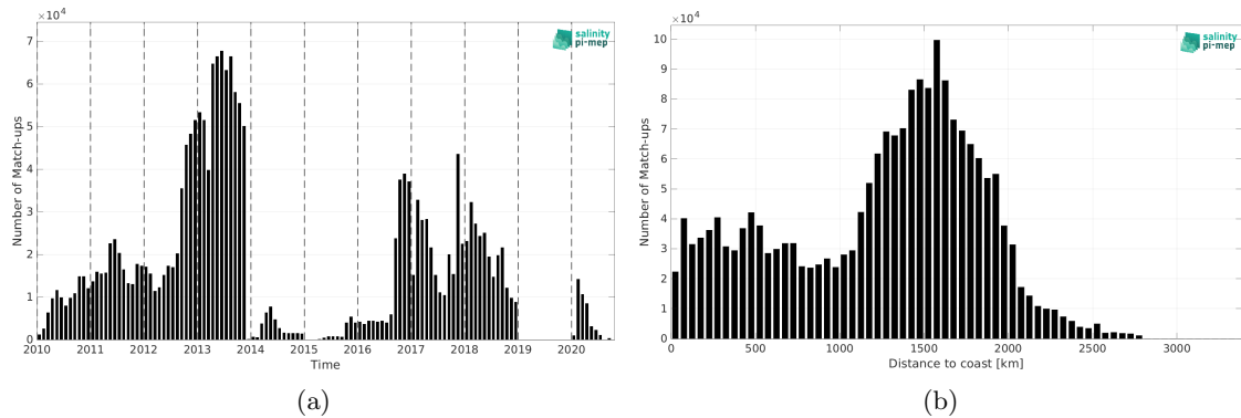
Figure 2: Number of match-ups between Surface drifters and SMOS SSS L3 v9 - 18 Days (CATDS-CEC-LOCEAN) SSS as a function of time (a) and as function of the distance to coast (b) over the Mid-Low Latitudes 45N-45S Pi-MEP region and for the full satellite product period.
