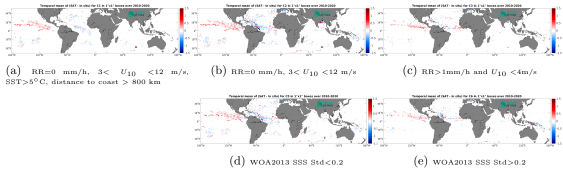
Figure 11: Temporal mean gridded over spatial boxes of size 1^\circ \times 1^\circ of \Delta SSS (SMOS SSS L3 v9 - 18 Days (CATDS-CEC-LOCEAN) - Surface drifters) for 5 different subdatasets corresponding to:RR=0 mm/h, 3 < U_{10} < 12 m/s, SST >5^\circ C, distance to coast > 800 km (a), RR=0 mm/h, 3 < U_{10} < 12 m/s (b), RR >1 mm/h and U_{10} < 4 m/s (c), WOA2013 SSS Std <0.2 (d), WOA2013 SSS Std >0.2 (e).
