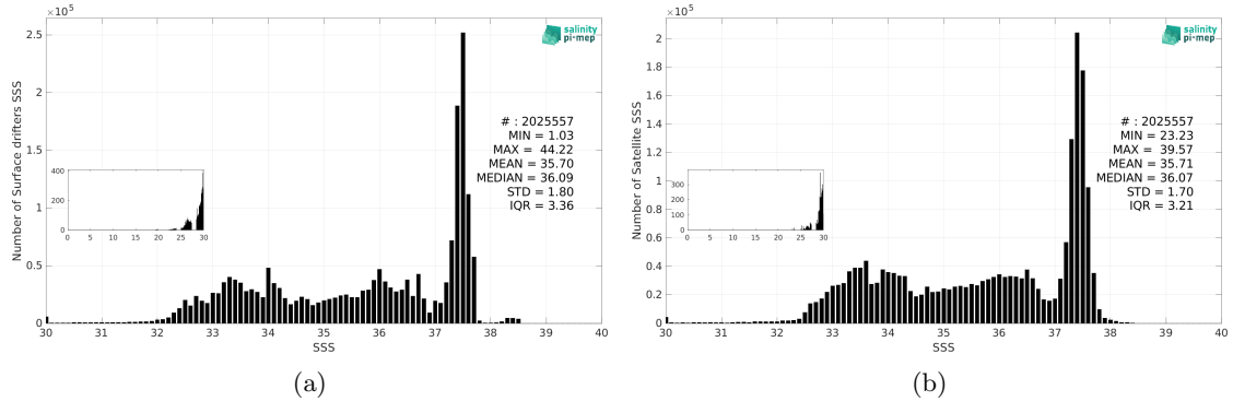
Figure 2: Histograms of SSS from Surface drifters (a) and SMOS SSS L3 v9 - 18 Days (CATDS-CEC-LOCEAN) (b) considering all match-up pairs per bins of 0.1 over the Mid-Low Latitudes 45N-45S Pi-MEP region and for the full satellite product period.
