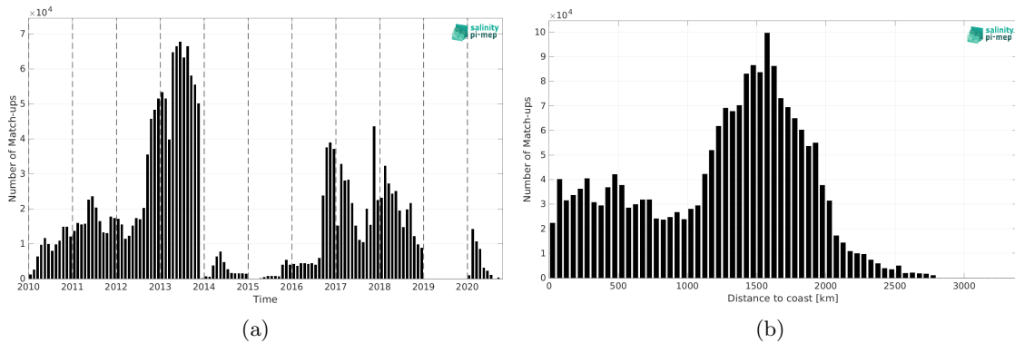
Figure 1: Number of match-ups between Surface drifters and SMOS SSS L3 v9 - 18 Days (CATDS-CEC-LOCEAN) SSS as a function of time (a) and as function of the distance to coast (b) over the Mid-Low Latitudes 45N-45S Pi-MEP region and for the full satellite product period.
