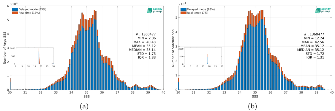
Figure 2: Histograms of SSS from Argo (a) and SMOS SSS L3 v9 - 18 Days (CATDS-CEC-LOCEAN) (b) considering all match-up pairs per bins of 0.1 over the Mid-Low Latitudes 45N-45S Pi-MEP region and for the full satellite product period.
