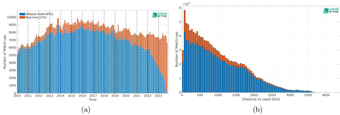
Figure 1: Number of match-ups between Argo and SMOS SSS L3 v9 - 18 Days (CATDS-CEC-LOCEAN) SSS as a function of time (a) and as function of the distance to coast (b) over the Mid-Low Latitudes 45N-45S Pi-MEP region and for the full satellite product period.
