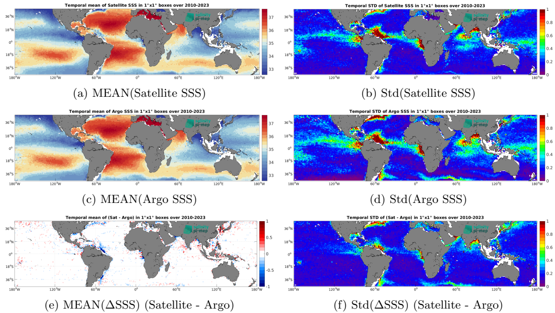
Figure 6: Temporal mean (left) and Std (right) of SSS from SMOS SSS L3 v9 - 18 Days (CATDS-CEC-LOCEAN) (top), Argo (middle), and of \Delta SSS (Satellite - Argo). Only match-up pairs are used to generate these maps.
