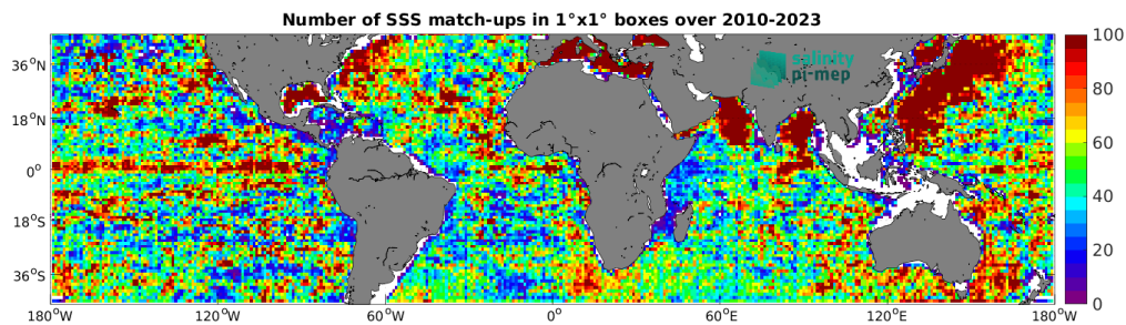
Figure 4: Number of SSS match-ups between Argo SSS and the SMOS SSS L3 v9 - 18 Days (CATDS-CEC-LOCEAN) SSS product for the Mid-Low Latitudes 45N-45S Pi-MEP region over 1^\circ \times 1^\circ boxes and for the full satellite product period.
