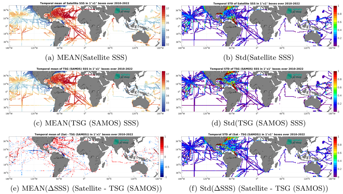
Figure 6: Temporal mean (left) and Std (right) of SSS from SMOS SSS L3 v8 - 9 Days (CATDS-CEC-LOCEAN) (top), TSG (SAMOS) (middle), and of \Delta SSS (Satellite - TSG (SAMOS)). Only match-up pairs are used to generate these maps.
