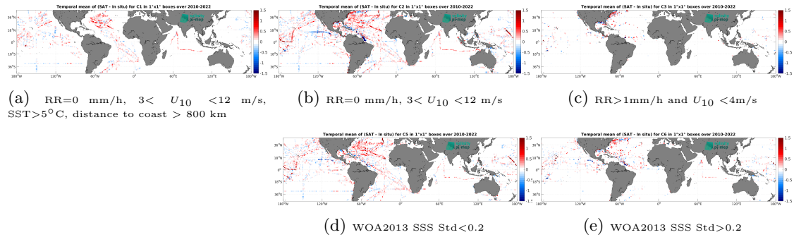
Figure 12: Temporal mean gridded over spatial boxes of size 1^\circ \times 1^\circ of \Delta SSS (SMOS SSS L3 v8 - 9 Days (CATDS-CEC-LOCEAN) - TSG (SAMOS)) for 5 different subdatasets corresponding to: RR=0 mm/h, 3 < U_{10} < 12 m/s, SST > 5^\circ C , distance to coast > 800 km (a), RR=0 mm/h, 3 < U_{10} < 12 m/s (b), RR > 1 mm/h and U_{10} < 4 m/s (c), WOA2013 SSS Std <0.2 (d), WOA2013 SSS Std >0.2 (e).
