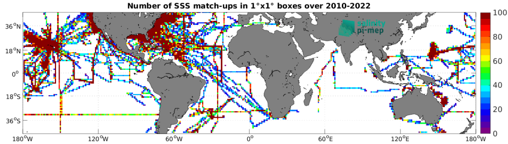
Figure 4: Number of SSS match-ups between TSG (SAMOS) SSS and the SMOS SSS L3 v8 - 9 Days (CATDS-CEC-LOCEAN) SSS product for the Mid-Low Latitudes 45N-45S Pi-MEP region over 1^\circ \times 1^\circ boxes and for the full satellite product period.
