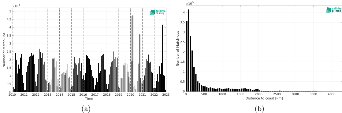
Figure 1: Number of match-ups between TSG (SAMOS) and SMOS SSS L3 v8 - 9 Days (CATDS-CEC-LOCEAN) SSS as a function of time (a) and as function of the distance to coast (b) over the Mid-Low Latitudes 45N-45S Pi-MEP region and for the full satellite product period.
