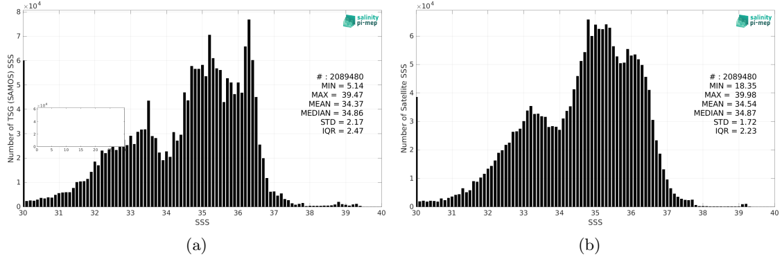
Figure 2: Histograms of SSS from TSG (SAMOS) (a) and SMOS SSS L3 v8 - 9 Days (CATDS-CEC-LOCEAN) (b) considering all match-up pairs per bins of 0.1 over the Mid-Low Latitudes 45N-45S Pi-MEP region and for the full satellite product period.
