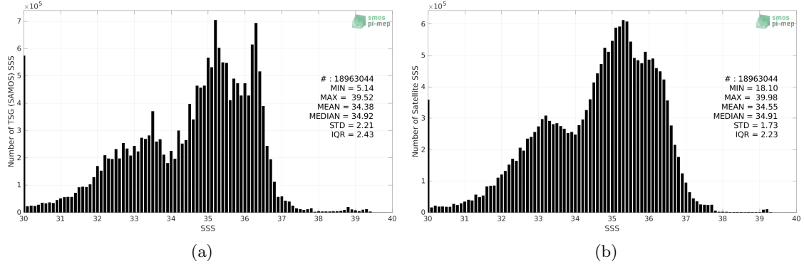
Figure 2: Histograms of SSS from TSG (SAMOS) (a) and SMOS SSS L3 v8 - 9 Days (CATDS-CECOS-LOCEAN) (b) considering all match-up pairs per bins of 0.1 over the Mid-Low Latitudes 45N-45S Pi-MEP region and for the full satellite product period.
