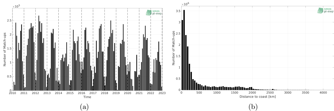
Figure 1: Number of match-ups between TSG (SAMOS) and SMOS SSS L3 v8 - 9 Days (CATDS-CECOS-LOCEAN) SSS as a function of time (a) and as function of the distance to coast (b) over the Mid-Low Latitudes 45N-45S Pi-MEP region and for the full satellite product period.
