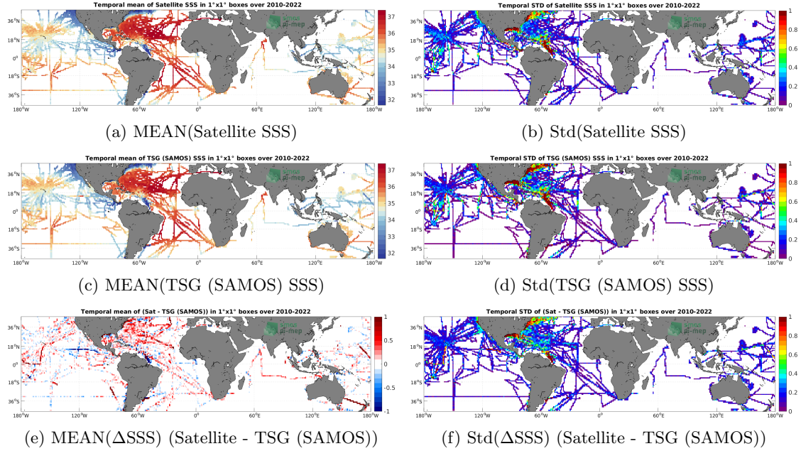
Figure 6: Temporal mean (left) and Std (right) of SSS from SMOS SSS L3 v8 - 9 Days (CATDS-CECOS-LOCEAN) (top), TSG (SAMOS) (middle), and of \Delta SSS (Satellite - TSG (SAMOS)). Only match-up pairs are used to generate these maps.
