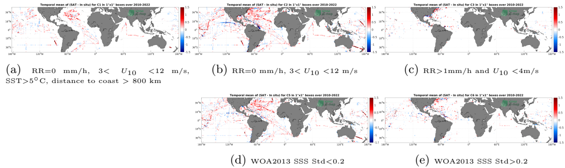
Figure 12: Temporal mean gridded over spatial boxes of size 1^\circ \times 1^\circ of \Delta\text{SSS} (SMOS SSS L3 v8 - 9 Days (CATDS-CECOS-LOCEAN) - TSG (SAMOS)) for 5 different subdatasets corresponding to:RR=0 mm/h, 3 < U_{10} < 12 m/s, SST >5^\circ\text{C} , distance to coast > 800 km (a), RR=0 mm/h, 3 < U_{10} < 12 m/s (b), RR >1 mm/h and U_{10} < 4 m/s (c), WOA2013 SSS Std <0.2 (d), WOA2013 SSS Std >0.2 (e).
