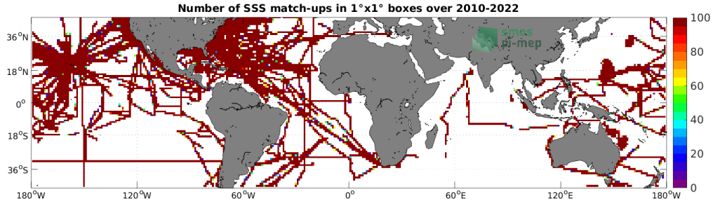
Figure 4: Number of SSS match-ups between TSG (SAMOS) SSS and the SMOS SSS L3 v8 - 9 Days (CATDS-CECOS-LOCEAN) SSS product for the Mid-Low Latitudes 45N-45S Pi-MEP region over 1^\circ \times 1^\circ boxes and for the full satellite product period.
