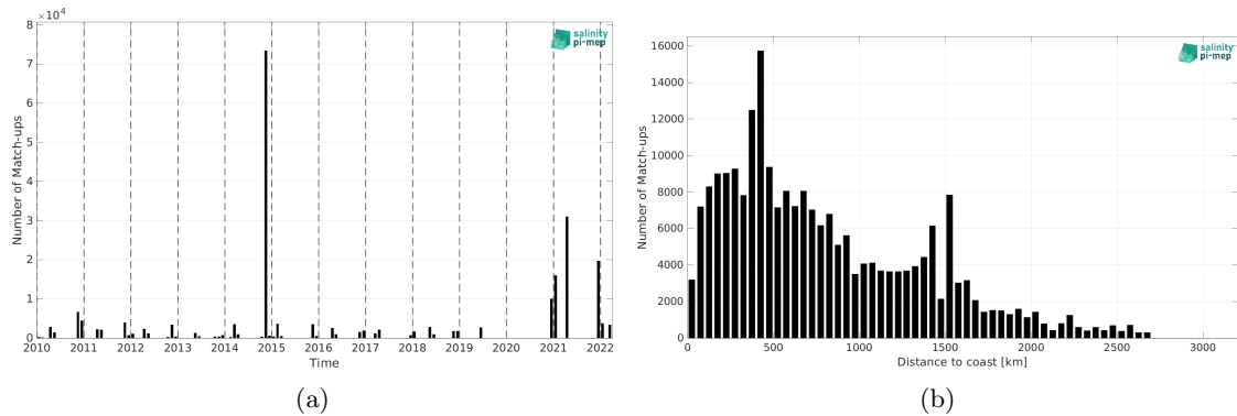
Figure 1: Number of match-ups between TSG (Polarstern) and SMOS SSS L3 v8 - 9 Days (CATDS-CEC-LOCEAN) SSS as a function of time (a) and as function of the distance to coast (b) over the Mid-Low Latitudes 45N-45S Pi-MEP region and for the full satellite product period.
