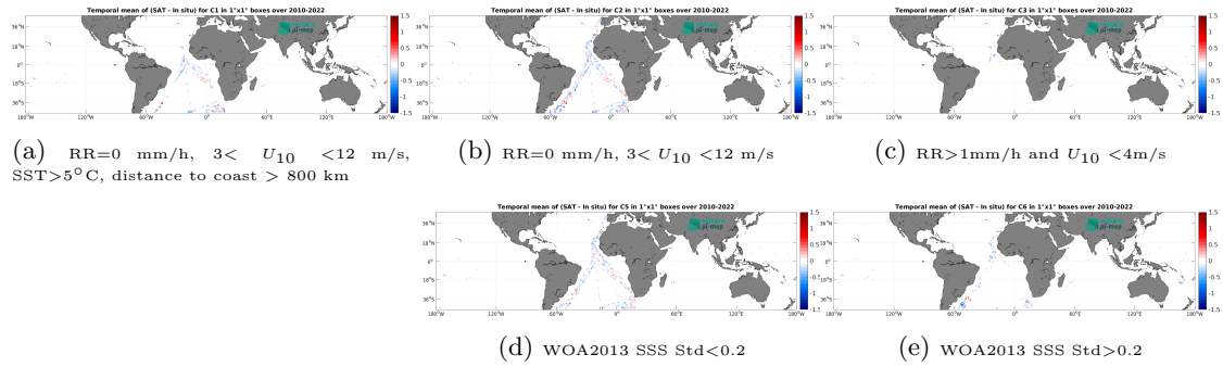
Figure 12: Temporal mean gridded over spatial boxes of size 1^\circ \times 1^\circ of \Delta SSS (SMOS SSS L3 v8 - 9 Days (CATDS-CEC-LOCEAN) - TSG (Polarstern)) for 5 different subdatasets corresponding to:RR=0 mm/h, 3 < U_{10} < 12 m/s, SST >5^\circ\text{C} , distance to coast > 800 km (a), RR=0 mm/h, 3 < U_{10} < 12 m/s (b), RR >1 mm/h and U_{10} < 4 m/s (c), WOA2013 SSS Std <0.2 (d), WOA2013 SSS Std >0.2 (e).
