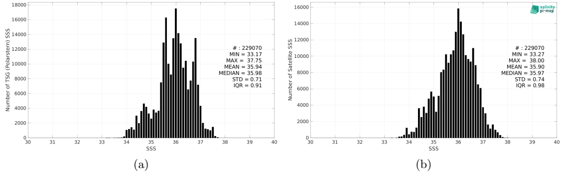
Figure 2: Histograms of SSS from TSG (Polarstern) (a) and SMOS SSS L3 v8 - 9 Days (CATDS-CEC-LOCEAN) (b) considering all match-up pairs per bins of 0.1 over the Mid-Low Latitudes 45N-45S Pi-MEP region and for the full satellite product period.
