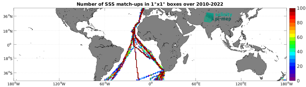
Figure 4: Number of SSS match-ups between TSG (Polarstern) SSS and the SMOS SSS L3 v8 - 9 Days (CATDS-CEC-LOCEAN) SSS product for the Mid-Low Latitudes 45N-45S Pi-MEP region over 1^\circ \times 1^\circ boxes and for the full satellite product period.
