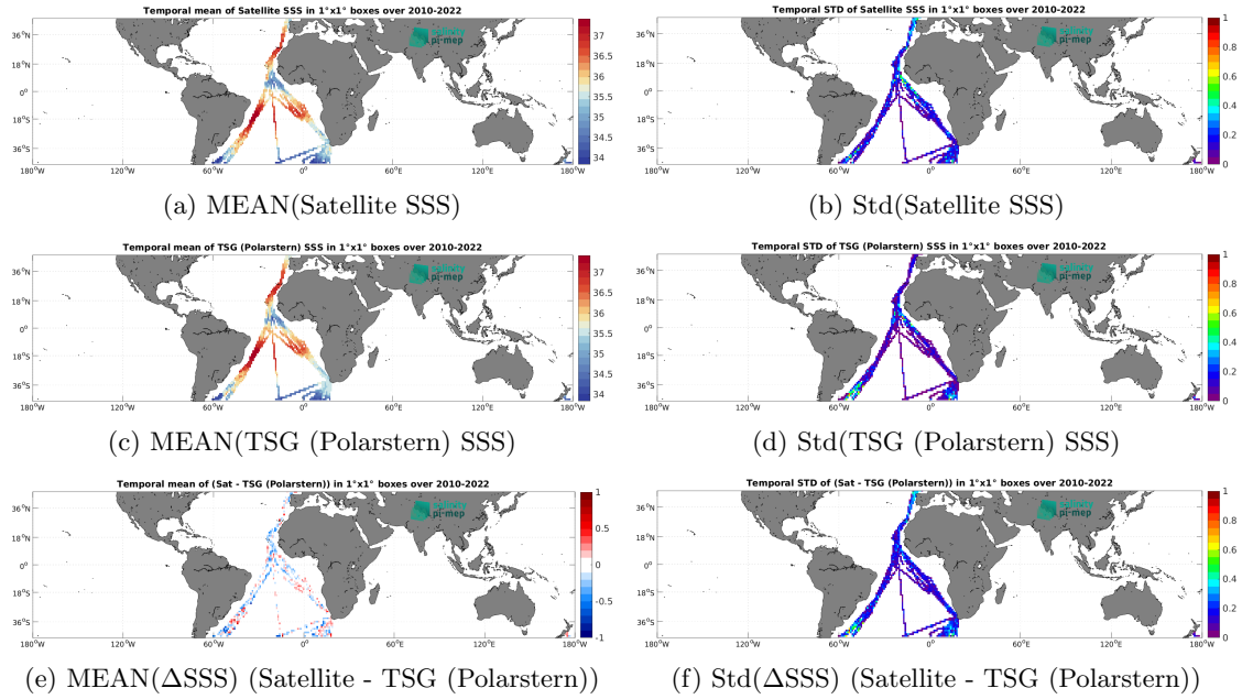
Figure 6: Temporal mean (left) and Std (right) of SSS from SMOS SSS L3 v8 - 9 Days (CATDS-CEC-LOCEAN) (top), TSG (Polarstern) (middle), and of \Delta SSS (Satellite - TSG (Polarstern)). Only match-up pairs are used to generate these maps.
