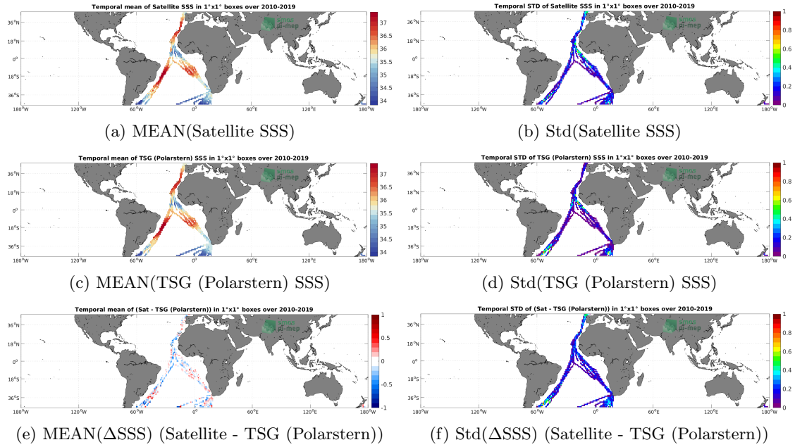
Figure 6: Temporal mean (left) and Std (right) of SSS from SMOS SSS L3 v8 - 9 Days (CATDS-CECOS-LOCEAN) (top), TSG (Polarstern) (middle), and of \Delta SSS (Satellite - TSG (Polarstern)). Only match-up pairs are used to generate these maps.
