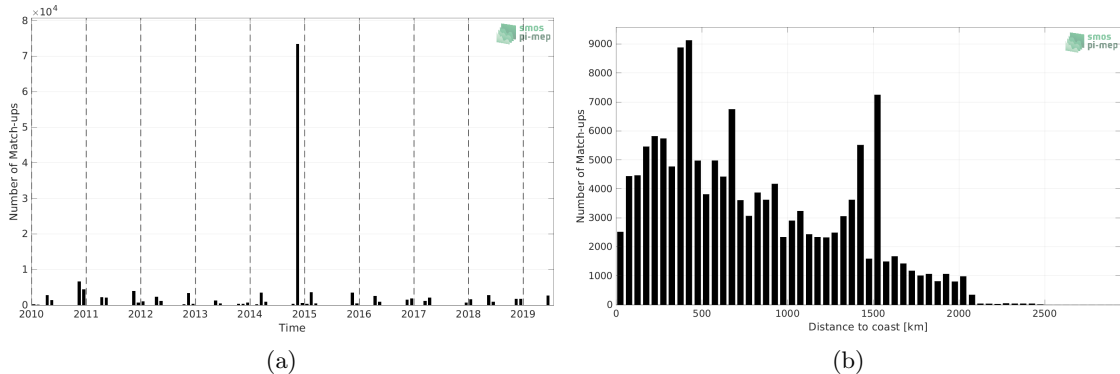
Figure 1: Number of match-ups between TSG (Polarstern) and SMOS SSS L3 v8 - 9 Days (CATDS-CECOS-LOCEAN) SSS as a function of time (a) and as function of the distance to coast (b) over the Mid-Low Latitudes 45N-45S Pi-MEP region and for the full satellite product period.
