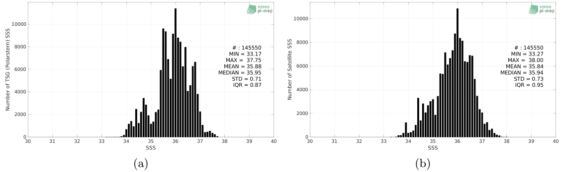
Figure 2: Histograms of SSS from TSG (Polarstern) (a) and SMOS SSS L3 v8 - 9 Days (CATDS-CECOS-LOCEAN) (b) considering all match-up pairs per bins of 0.1 over the Mid-Low Latitudes 45N-45S Pi-MEP region and for the full satellite product period.
