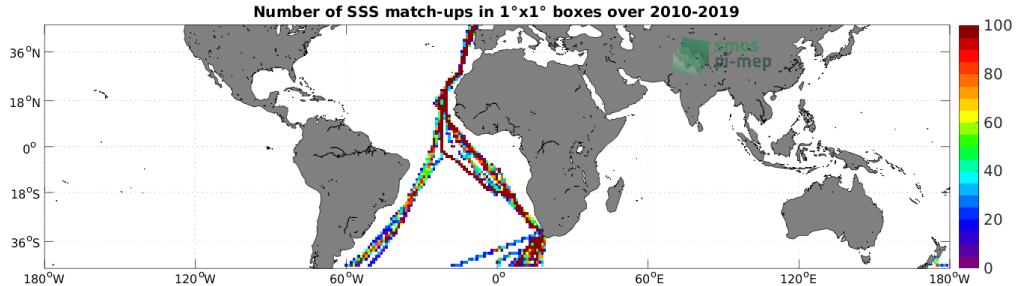
Figure 4: Number of SSS match-ups between TSG (Polarstern) SSS and the SMOS SSS L3 v8 - 9 Days (CATDS-CECOS-LOCEAN) SSS product for the Mid-Low Latitudes 45N-45S Pi-MEP region over 1^\circ \times 1^\circ boxes and for the full satellite product period.
