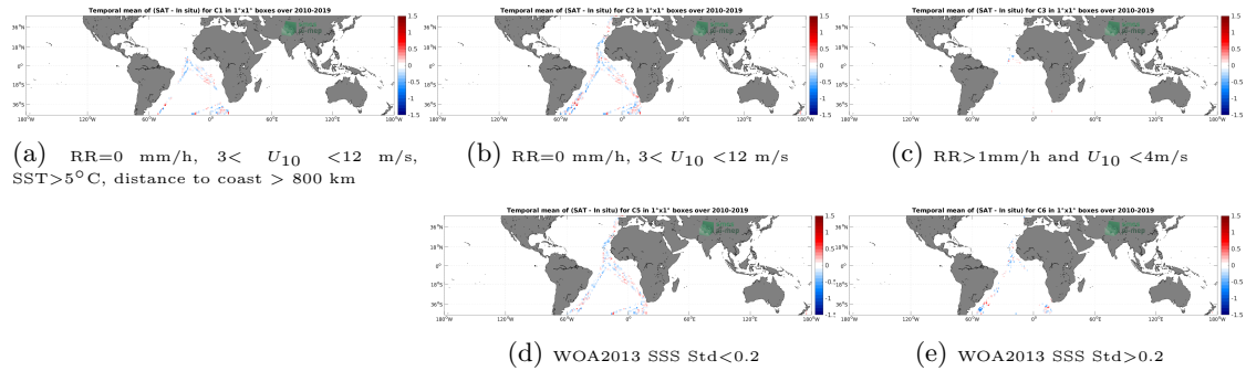
Figure 12: Temporal mean gridded over spatial boxes of size 1^\circ \times 1^\circ of \Delta SSS (SMOS SSS L3 v8 - 9 Days (CATDS-CECOS-LOCEAN) - TSG (Polarstern)) for 5 different subdatasets corresponding to:RR=0 mm/h, 3 < U_{10} < 12 m/s, SST >5^\circ C, distance to coast > 800 km (a), RR=0 mm/h, 3 < U_{10} < 12 m/s (b), RR >1 mm/h and U_{10} < 4 m/s (c), WOA2013 SSS Std <0.2 (d), WOA2013 SSS Std >0.2 (e).
