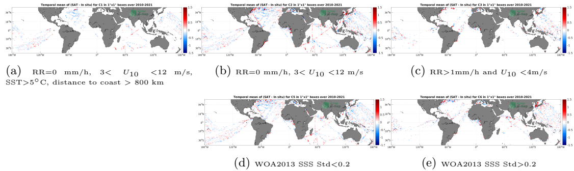
Figure 12: Temporal mean gridded over spatial boxes of size 1^\circ \times 1^\circ of \Delta SSS (SMOS SSS L3 v8 - 9 Days (CATDS-CECOS-LOCEAN) - TSG (LEGOS-DM)) for 5 different subdatasets corresponding to:RR=0 mm/h, 3 < U_{10} < 12 m/s, SST > 5^\circ\text{C} , distance to coast > 800 km (a), RR=0 mm/h, 3 < U_{10} < 12 m/s (b), RR > 1 mm/h and U_{10} < 4 m/s (c), WOA2013 SSS Std < 0.2 (d), WOA2013 SSS Std > 0.2 (e).
