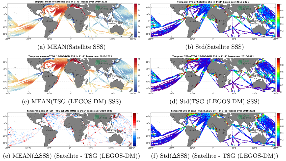
Figure 6: Temporal mean (left) and Std (right) of SSS from SMOS SSS L3 v8 - 9 Days (CATDS-CECOS-LOCEAN) (top), TSG (LEGOS-DM) (middle), and of \Delta SSS (Satellite - TSG (LEGOS-DM)). Only match-up pairs are used to generate these maps.
