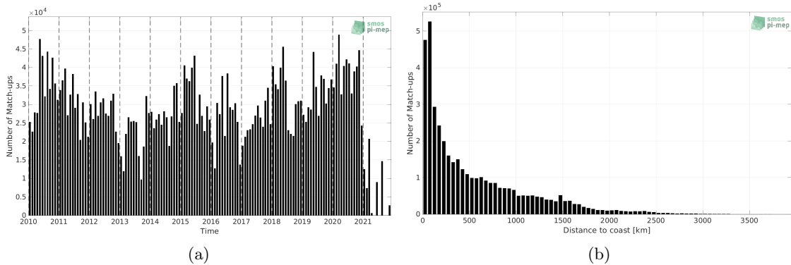
Figure 1: Number of match-ups between TSG (LEGOS-DM) and SMOS SSS L3 v8 - 9 Days (CATDS-CECOS-LOCEAN) SSS as a function of time (a) and as function of the distance to coast (b) over the Mid-Low Latitudes 45N-45S Pi-MEP region and for the full satellite product period.
