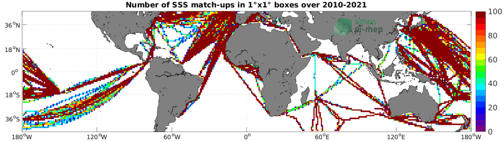
Figure 4: Number of SSS match-ups between TSG (LEGOS-DM) SSS and the SMOS SSS L3 v8 - 9 Days (CATDS-CECOS-LOCEAN) SSS product for the Mid-Low Latitudes 45N-45S Pi-MEP region over 1^{\circ} \times 1^{\circ} boxes and for the full satellite product period.
