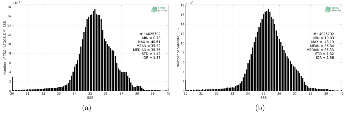
Figure 2: Histograms of SSS from TSG (LEGOS-DM) (a) and SMOS SSS L3 v8 - 9 Days (CATDS-CECOS-LOCEAN) (b) considering all match-up pairs per bins of 0.1 over the Mid-Low Latitudes 45N-45S Pi-MEP region and for the full satellite product period.
