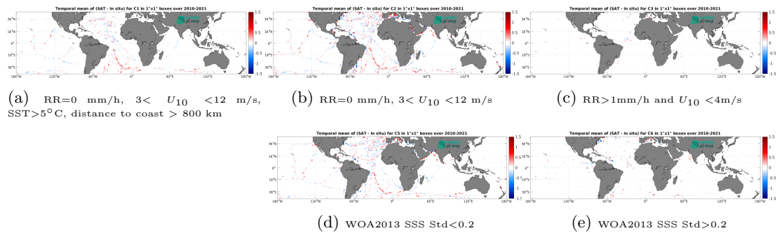
Figure 12: Temporal mean gridded over spatial boxes of size 1^\circ \times 1^\circ of \Delta SSS (SMOS SSS L3 v8 - 9 Days (CATDS-CEC-LOCEAN) - TSG (GOSUD-Sailing-ship)) for 5 different subdatasets corresponding to: RR=0 mm/h, 3 < U_{10} < 12 m/s, SST > 5°C, distance to coast > 800 km (a), RR=0 mm/h, 3 < U_{10} < 12 m/s (b), RR > 1mm/h and U_{10} < 4 m/s (c), WOA2013 SSS Std < 0.2 (d), WOA2013 SSS Std > 0.2 (e).
