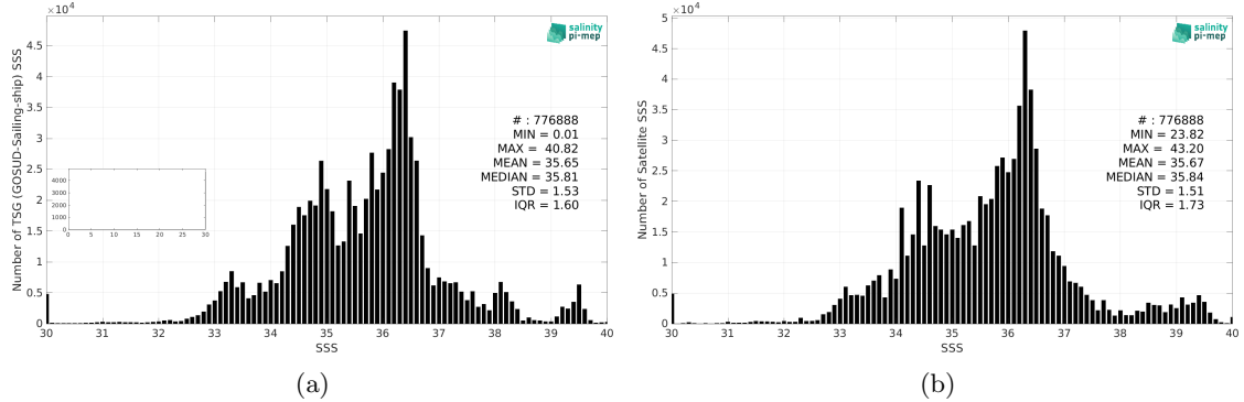
Figure 2: Histograms of SSS from TSG (GOSUD-Sailing-ship) (a) and SMOS SSS L3 v8 - 9 Days (CATDS-CEC-LOCEAN) (b) considering all match-up pairs per bins of 0.1 over the Mid-Low Latitudes 45N-45S Pi-MEP region and for the full satellite product period.
