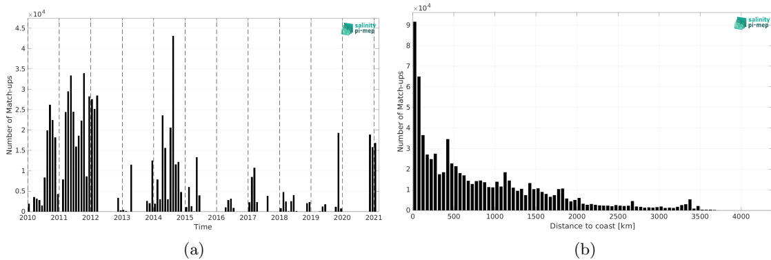
Figure 1: Number of match-ups between TSG (GOSUD-Sailing-ship) and SMOS SSS L3 v8 - 9 Days (CATDS-CEC-LOCEAN) SSS as a function of time (a) and as function of the distance to coast (b) over the Mid-Low Latitudes 45N-45S Pi-MEP region and for the full satellite product period.
