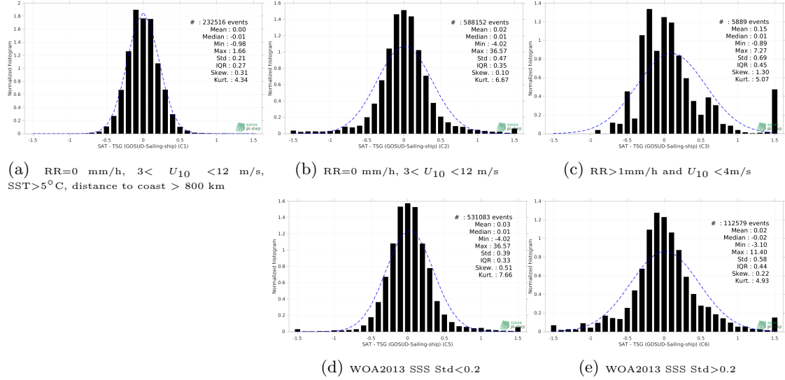
Figure 13: Normalized histogram of \Delta SSS (SMOS SSS L3 v8 - 9 Days (CATDS-CECOS-LOCEAN) - TSG (GOSUD-Sailing-ship)) for 5 different subdatasets corresponding to: RR=0 mm/h, 3 < U_{10} < 12 m/s, SST>5°C, distance to coast > 800 km (a), RR=0 mm/h, 3 < U_{10} < 12 m/s (b), RR>1mm/h and U_{10} < 4 m/s (c), WOA2013 SSS Std<0.2 (d), WOA2013 SSS Std>0.2 (e).
