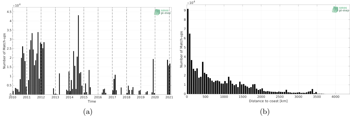
Figure 1: Number of match-ups between TSG (GOSUD-Sailing-ship) and SMOS SSS L3 v8 - 9 Days (CATDS-CECOS-LOCEAN) SSS as a function of time (a) and as function of the distance to coast (b) over the Mid-Low Latitudes 45N-45S Pi-MEP region and for the full satellite product period.
