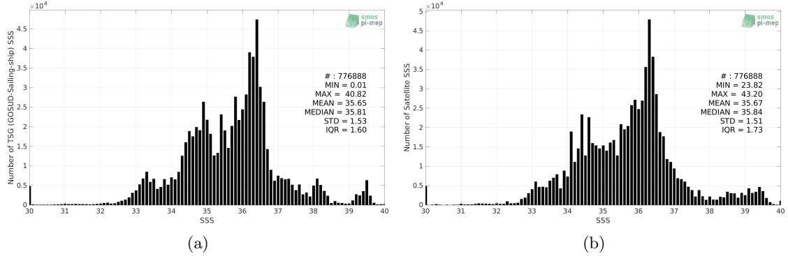
Figure 2: Histograms of SSS from TSG (GOSUD-Sailing-ship) (a) and SMOS SSS L3 v8 - 9 Days (CATDS-CECOS-LOCEAN) (b) considering all match-up pairs per bins of 0.1 over the Mid-Low Latitudes 45N-45S Pi-MEP region and for the full satellite product period.
