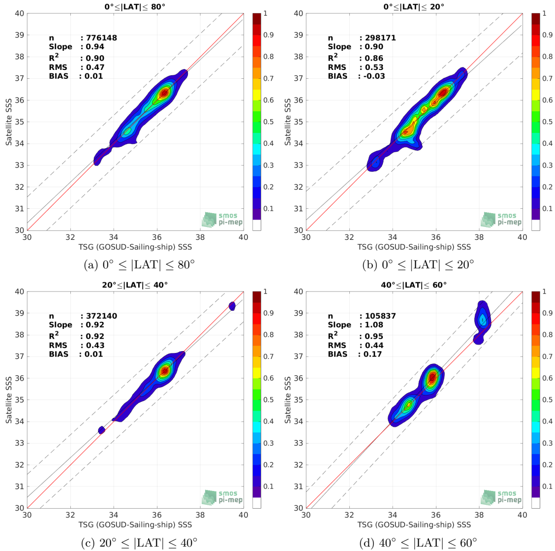
Figure 9: Contour maps of the concentration of SMOS SSS L3 v8 - 9 Days (CATDS-CECOS-LOCEAN) SSS (y-axis) versus TSG (GOSUD-Sailing-ship) SSS (x-axis) at match-up pairs for different latitude bands. For each plot, the red line shows x=y . The black thin and dashed lines indicate a linear fit through the data cloud and the \pm 95\% confidence levels, respectively. The number match-up pairs n , the slope and R^2 coefficient of the linear fit, the root mean square (RMS) and the mean bias between satellite and in situ data are indicated for each latitude band in each plots.
