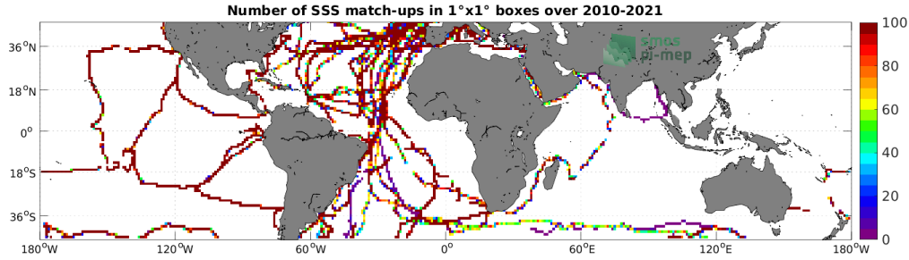
Figure 4: Number of SSS match-ups between TSG (GOSUD-Sailing-ship) SSS and the SMOS SSS L3 v8 - 9 Days (CATDS-CECOS-LOCEAN) SSS product for the Mid-Low Latitudes 45N-45S Pi-MEP region over 1^\circ \times 1^\circ boxes and for the full satellite product period.
