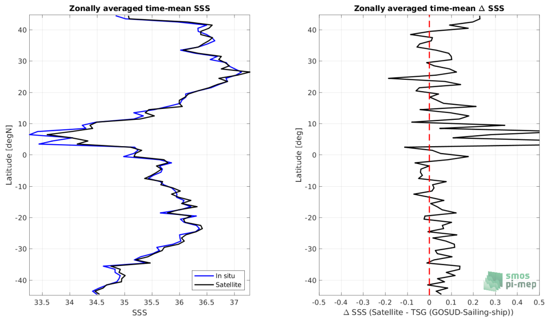
Figure 8: Left panel: Zonal mean SSS from SMOS SSS L3 v8 - 9 Days (CATDS-CECOS-LOCEAN) satellite product (black) and from TSG (GOSUD-Sailing-ship) (blue). Right panel: Zonal mean of \Delta SSS (Satellite - TSG (GOSUD-Sailing-ship)) for all the collected Pi-MEP match-up pairs estimated over the full satellite product period.
