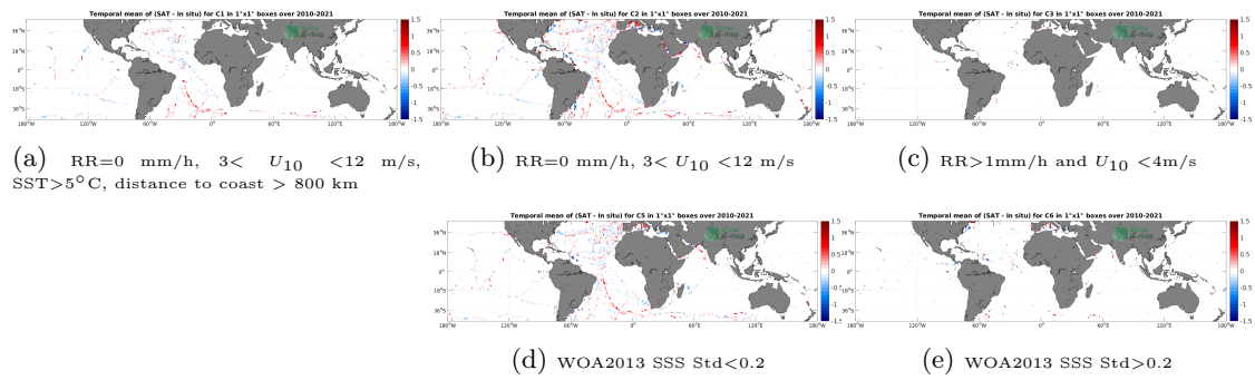
Figure 12: Temporal mean gridded over spatial boxes of size 1^\circ \times 1^\circ of \Delta\text{SSS} (SMOS SSS L3 v8 - 9 Days (CATDS-CECOS-LOCEAN) - TSG (GOSUD-Sailing-ship)) for 5 different subdatasets corresponding to: RR=0 mm/h, 3 < U_{10} < 12 m/s, SST > 5°C, distance to coast > 800 km (a), RR=0 mm/h, 3 < U_{10} < 12 m/s (b), RR > 1mm/h and U_{10} < 4 m/s (c), WOA2013 SSS Std < 0.2 (d), WOA2013 SSS Std > 0.2 (e).
