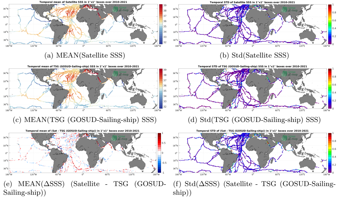
Figure 6: Temporal mean (left) and Std (right) of SSS from SMOS SSS L3 v8 - 9 Days (CATDS-CECOS-LOCEAN) (top), TSG (GOSUD-Sailing-ship) (middle), and of \Delta SSS (Satellite - TSG (GOSUD-Sailing-ship)). Only match-up pairs are used to generate these maps.
