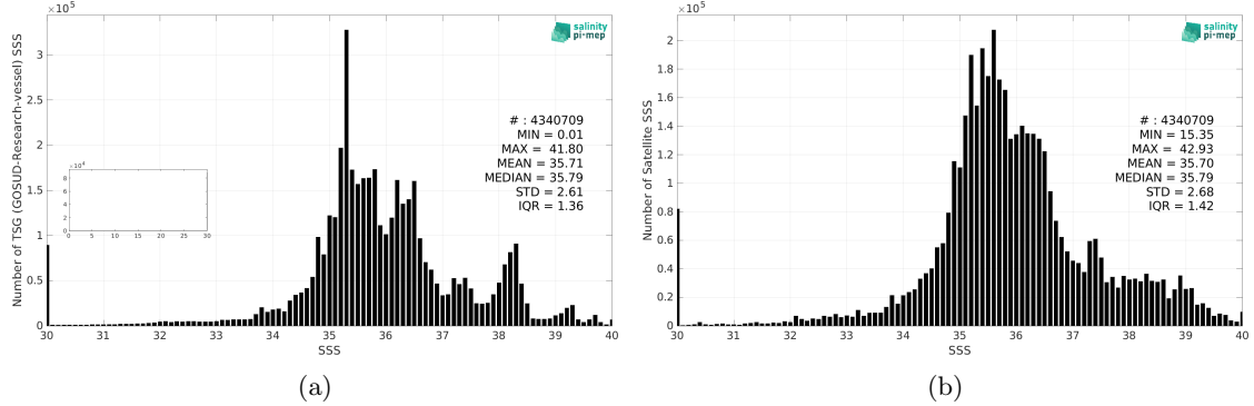
Figure 2: Histograms of SSS from TSG (GOSUD-Research-vessel) (a) and SMOS SSS L3 v8 - 9 Days (CATDS-CEC-LOCEAN) (b) considering all match-up pairs per bins of 0.1 over the Mid-Low Latitudes 45N-45S Pi-MEP region and for the full satellite product period.
