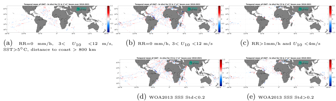
Figure 12: Temporal mean gridded over spatial boxes of size 1^\circ \times 1^\circ of \Delta\text{SSS} (SMOS SSS L3 v8 - 9 Days (CATDS-CEC-LOCEAN) - TSG (GOSUD-Research-vessel)) for 5 different subdatasets corresponding to:RR=0 mm/h, 3 < U_{10} < 12 m/s, SST>5°C, distance to coast > 800 km (a), RR=0 mm/h, 3 < U_{10} < 12 m/s (b), RR>1mm/h and U_{10} < 4 m/s (c), WOA2013 SSS Std<0.2 (d), WOA2013 SSS Std>0.2 (e).
