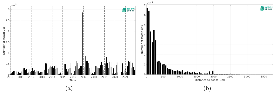
Figure 1: Number of match-ups between TSG (GOSUD-Research-vessel) and SMOS SSS L3 v8 - 9 Days (CATDS-CEC-LOCEAN) SSS as a function of time (a) and as function of the distance to coast (b) over the Mid-Low Latitudes 45N-45S Pi-MEP region and for the full satellite product period.
