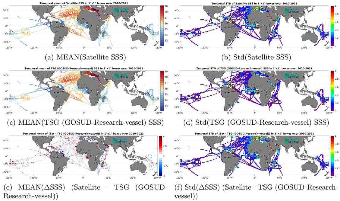
Figure 6: Temporal mean (left) and Std (right) of SSS from SMOS SSS L3 v8 - 9 Days (CATDS-CEC-LOCEAN) (top), TSG (GOSUD-Research-vessel) (middle), and of \Delta SSS (Satellite - TSG (GOSUD-Research-vessel)). Only match-up pairs are used to generate these maps.
