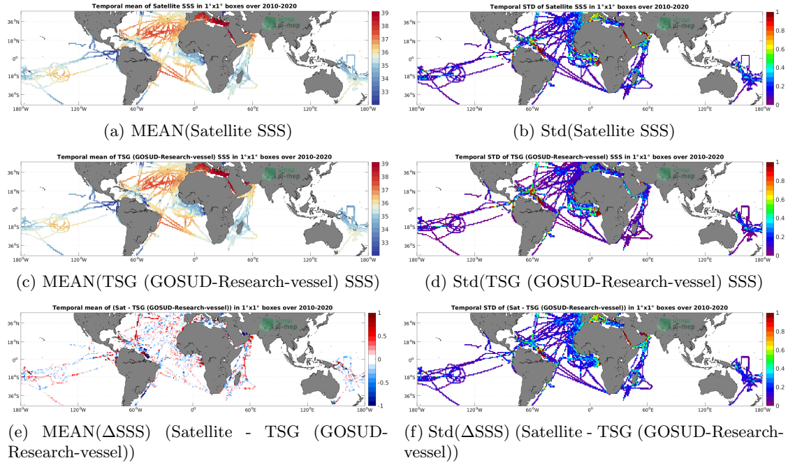
Figure 6: Temporal mean (left) and Std (right) of SSS from SMOS SSS L3 v8 - 9 Days (CATDS-CECOS-LOCEAN) (top), TSG (GOSUD-Research-vessel) (middle), and of \Delta SSS (Satellite - TSG (GOSUD-Research-vessel)). Only match-up pairs are used to generate these maps.
