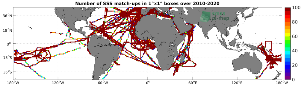
Figure 4: Number of SSS match-ups between TSG (GOSUD-Research-vessel) SSS and the SMOS SSS L3 v8 - 9 Days (CATDS-CECOS-LOCEAN) SSS product for the Mid-Low Latitudes 45N-45S Pi-MEP region over 1^\circ \times 1^\circ boxes and for the full satellite product period.
