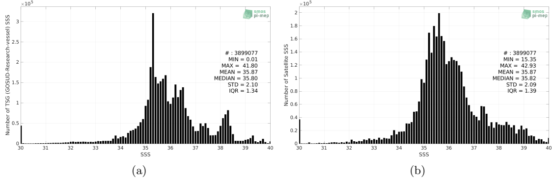
Figure 2: Histograms of SSS from TSG (GOSUD-Research-vessel) (a) and SMOS SSS L3 v8 - 9 Days (CATDS-CECOS-LOCEAN) (b) considering all match-up pairs per bins of 0.1 over the Mid-Low Latitudes 45N-45S Pi-MEP region and for the full satellite product period.
