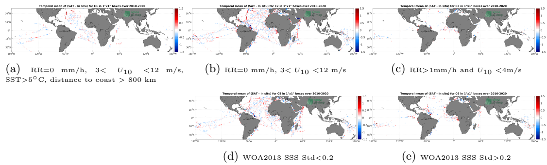
Figure 12: Temporal mean gridded over spatial boxes of size 1^\circ \times 1^\circ of \Delta SSS (SMOS SSS L3 v8 - 9 Days (CATDS-CECOS-LOCEAN) - TSG (GOSUD-Research-vessel)) for 5 different subdatasets corresponding to:RR=0 mm/h, 3 < U_{10} < 12 m/s, SST >5^\circ C, distance to coast > 800 km (a), RR=0 mm/h, 3 < U_{10} < 12 m/s (b), RR >1 mm/h and U_{10} < 4 m/s (c), WOA2013 SSS Std <0.2 (d), WOA2013 SSS Std >0.2 (e).
