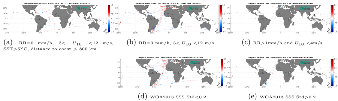
Figure 12: Temporal mean gridded over spatial boxes of size 1^\circ \times 1^\circ of \Delta SSS (SMOS SSS L3 v8 - 9 Days (CATDS-CEC-LOCEAN) - TSG (CSIC-UTM)) for 5 different subdatasets corresponding to:RR=0 mm/h, 3 < U_{10} < 12 m/s, SST >5^\circ\text{C} , distance to coast > 800 km (a), RR=0 mm/h, 3 < U_{10} < 12 m/s (b), RR >1 mm/h and U_{10} < 4 m/s (c), WOA2013 SSS Std <0.2 (d), WOA2013 SSS Std >0.2 (e).
