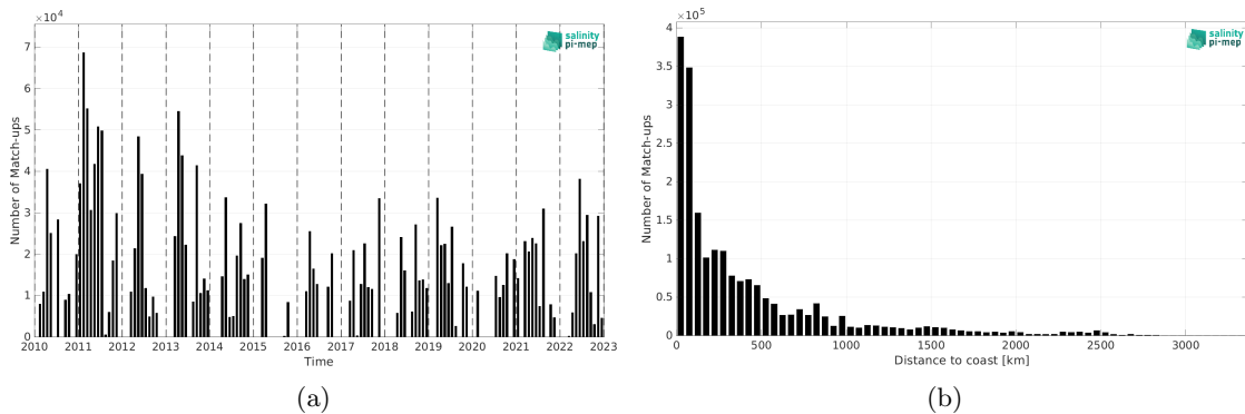
Figure 1: Number of match-ups between TSG (CSIC-UTM) and SMOS SSS L3 v8 - 9 Days (CATDS-CEC-LOCEAN) SSS as a function of time (a) and as function of the distance to coast (b) over the Mid-Low Latitudes 45N-45S Pi-MEP region and for the full satellite product period.
