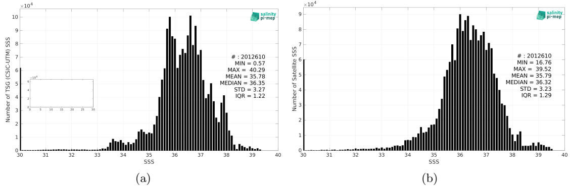
Figure 2: Histograms of SSS from TSG (CSIC-UTM) (a) and SMOS SSS L3 v8 - 9 Days (CATDS-CEC-LOCEAN) (b) considering all match-up pairs per bins of 0.1 over the Mid-Low Latitudes 45N-45S Pi-MEP region and for the full satellite product period.
