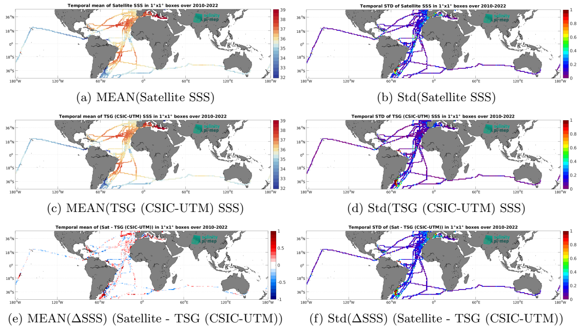
Figure 6: Temporal mean (left) and Std (right) of SSS from SMOS SSS L3 v8 - 9 Days (CATDS-CEC-LOCEAN) (top), TSG (CSIC-UTM) (middle), and of \Delta SSS (Satellite - TSG (CSIC-UTM)). Only match-up pairs are used to generate these maps.
