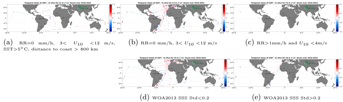
Figure 12: Temporal mean gridded over spatial boxes of size 1^\circ \times 1^\circ of \Delta SSS (SMOS SSS L3 v8 - 9 Days (CATDS-CECOS-LOCEAN) - TSG (CSIC-UTM)) for 5 different subdatasets corresponding to:RR=0 mm/h, 3 < U_{10} < 12 m/s, SST >5^\circ C, distance to coast > 800 km (a), RR=0 mm/h, 3 < U_{10} < 12 m/s (b), RR >1 mm/h and U_{10} < 4 m/s (c), WOA2013 SSS Std <0.2 (d), WOA2013 SSS Std >0.2 (e).
