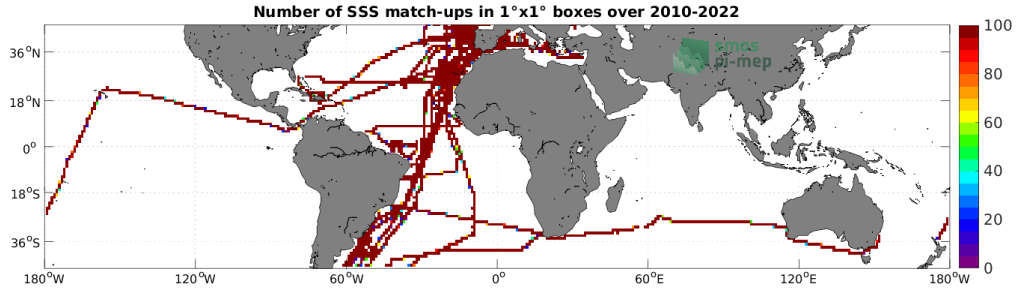
Figure 4: Number of SSS match-ups between TSG (CSIC-UTM) SSS and the SMOS SSS L3 v8 - 9 Days (CATDS-CECOS-LOCEAN) SSS product for the Mid-Low Latitudes 45N-45S Pi-MEP region over 1^\circ \times 1^\circ boxes and for the full satellite product period.
