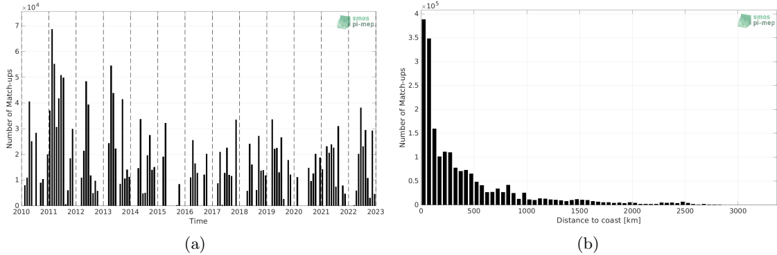
Figure 1: Number of match-ups between TSG (CSIC-UTM) and SMOS SSS L3 v8 - 9 Days (CATDS-CECOS-LOCEAN) SSS as a function of time (a) and as function of the distance to coast (b) over the Mid-Low Latitudes 45N-45S Pi-MEP region and for the full satellite product period.
