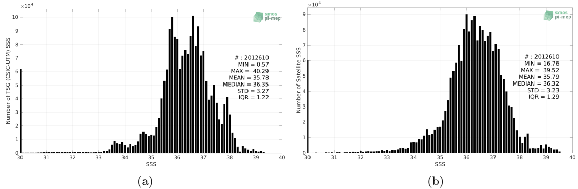
Figure 2: Histograms of SSS from TSG (CSIC-UTM) (a) and SMOS SSS L3 v8 - 9 Days (CATDS-CECOS-LOCEAN) (b) considering all match-up pairs per bins of 0.1 over the Mid-Low Latitudes 45N-45S Pi-MEP region and for the full satellite product period.
