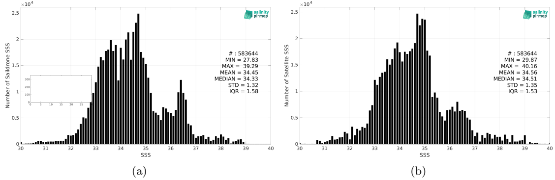
Figure 2: Histograms of SSS from Saildrone (a) and SMOS SSS L3 v8 - 9 Days (CATDS-CEC-LOCEAN) (b) considering all match-up pairs per bins of 0.1 over the Mid-Low Latitudes 45N-45S Pi-MEP region and for the full satellite product period.
