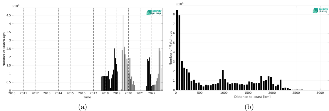
Figure 1: Number of match-ups between Saildrone and SMOS SSS L3 v8 - 9 Days (CATDS-CEC-LOCEAN) SSS as a function of time (a) and as function of the distance to coast (b) over the Mid-Low Latitudes 45N-45S Pi-MEP region and for the full satellite product period.
