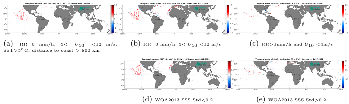
Figure 12: Temporal mean gridded over spatial boxes of size 1^\circ \times 1^\circ of \Delta SSS (SMOS SSS L3 v8 - 9 Days (CATDS-CEC-LOCEAN) - Saifdrone) for 5 different subdatasets corresponding to:RR=0 mm/h, 3 < U_{10} < 12 m/s, SST >5^\circ C, distance to coast > 800 km (a), RR=0 mm/h, 3 < U_{10} < 12 m/s (b), RR >1 mm/h and U_{10} < 4 m/s (c), WOA2013 SSS Std <0.2 (d), WOA2013 SSS Std >0.2 (e).
