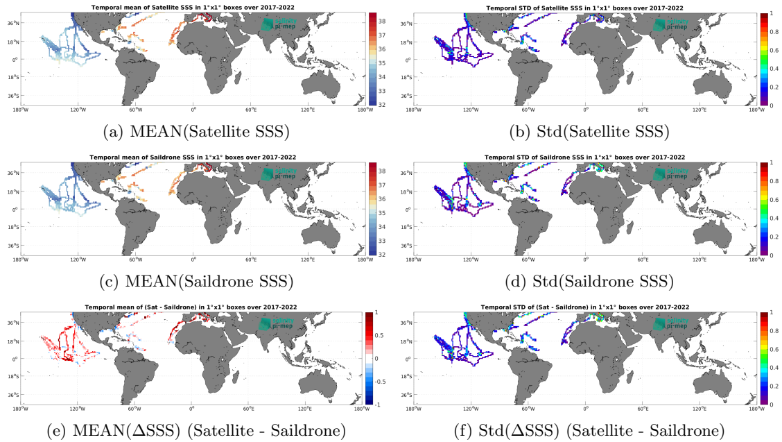
Figure 6: Temporal mean (left) and Std (right) of SSS from SMOS SSS L3 v8 - 9 Days (CATDS-CEC-LOCEAN) (top), Saildrone (middle), and of \Delta SSS (Satellite - Saildrone). Only match-up pairs are used to generate these maps.
