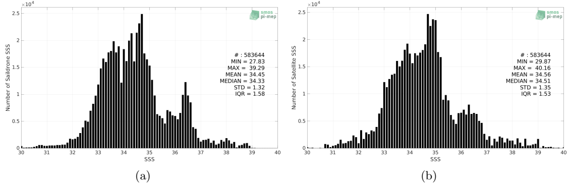
Figure 2: Histograms of SSS from Saildrone (a) and SMOS SSS L3 v8 - 9 Days (CATDS-CECOS-LOCEAN) (b) considering all match-up pairs per bins of 0.1 over the Mid-Low Latitudes 45N-45S Pi-MEP region and for the full satellite product period.
