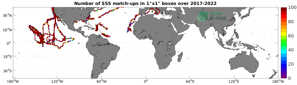
Figure 4: Number of SSS match-ups between Saildrone SSS and the SMOS SSS L3 v8 - 9 Days (CATDS-CECOS-LOCEAN) SSS product for the Mid-Low Latitudes 45N-45S Pi-MEP region over 1^\circ \times 1^\circ boxes and for the full satellite product period.
