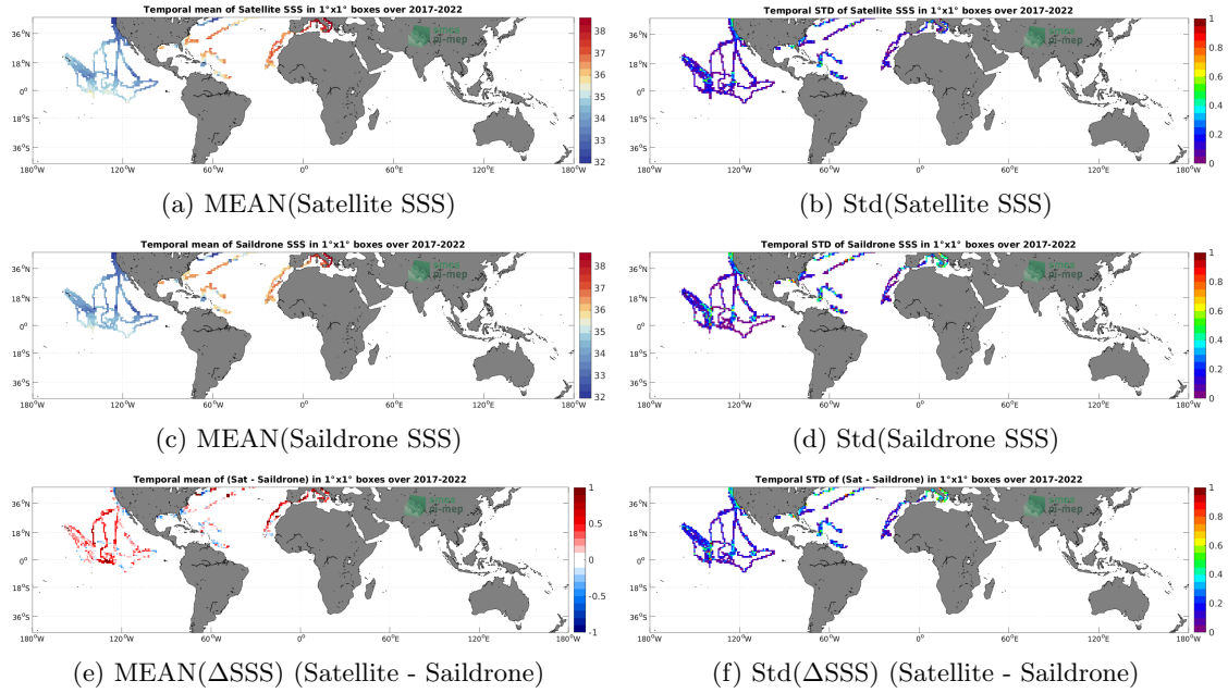
Figure 6: Temporal mean (left) and Std (right) of SSS from SMOS SSS L3 v8 - 9 Days (CATDS-CECOS-LOCEAN) (top), Saildrone (middle), and of \Delta SSS (Satellite - Saildrone). Only match-up pairs are used to generate these maps.
