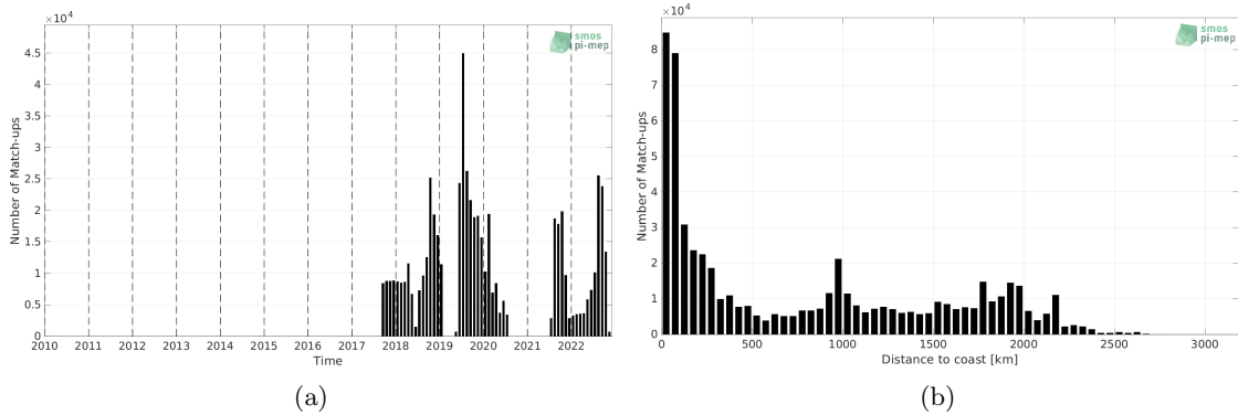
Figure 1: Number of match-ups between Saildrone and SMOS SSS L3 v8 - 9 Days (CATDS-CECOS-LOCEAN) SSS as a function of time (a) and as function of the distance to coast (b) over the Mid-Low Latitudes 45N-45S Pi-MEP region and for the full satellite product period.
