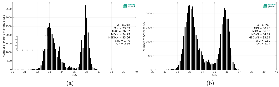
Figure 2: Histograms of SSS from Marine mammals (a) and SMOS SSS L3 v8 - 9 Days (CATDS-CEC-LOCEAN) (b) considering all match-up pairs per bins of 0.1 over the Mid-Low Latitudes 45N-45S Pi-MEP region and for the full satellite product period.
