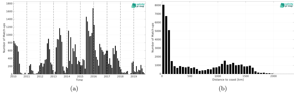
Figure 1: Number of match-ups between Marine mammals and SMOS SSS L3 v8 - 9 Days (CATDS-CEC-LOCEAN) SSS as a function of time (a) and as function of the distance to coast (b) over the Mid-Low Latitudes 45N-45S Pi-MEP region and for the full satellite product period.
