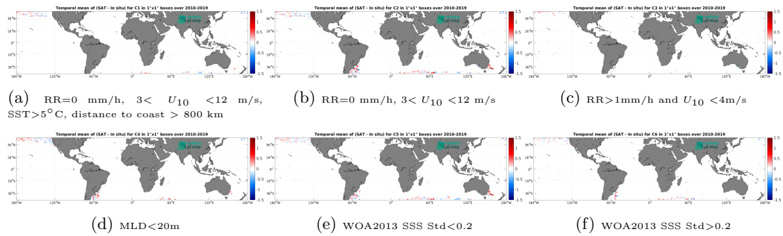
Figure 12: Temporal mean gridded over spatial boxes of size 1^{\circ}\times 1^{\circ} of \Delta\text{SSS} (SMOS SSS L3 v8 - 9 Days (CATDS-CEC-LOCEAN) - Marine mammals) for 6 different subdatasets corresponding to: \text{RR}=0 mm/h, 3 < U_{10} < 12 m/s, \text{SST} > 5^{\circ}\text{C} , distance to coast > 800 km (a), \text{RR}=0 mm/h, 3 < U_{10} < 12 m/s (b), \text{RR} > 1\text{mm/h} and U_{10} < 4\text{m/s} (c), \text{MLD} < 20\text{m} (d), WOA2013 SSS Std < 0.2 (e), WOA2013 SSS Std > 0.2 (f).
