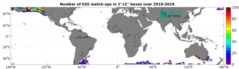
Figure 4: Number of SSS match-ups between Marine mammals SSS and the SMOS SSS L3 v8 - 9 Days (CATDS-CEC-LOCEAN) SSS product for the Mid-Low Latitudes 45N-45S Pi-MEP region over 1^\circ \times 1^\circ boxes and for the full satellite product period.
