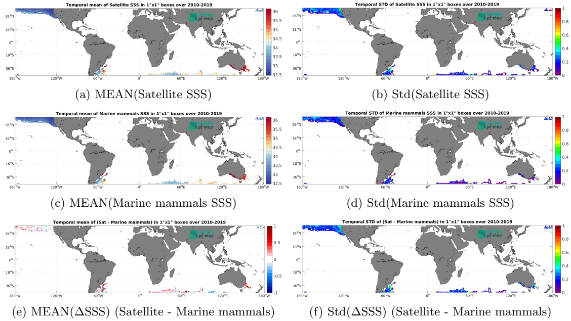
Figure 6: Temporal mean (left) and Std (right) of SSS from SMOS SSS L3 v8 - 9 Days (CATDS-CEC-LOCEAN) (top), Marine mammals (middle), and of \Delta SSS (Satellite - Marine mammals). Only match-up pairs are used to generate these maps.
