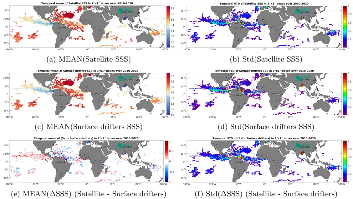
Figure 5: Temporal mean (left) and Std (right) of SSS from SMOS SSS L3 v8 - 9 Days (CATDS-CEC-LOCEAN) (top), Surface drifters (middle), and of \Delta SSS (Satellite - Surface drifters). Only match-up pairs are used to generate these maps.
