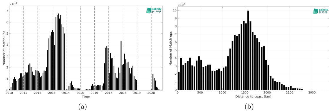
Figure 1: Number of match-ups between Surface drifters and SMOS SSS L3 v8 - 9 Days (CATDS-CEC-LOCEAN) SSS as a function of time (a) and as function of the distance to coast (b) over the Mid-Low Latitudes 45N-45S Pi-MEP region and for the full satellite product period.
