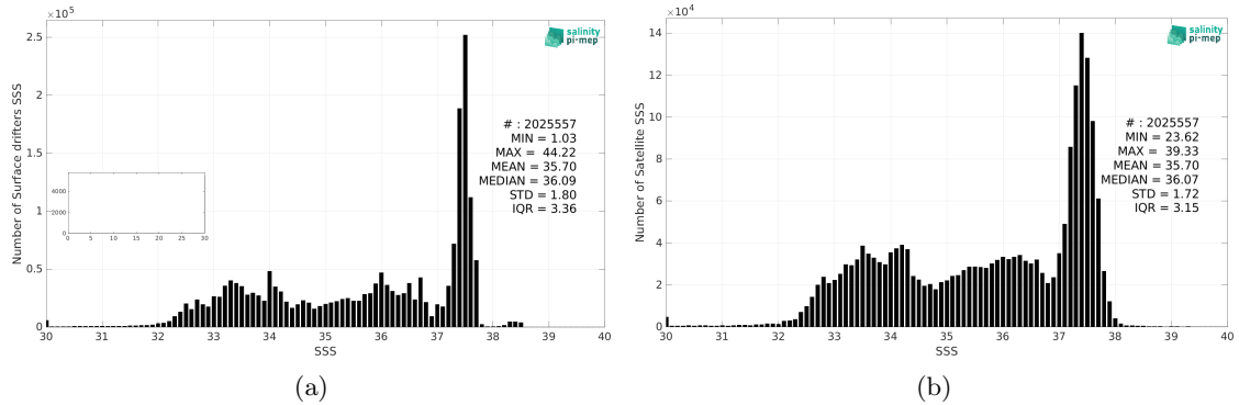
Figure 2: Histograms of SSS from Surface drifters (a) and SMOS SSS L3 v8 - 9 Days (CATDS-CEC-LOCEAN) (b) considering all match-up pairs per bins of 0.1 over the Mid-Low Latitudes 45N-45S Pi-MEP region and for the full satellite product period.
