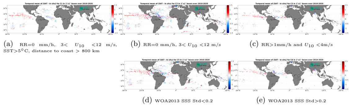
Figure 11: Temporal mean gridded over spatial boxes of size 1^\circ \times 1^\circ of \Delta\text{SSS} (SMOS SSS L3 v8 - 9 Days (CATDS-CEC-LOCEAN) - Surface drifters) for 5 different subdatasets corresponding to:RR=0 mm/h, 3 < U_{10} < 12 m/s, SST >5^\circ\text{C} , distance to coast > 800 km (a), RR=0 mm/h, 3 < U_{10} < 12 m/s (b), RR >1 mm/h and U_{10} < 4 m/s (c), WOA2013 SSS Std <0.2 (d), WOA2013 SSS Std >0.2 (e).
