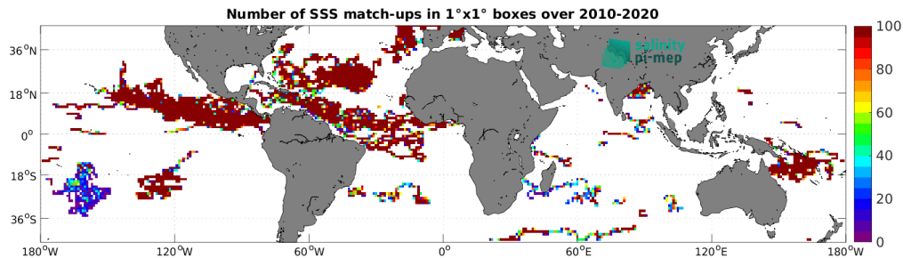
Figure 3: Number of SSS match-ups between Surface drifters SSS and the SMOS SSS L3 v8 - 9 Days (CATDS-CEC-LOCEAN) SSS product for the Mid-Low Latitudes 45N-45S Pi-MEP region over 1^\circ \times 1^\circ boxes and for the full satellite product period.
