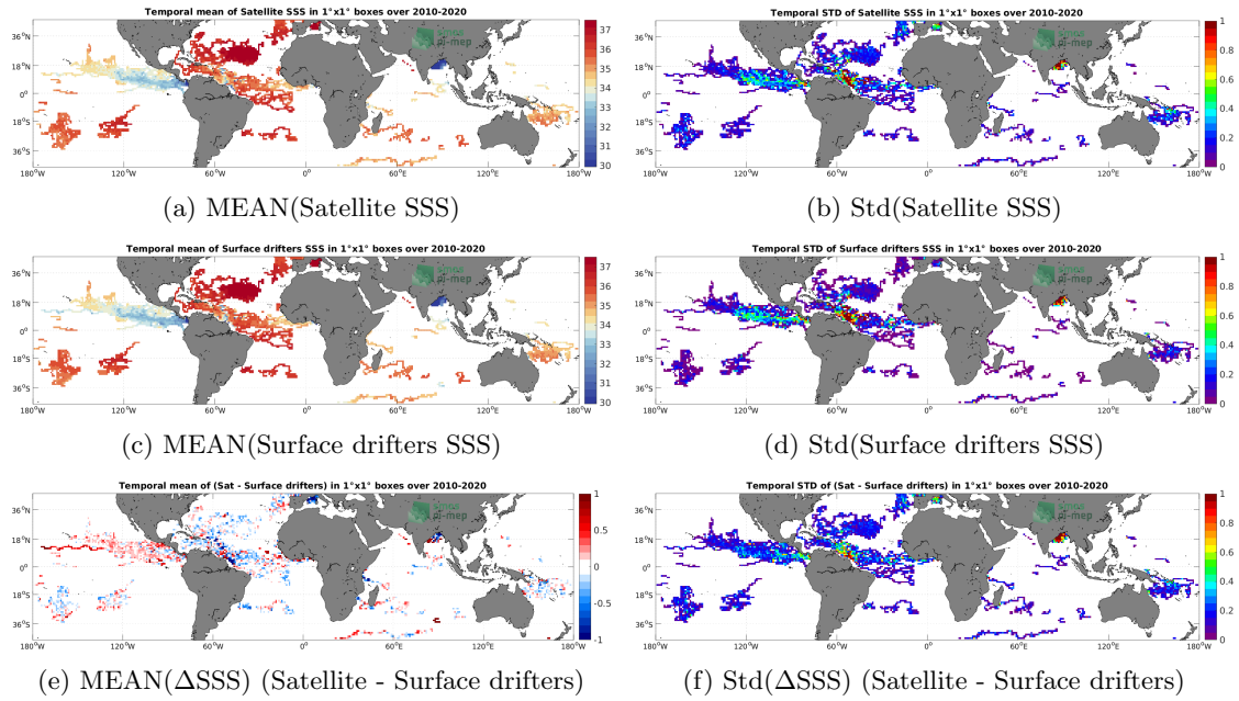
Figure 5: Temporal mean (left) and Std (right) of SSS from SMOS SSS L3 v8 - 9 Days (CATDS-CECOS-LOCEAN) (top), Surface drifters (middle), and of \Delta SSS (Satellite - Surface drifters). Only match-up pairs are used to generate these maps.
