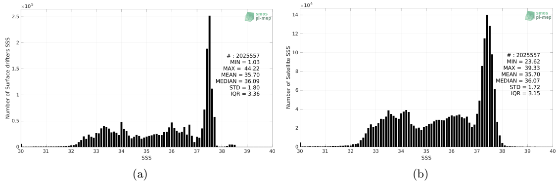
Figure 2: Histograms of SSS from Surface drifters (a) and SMOS SSS L3 v8 - 9 Days (CATDS-CECOS-LOCEAN) (b) considering all match-up pairs per bins of 0.1 over the Mid-Low Latitudes 45N-45S Pi-MEP region and for the full satellite product period.
