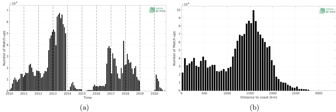
Figure 1: Number of match-ups between Surface drifters and SMOS SSS L3 v8 - 9 Days (CATDS-CECOS-LOCEAN) SSS as a function of time (a) and as function of the distance to coast (b) over the Mid-Low Latitudes 45N-45S Pi-MEP region and for the full satellite product period.
