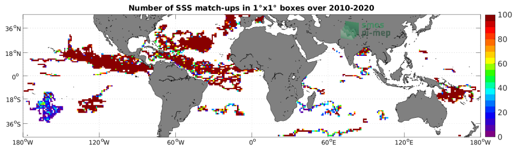
Figure 3: Number of SSS match-ups between Surface drifters SSS and the SMOS SSS L3 v8 - 9 Days (CATDS-CECOS-LOCEAN) SSS product for the Mid-Low Latitudes 45N-45S Pi-MEP region over 1^\circ \times 1^\circ boxes and for the full satellite product period.
