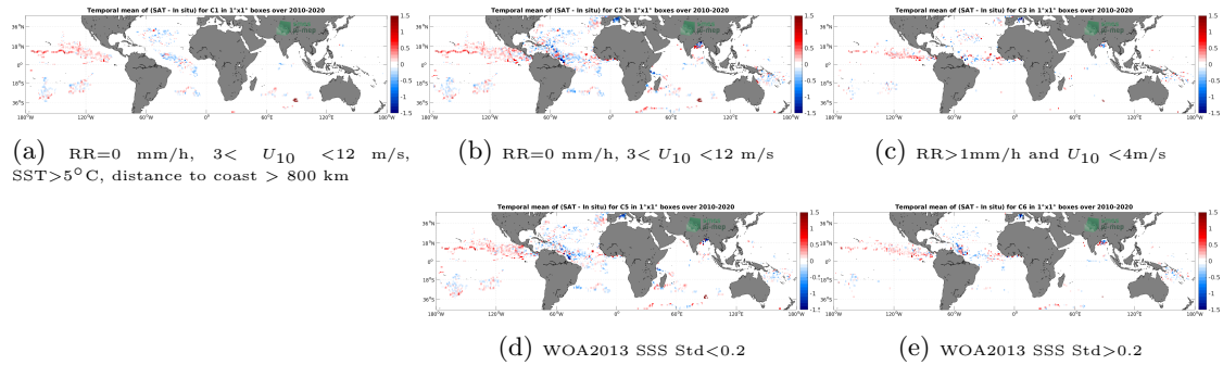
Figure 11: Temporal mean gridded over spatial boxes of size 1^\circ \times 1^\circ of \Delta SSS (SMOS SSS L3 v8 - 9 Days (CATDS-CECOS-LOCEAN) - Surface drifters) for 5 different subdatasets corresponding to:RR=0 mm/h, 3 < U_{10} < 12 m/s, SST >5^\circ C, distance to coast > 800 km (a), RR=0 mm/h, 3 < U_{10} < 12 m/s (b), RR >1 mm/h and U_{10} < 4 m/s (c), WOA2013 SSS Std <0.2 (d), WOA2013 SSS Std >0.2 (e).
