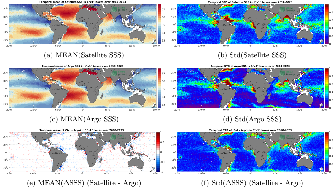
Figure 6: Temporal mean (left) and Std (right) of SSS from SMOS SSS L3 v8 - 9 Days (CATDS-CECOS-LOCEAN) (top), Argo (middle), and of \Delta SSS (Satellite - Argo). Only match-up pairs are used to generate these maps.
