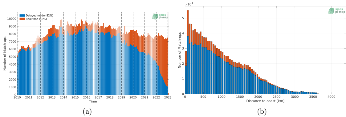
Figure 1: Number of match-ups between Argo and SMOS SSS L3 v8 - 9 Days (CATDS-CECOS-LOCEAN) SSS as a function of time (a) and as function of the distance to coast (b) over the Mid-Low Latitudes 45N-45S Pi-MEP region and for the full satellite product period.
