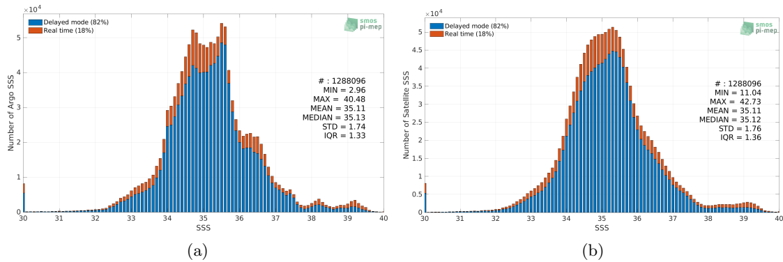
Figure 2: Histograms of SSS from Argo (a) and SMOS SSS L3 v8 - 9 Days (CATDS-CECOS-LOCEAN) (b) considering all match-up pairs per bins of 0.1 over the Mid-Low Latitudes 45N-45S Pi-MEP region and for the full satellite product period.
