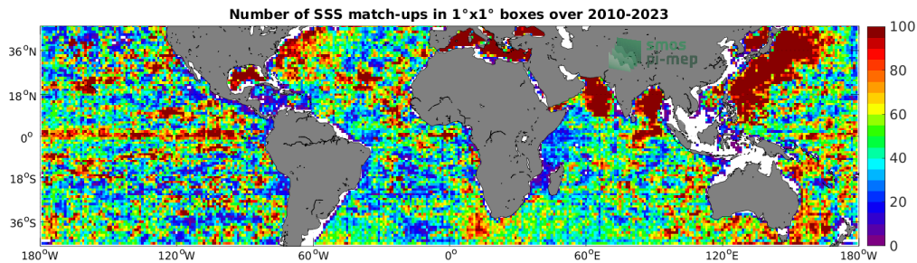
Figure 4: Number of SSS match-ups between Argo SSS and the SMOS SSS L3 v8 - 9 Days (CATDS-CECOS-LOCEAN) SSS product for the Mid-Low Latitudes 45N-45S Pi-MEP region over 1^\circ \times 1^\circ boxes and for the full satellite product period.
