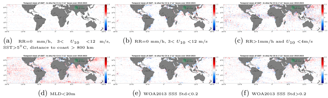
Figure 12: Temporal mean gridded over spatial boxes of size 1^\circ \times 1^\circ of \Delta SSS (SMOS SSS L3 v8 - 9 Days (CATDS-CECOS-LOCEAN) - Argo) for 6 different subdatasets corresponding to:RR=0 mm/h, 3 < U_{10} < 12 m/s, SST >5^\circ C, distance to coast > 800 km (a), RR=0 mm/h, 3 < U_{10} < 12 m/s (b), RR >1 mm/h and U_{10} < 4 m/s (c),MLD <20 m (d),WOA2013 SSS Std <0.2 (e),WOA2013 SSS Std >0.2 (f).
