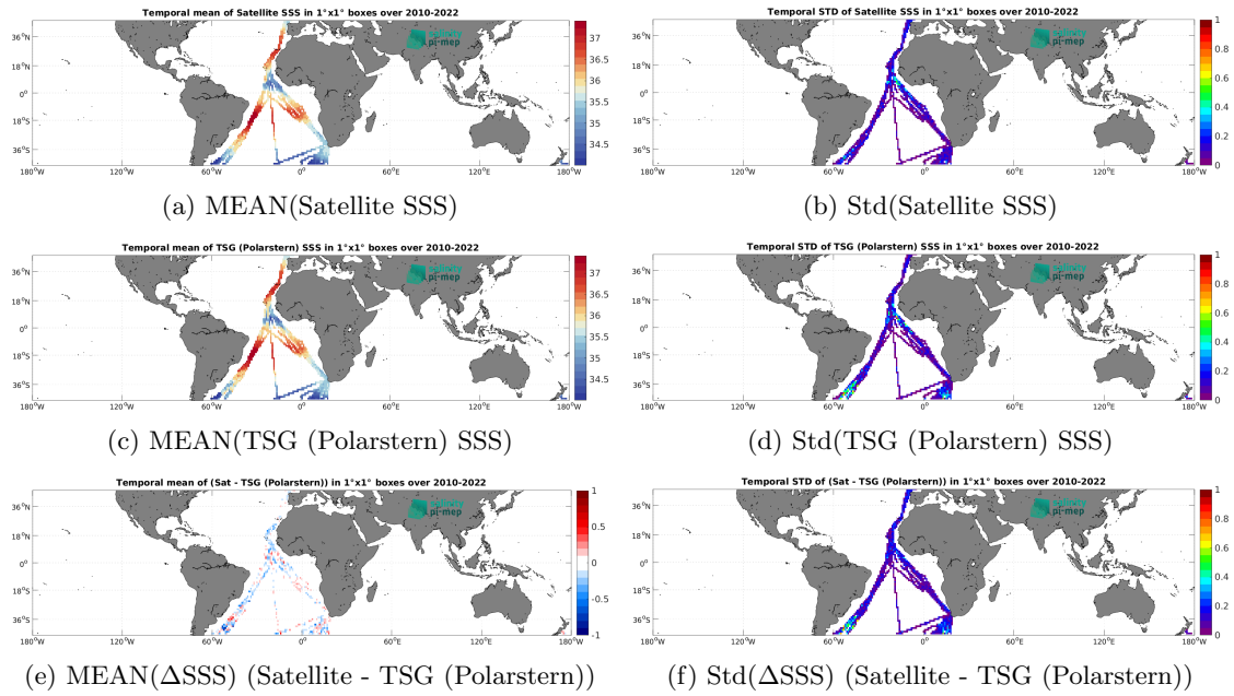
Figure 6: Temporal mean (left) and Std (right) of SSS from SMOS SSS L3 v8 - 18 Days (CATDS-CEC-LOCEAN) (top), TSG (Polarstern) (middle), and of \Delta SSS (Satellite - TSG (Polarstern)). Only match-up pairs are used to generate these maps.
