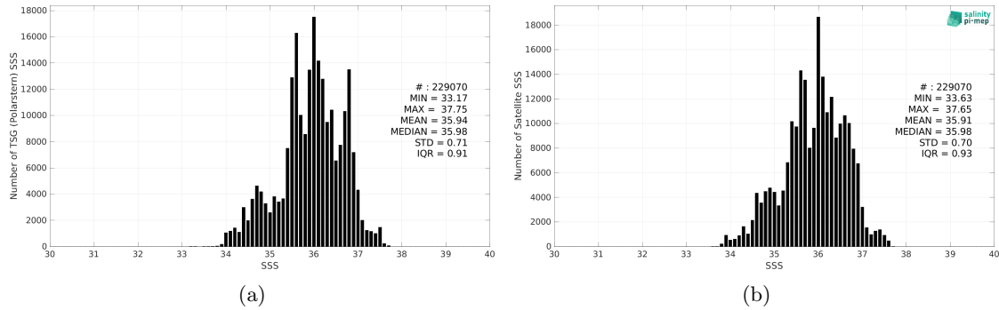
Figure 2: Histograms of SSS from TSG (Polarstern) (a) and SMOS SSS L3 v8 - 18 Days (CATDS-CEC-LOCEAN) (b) considering all match-up pairs per bins of 0.1 over the Mid-Low Latitudes 45N-45S Pi-MEP region and for the full satellite product period.
