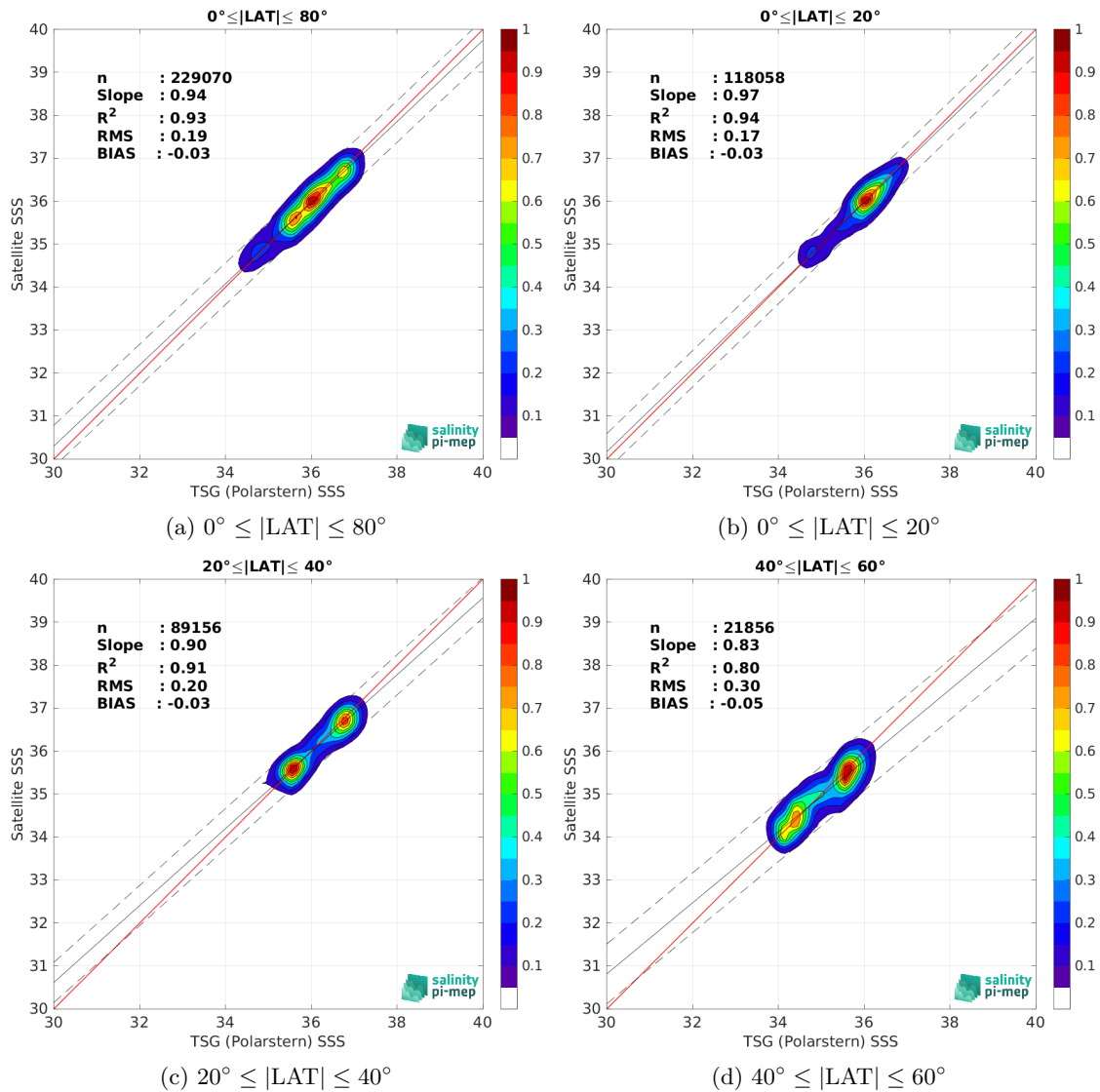
Figure 9: Contour maps of the concentration of SMOS SSS L3 v8 - 18 Days (CATDS-CEC-LOCEAN) SSS ( y -axis) versus TSG (Polarstern) SSS ( x -axis) at match-up pairs for different latitude bands. For each plot, the red line shows x=y . The black thin and dashed lines indicate a linear fit through the data cloud and the \pm 95\% confidence levels, respectively. The number match-up pairs n , the slope and R^2 coefficient of the linear fit, the root mean square (RMS) and the mean bias between satellite and in situ data are indicated for each latitude band in each plots.
