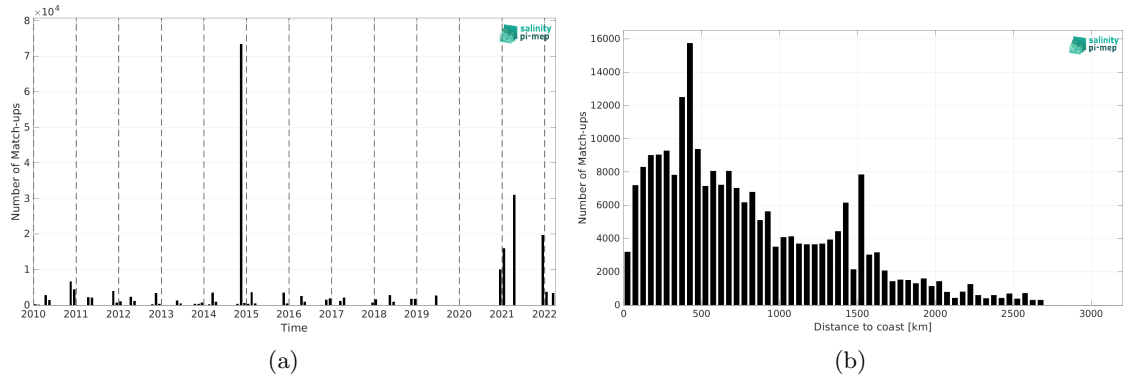
Figure 1: Number of match-ups between TSG (Polarstern) and SMOS SSS L3 v8 - 18 Days (CATDS-CEC-LOCEAN) SSS as a function of time (a) and as function of the distance to coast (b) over the Mid-Low Latitudes 45N-45S Pi-MEP region and for the full satellite product period.
