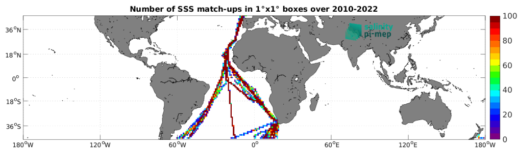
Figure 4: Number of SSS match-ups between TSG (Polarstern) SSS and the SMOS SSS L3 v8 - 18 Days (CATDS-CEC-LOCEAN) SSS product for the Mid-Low Latitudes 45N-45S Pi-MEP region over 1^\circ \times 1^\circ boxes and for the full satellite product period.
