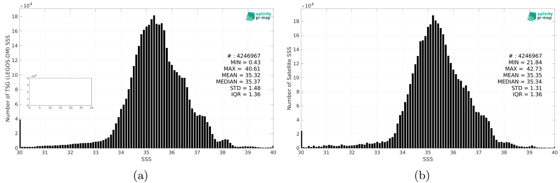
Figure 2: Histograms of SSS from TSG (LEGOS-DM) (a) and SMOS SSS L3 v8 - 18 Days (CATDS-CEC-LOCEAN) (b) considering all match-up pairs per bins of 0.1 over the Mid-Low Latitudes 45N-45S Pi-MEP region and for the full satellite product period.
