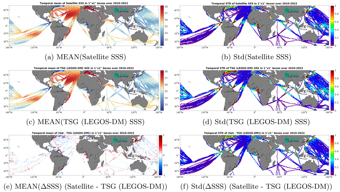
Figure 6: Temporal mean (left) and Std (right) of SSS from SMOS SSS L3 v8 - 18 Days (CATDS-CEC-LOCEAN) (top), TSG (LEGOS-DM) (middle), and of \Delta SSS (Satellite - TSG (LEGOS-DM)). Only match-up pairs are used to generate these maps.
