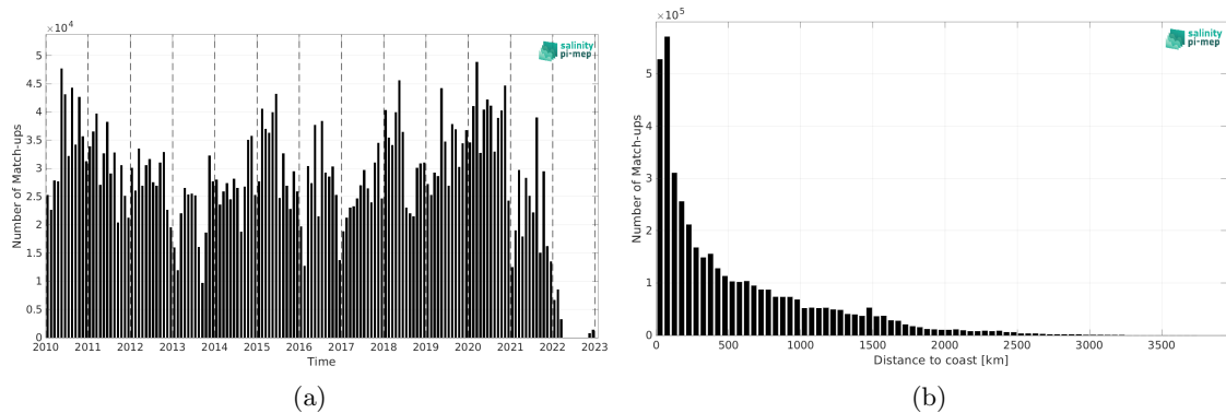
Figure 1: Number of match-ups between TSG (LEGOS-DM) and SMOS SSS L3 v8 - 18 Days (CATDS-CEC-LOCEAN) SSS as a function of time (a) and as function of the distance to coast (b) over the Mid-Low Latitudes 45N-45S Pi-MEP region and for the full satellite product period.
