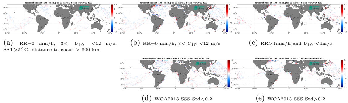
Figure 12: Temporal mean gridded over spatial boxes of size 1^\circ \times 1^\circ of \Delta SSS (SMOS SSS L3 v8 - 18 Days (CATDS-CEC-LOCEAN) - TSG (LEGOS-DM)) for 5 different subdatasets corresponding to:RR=0 mm/h, 3 < U_{10} < 12 m/s, SST >5^\circ C, distance to coast > 800 km (a), RR=0 mm/h, 3 < U_{10} < 12 m/s (b), RR >1 mm/h and U_{10} < 4 m/s (c), WOA2013 SSS Std <0.2 (d), WOA2013 SSS Std >0.2 (e).
