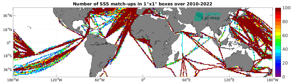
Figure 4: Number of SSS match-ups between TSG (LEGOS-DM) SSS and the SMOS SSS L3 v8 - 18 Days (CATDS-CEC-LOCEAN) SSS product for the Mid-Low Latitudes 45N-45S Pi-MEP region over 1^\circ \times 1^\circ boxes and for the full satellite product period.
